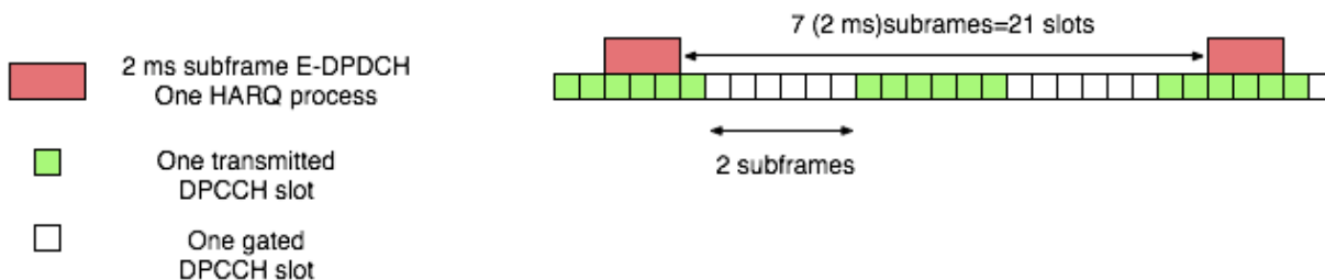
Figure 4.2.2.3.1.1-2: 50% gated DPCCH.
