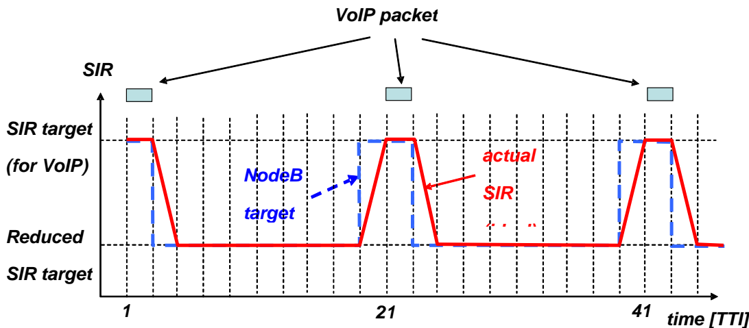
Figure 4.3.1.1.2-1 Illustration of an ideal SIR_target reduction profile for VoIP packets every 20ms (HARQ retransmission and inactive phases with SIDs are not shown in this example)
