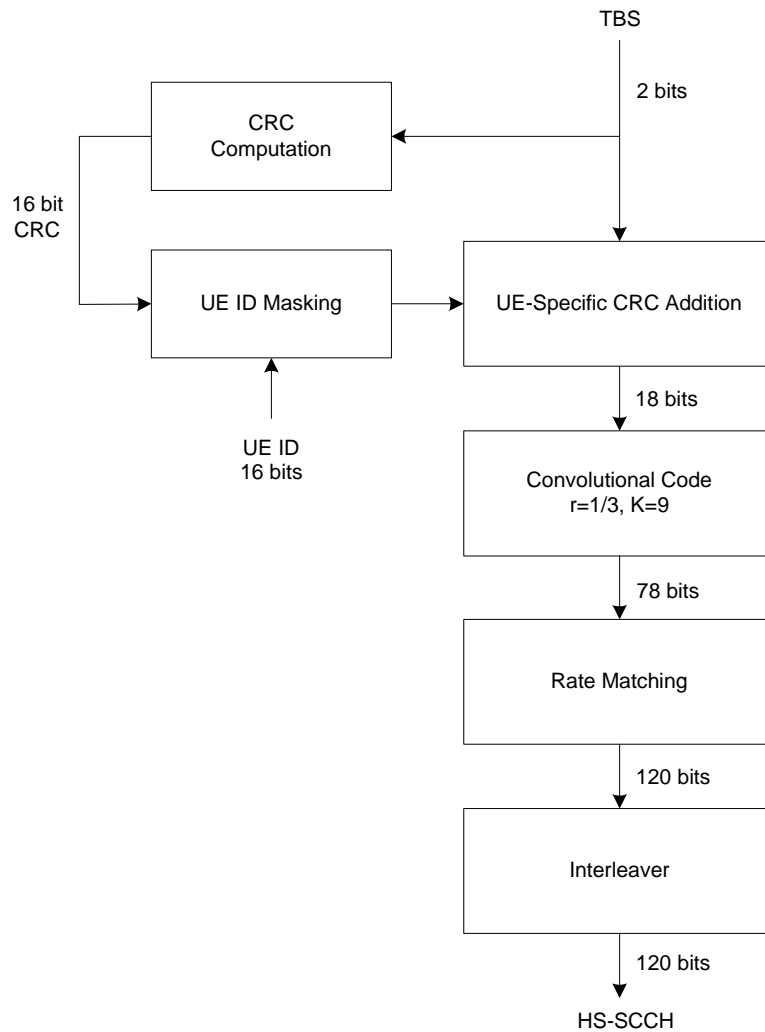
Figure 4.6.1.3-1: Coding for restricted HS-SCCH
