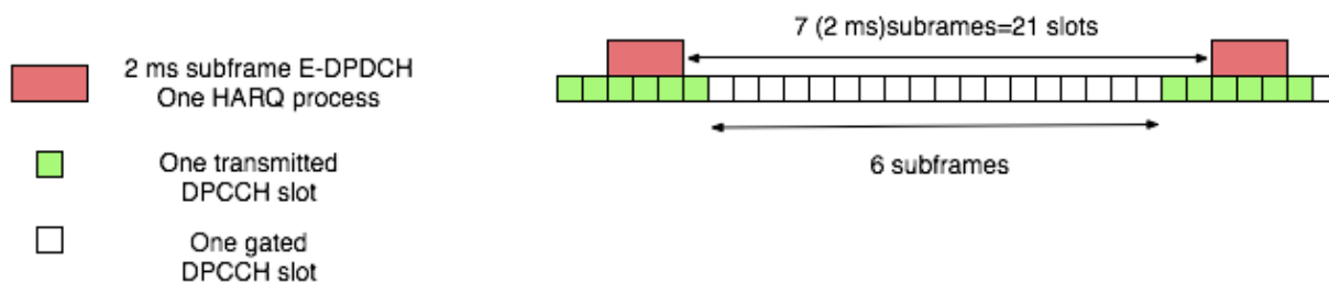
Figure 4.2.2.3.1.1-3: 75% gated DPCCH.
