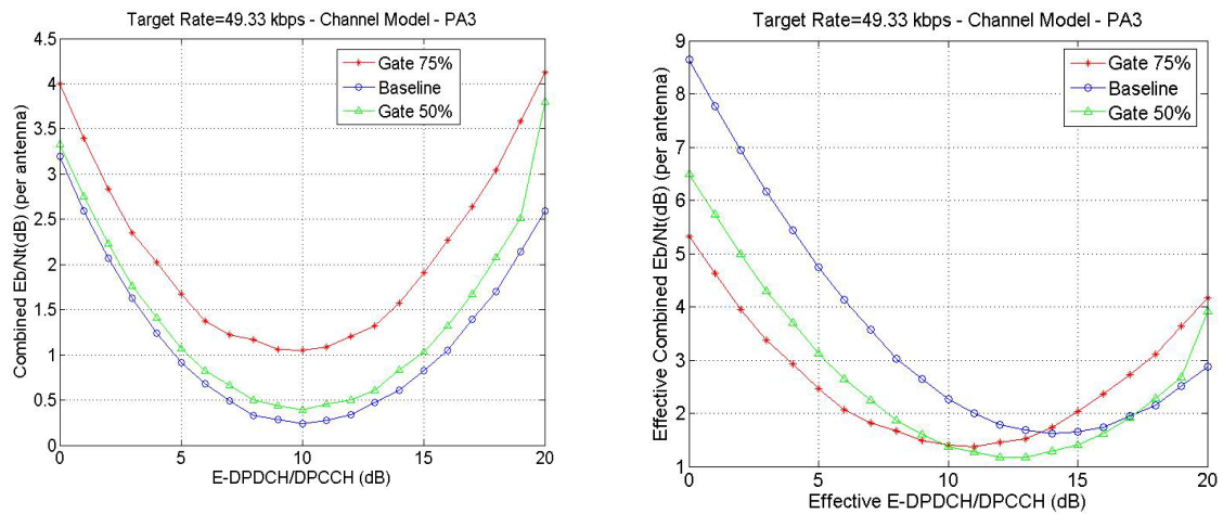
Figure 4.2.2.3.1.2.1-4: PA3 channel, different gating patterns, Combined Eb/Nt per antenna without TTL and FTL, target rate 49.3 kbps.
