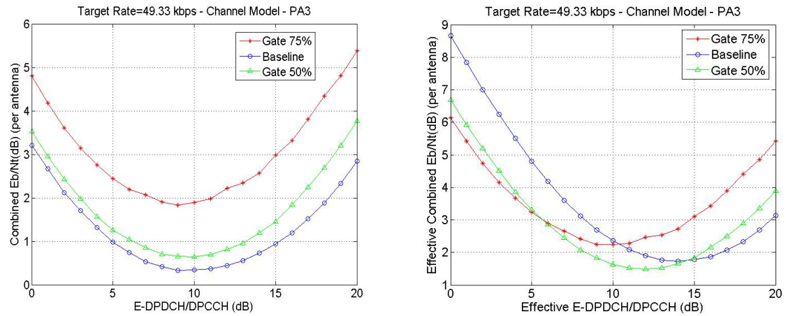
Figure 4.2.2.3.1.2.1-3: PA3 channel, different gating patterns, Combined Eb/Nt per antenna with TTL and FTL, target rate 49.3 kbps.
