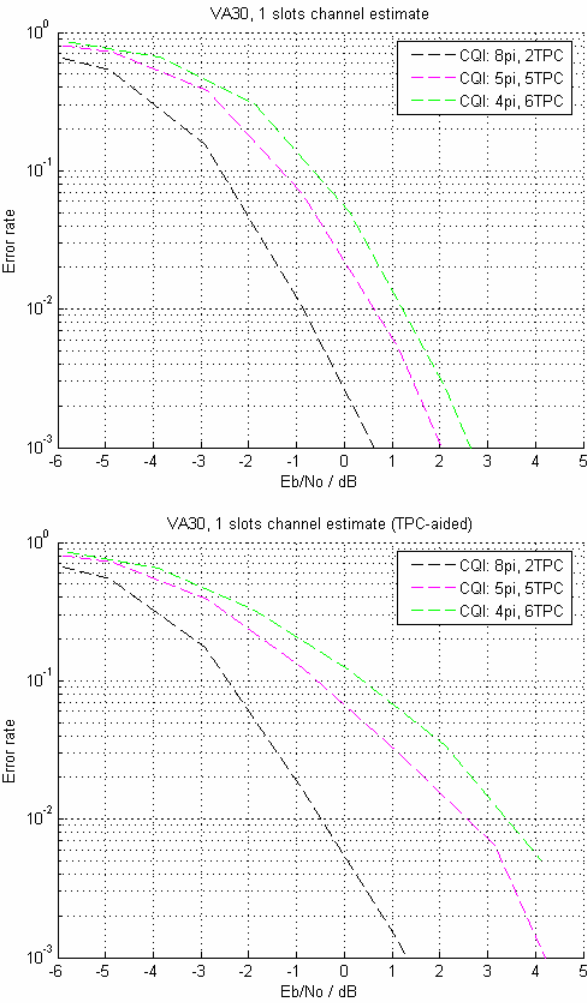
Figure 4.1.2.1-5: CQI performance in VA30, 1 slot channel estimation, with and without TPC-assistance
