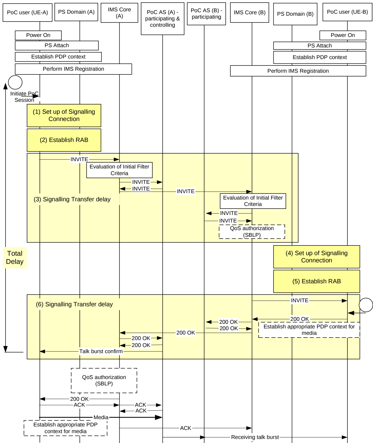
Figure B.1: Delay component for the case of on demand session with manual answer
