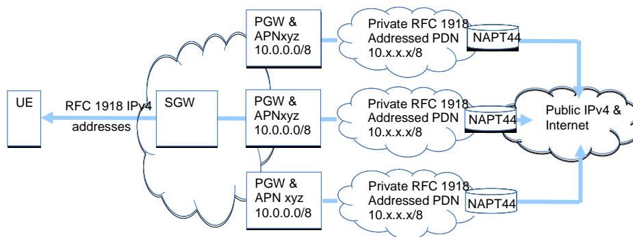
Figure 7.1.4: Overlapping RFC 1918 address spaces for the same APN and distributed NAPT44
