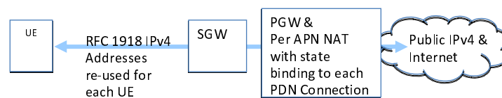
Figure B.4.1: Per-Interface NAT. Overlapping RFC 1918 address space for the same APN with per-interface (PDN Connection) basis NAT binding
