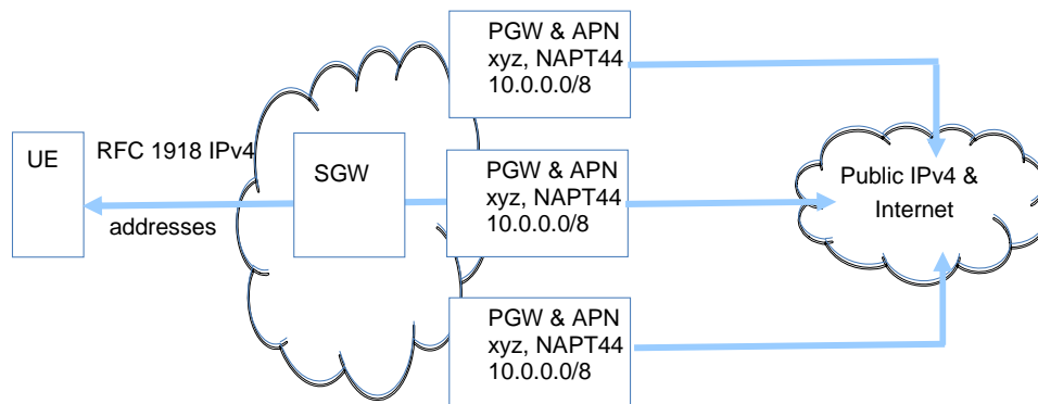
Figure 7.1.3: Overlapping RFC 1918 address spaces for the same APN and NAPT44 collocated with a PDN-GW
