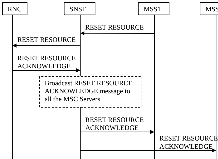
Figure 5.6.3.1.3.2.1.1: MSC Server initiated Reset Resource Procedure
