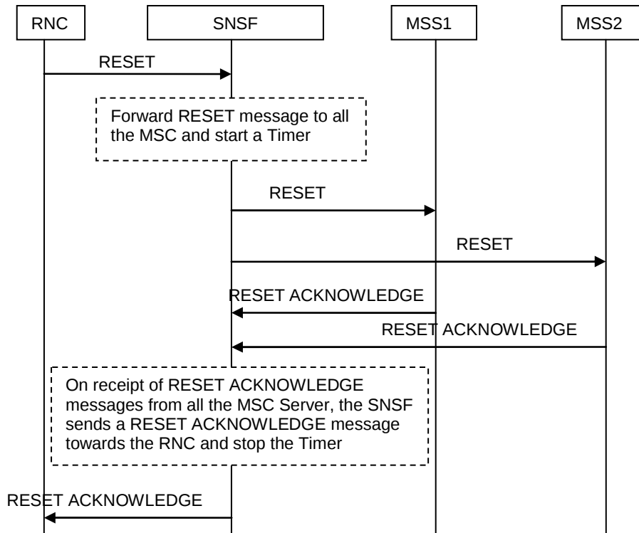
Figure 5.6.3.1.1.1: UTRAN initiated RESET procedure
