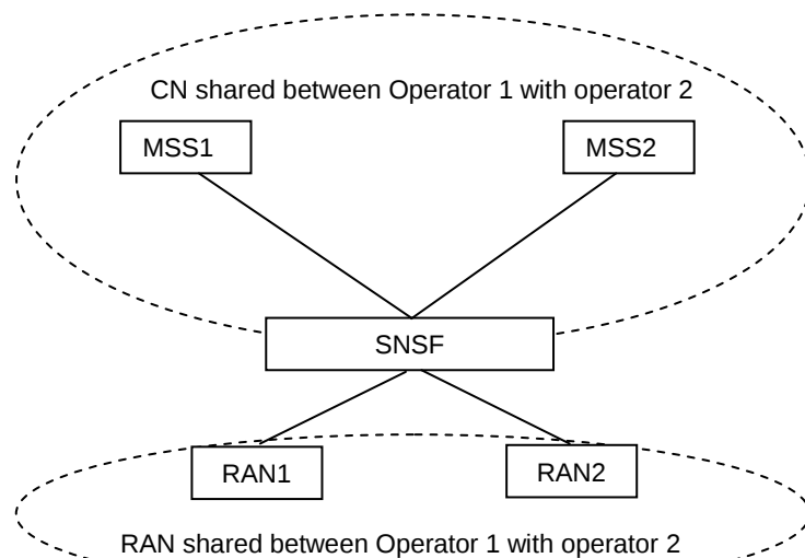
Figure 6.1.2-1b: Both GWCN and MSC Pool are configured
