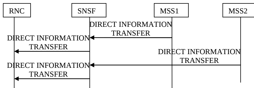
Figure 5.6.3.1.6.2.1: Direct Information Transfer initiated from the CN
