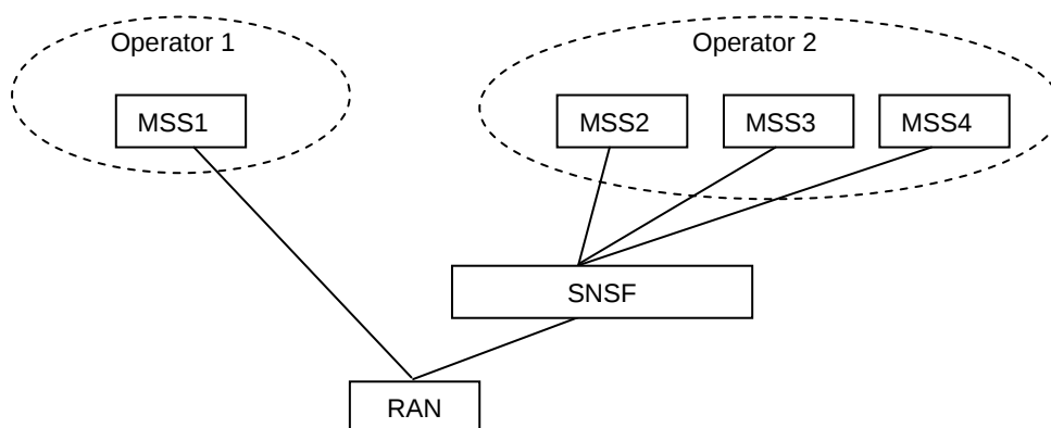
Figure 6.1.1.3.1: Network configurations for MOCN with MSC Pool
