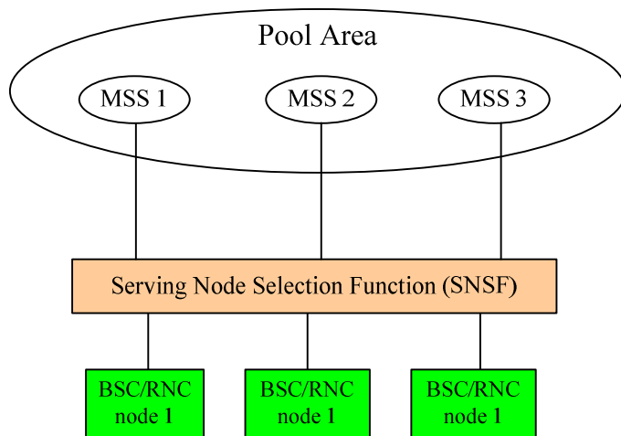
Figure 4.2.2.1: Deploying SNSF outside of the BSC/RNC nodes
