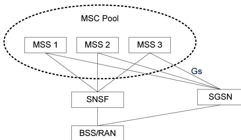
Deploying SNSF above the BSS/RAN nodes
