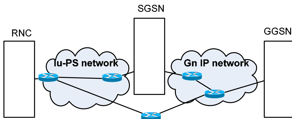
Figure 6-2: Connectivity with Iu-PS
