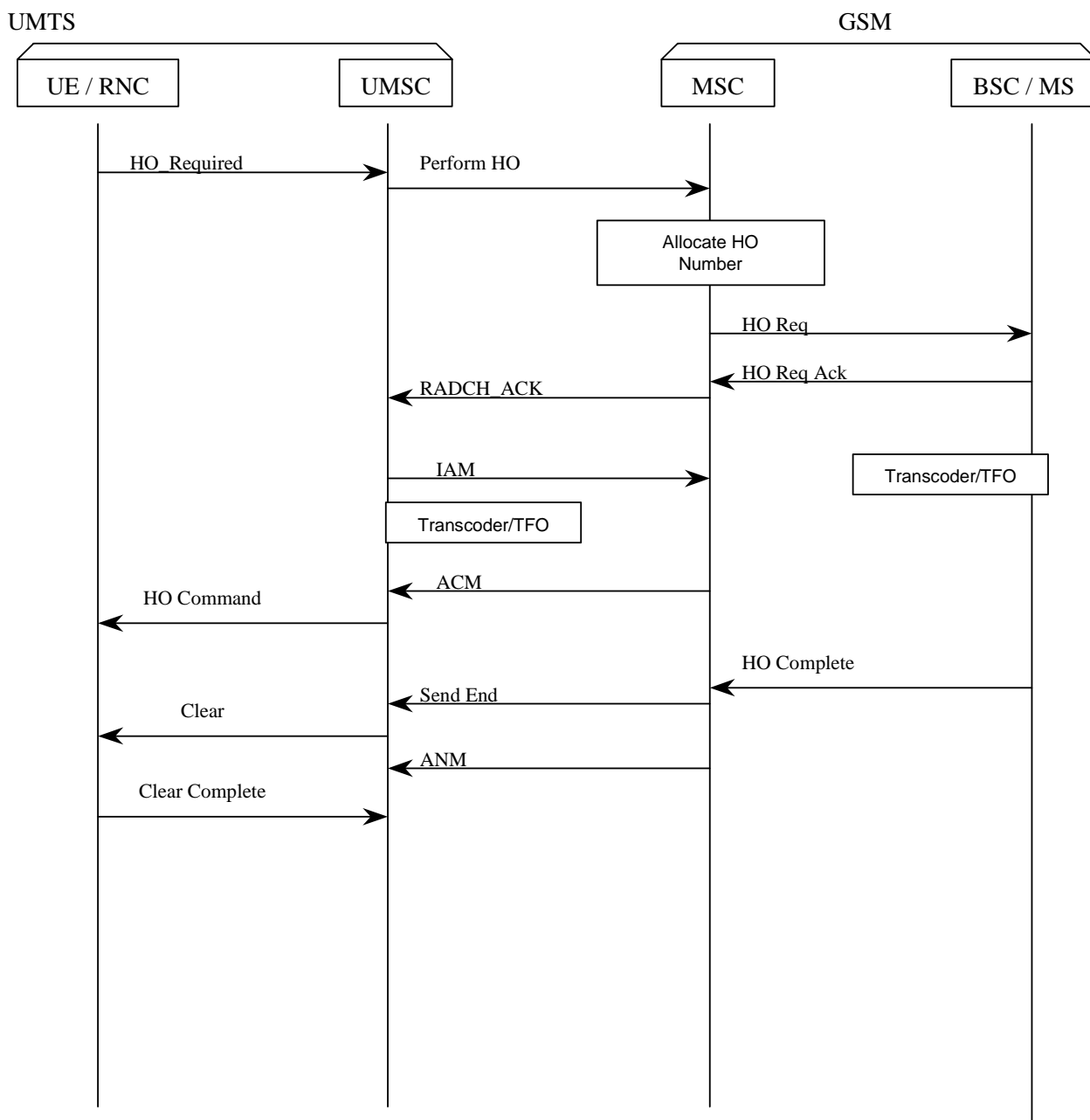
Figure 7.5.6: UMTS → GSM Handover after transcoder free establishment
