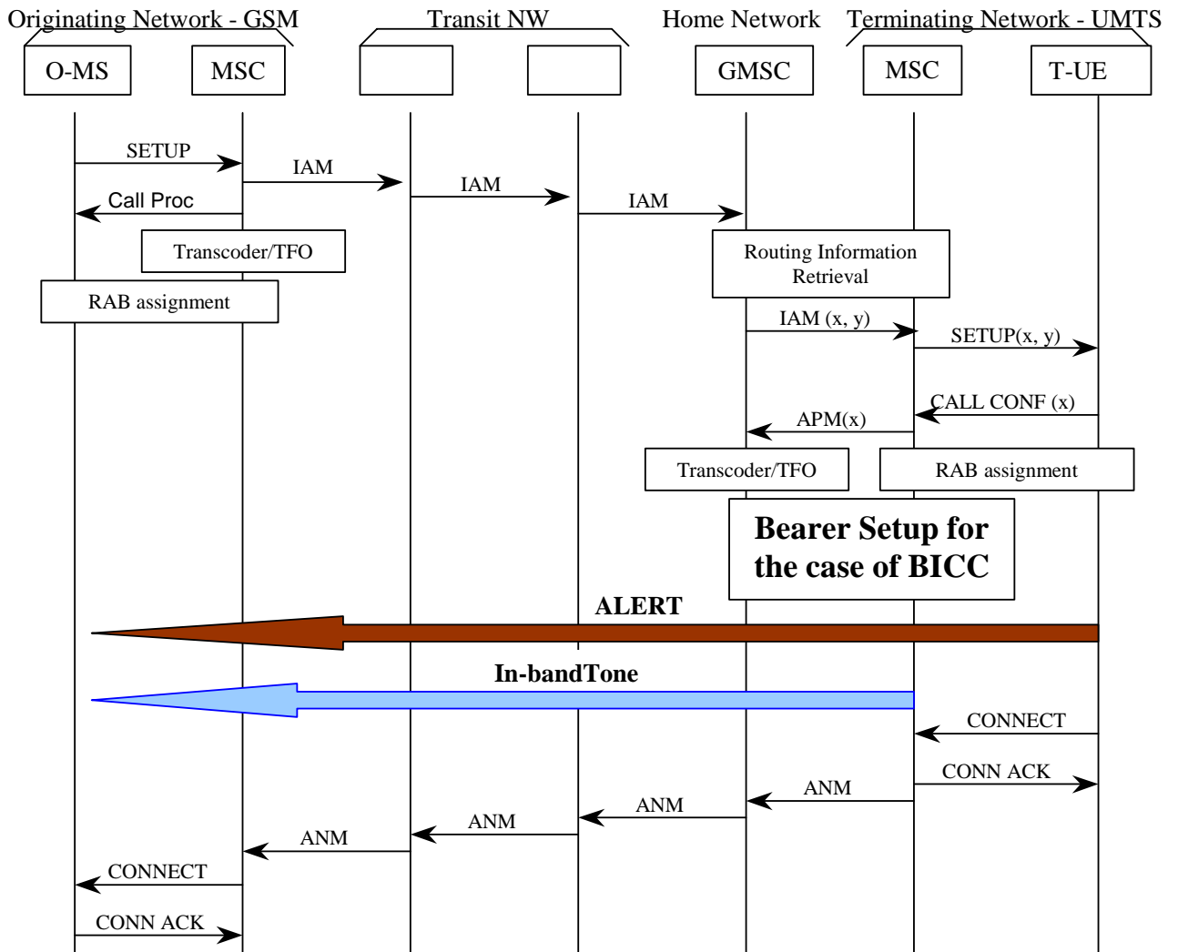
Figure 7.5.5: GSM MS →UMTS UE call, APM-user not supported in the GSM network
