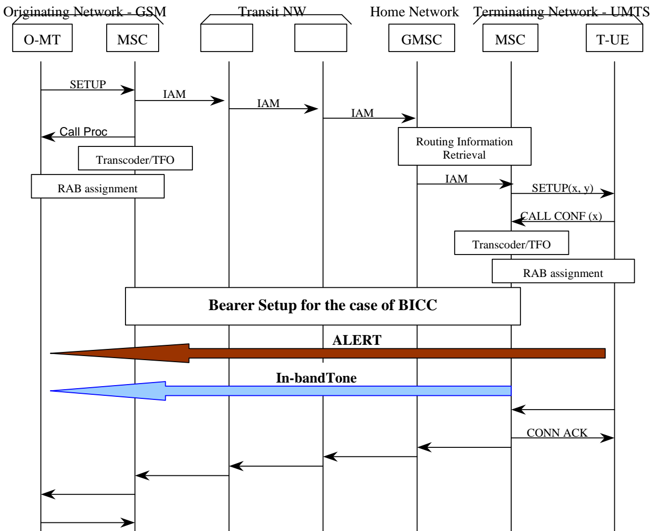
Figure 7.5.4: GSM MS →UMTS UE call, APM-user not supported in the GSM network
