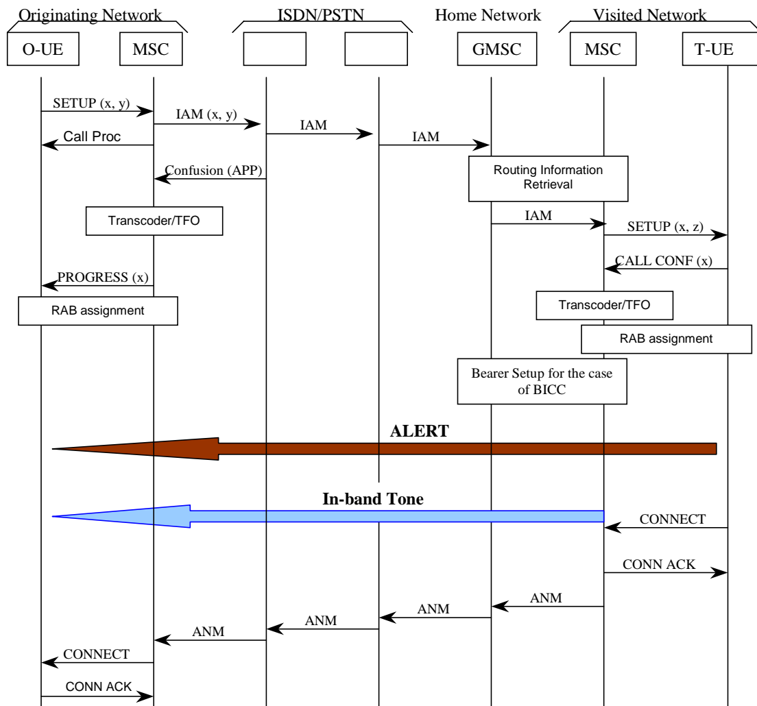
Figure 7.5.2. UMS UE – UMS UE call with transit network (PSTN/ISDN) not supporting
