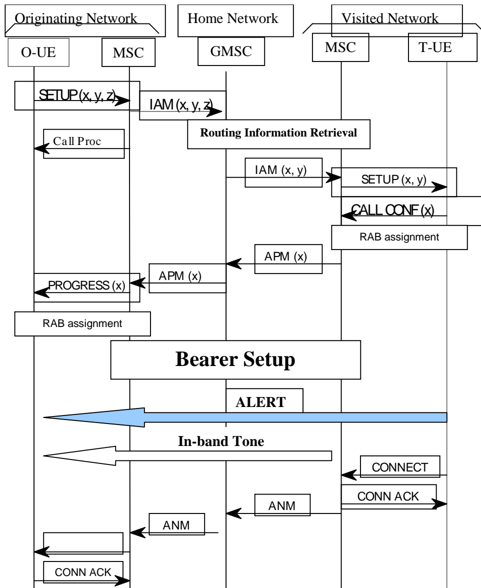
Figure 7.5.1 UMTS UE - UMTS UE call, BICC from O-MSC to T-MSC
