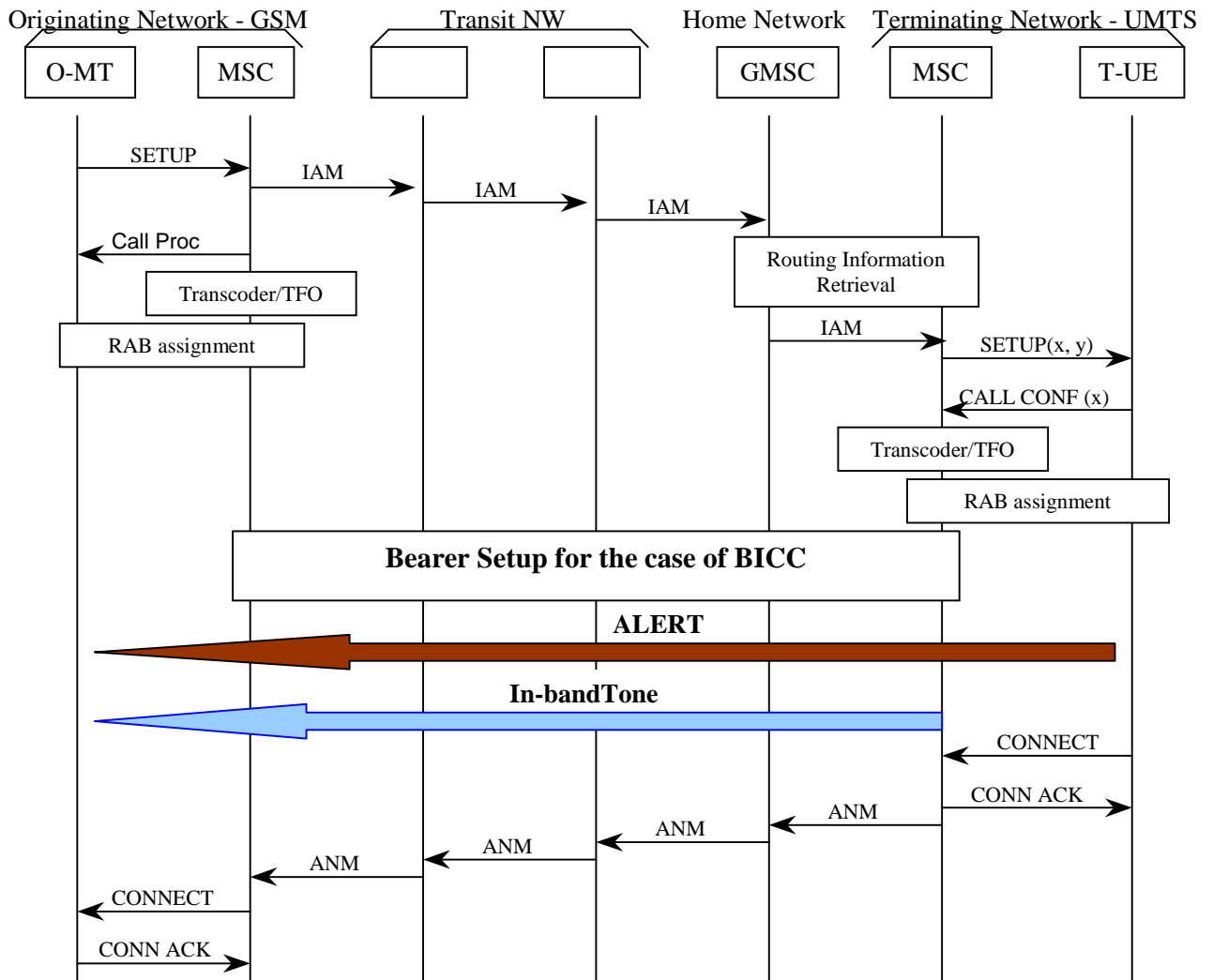
Figure 7.5.4. GSM MS → UMTS UE call, APM-user not supported in the GSM
