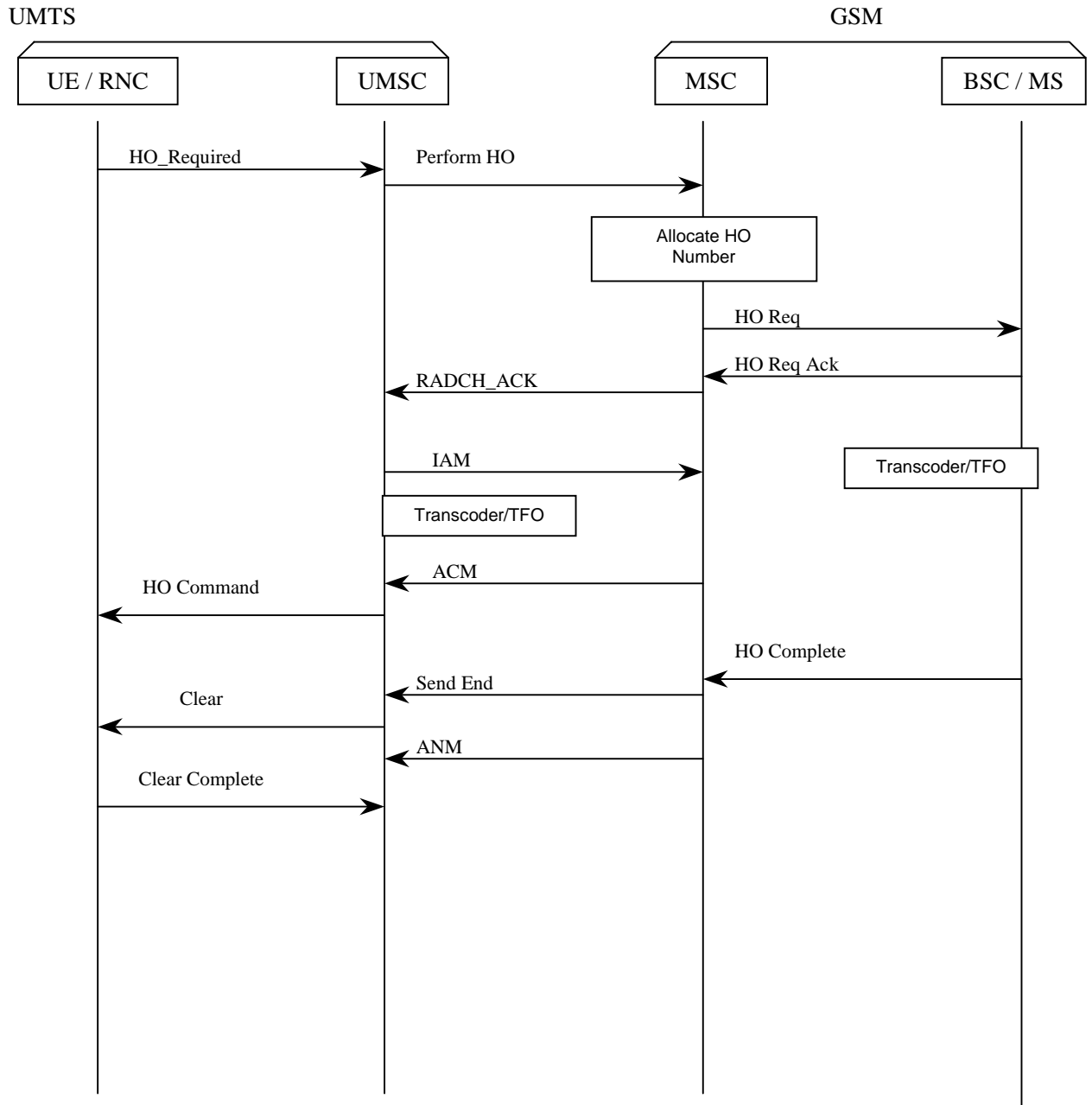
Figure 7.5.6. UMTS → GSM Handover after transcoder free establishment
