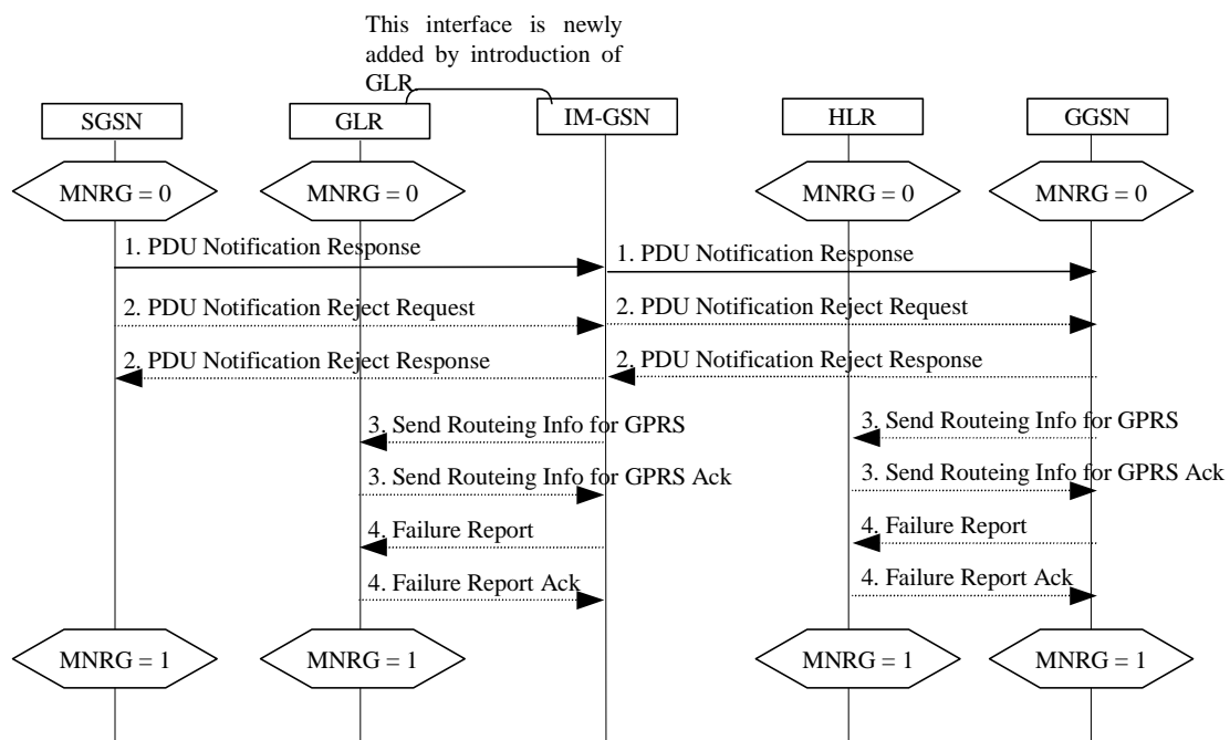
Figure 21: Protection Procedure
