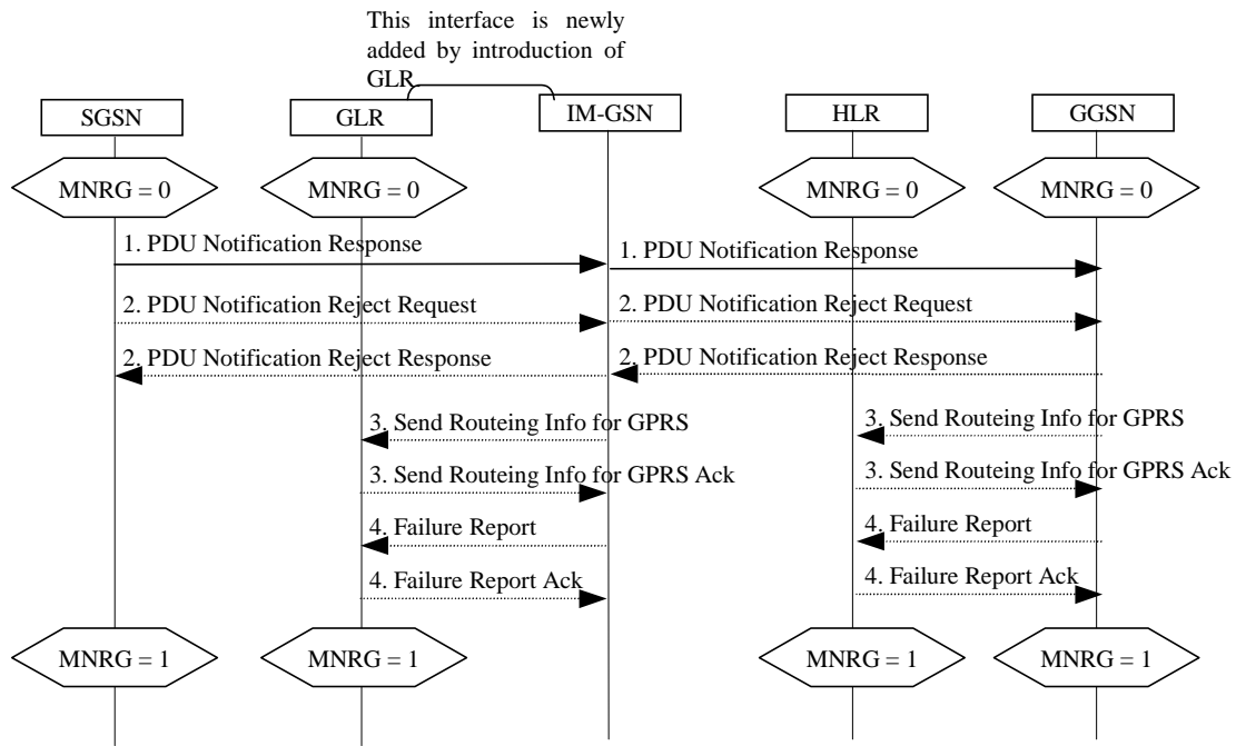
Figure 21: Protection Procedure
