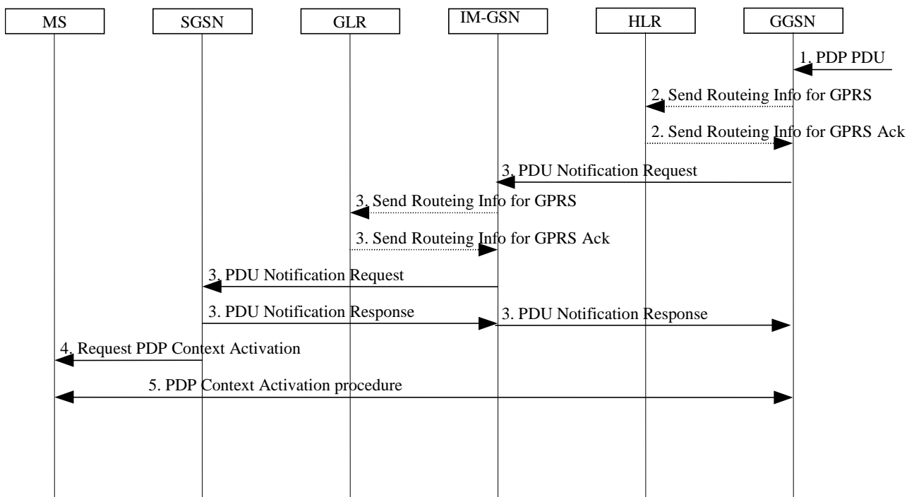
Figure 20: Successful Network-Requested PDP Context Activation Procedure
