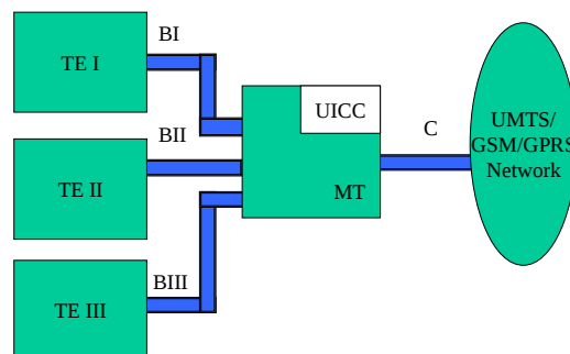
Figure 2: Multiple applications and/or users with one subscriber identity.
