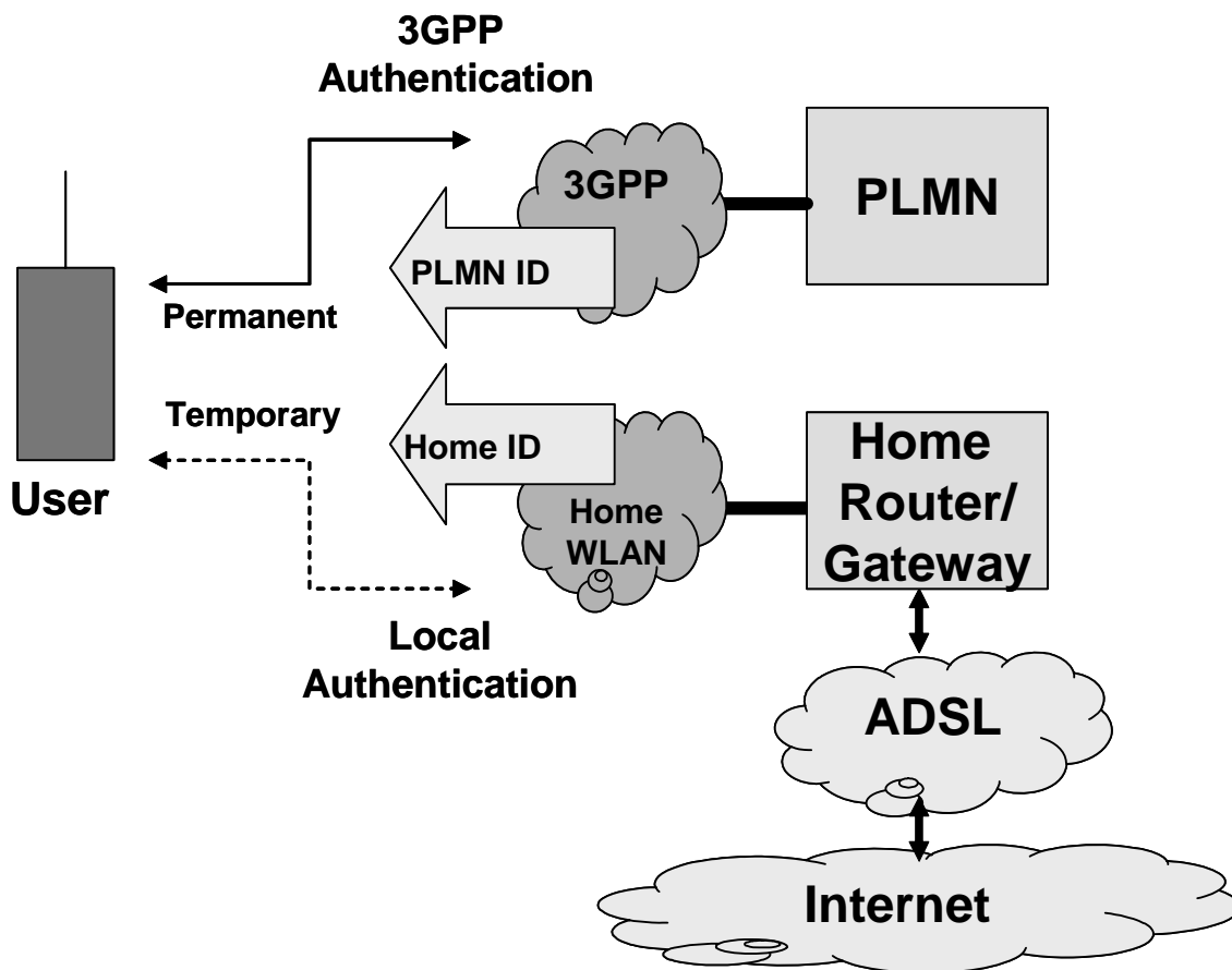
Figure 5.3: Use Case 3
