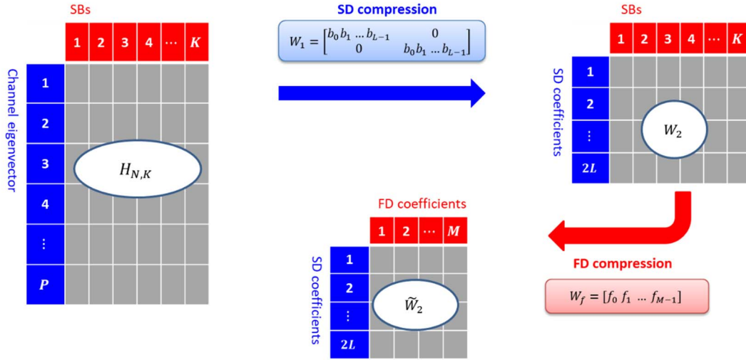
Figure 3 Frequency compression of H_{N,K} .
