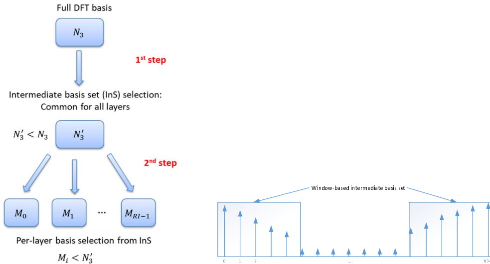
Figure 4 Two-step FD basis selection
