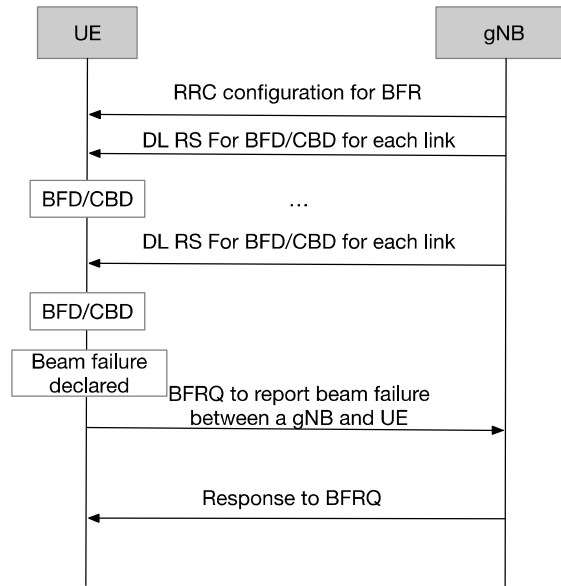
Figure 7 SCell BFR procedure
