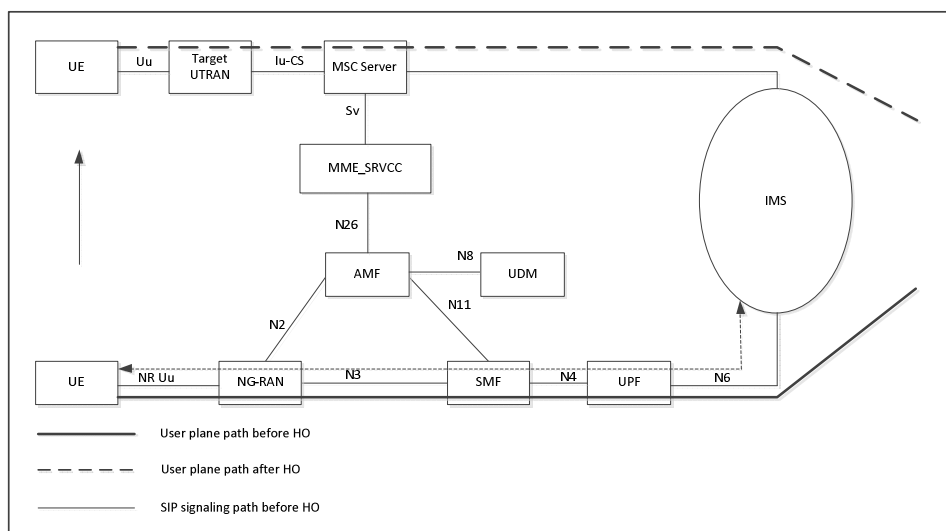
Figure 1: 5G-SRVCC architecture
