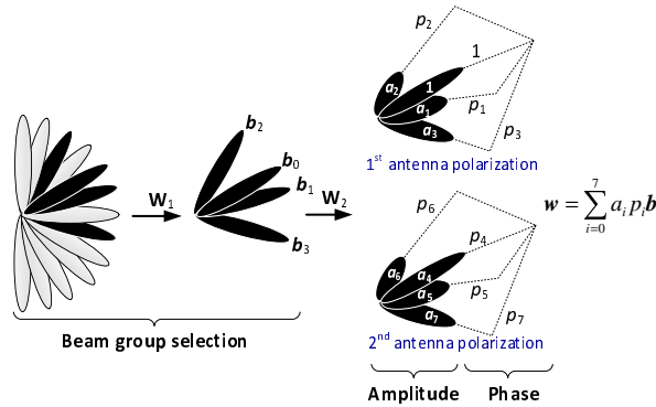
Figure 2 Linear combination based Rel. 15 Type II CSI feedback.
