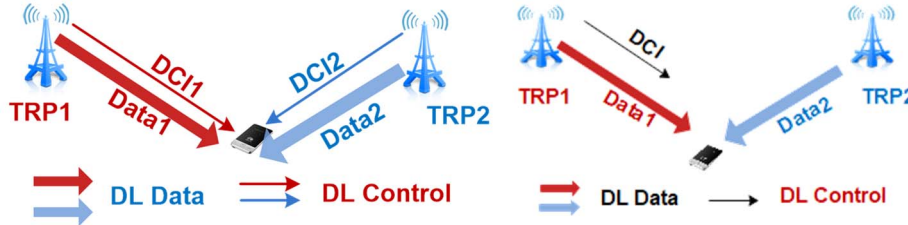
Figure 5 Two-TRP (DL) transmission/reception
