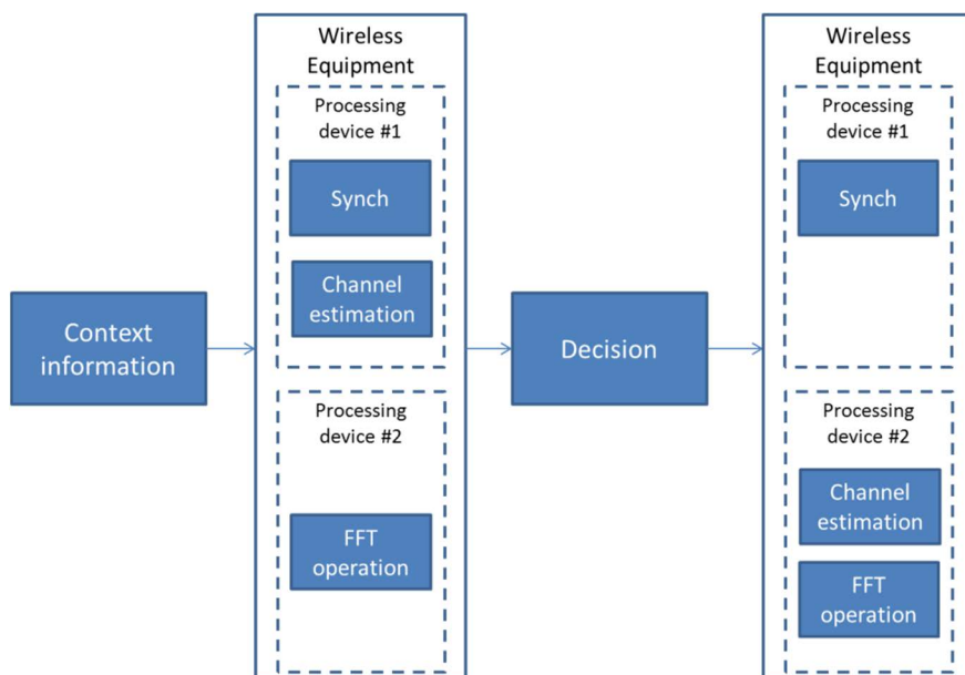
Figure 6: Scenario Illustration "Processing device selection for execution of protocols in Wireless Equipment depending on the context" - a wireless equipment changes the processing device where the channel estimation function is executed based on a decision taken according to the available context
