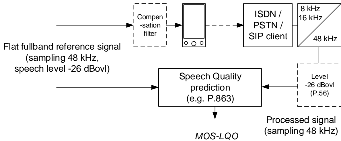
Figure 4: Test setup mobile to landline
