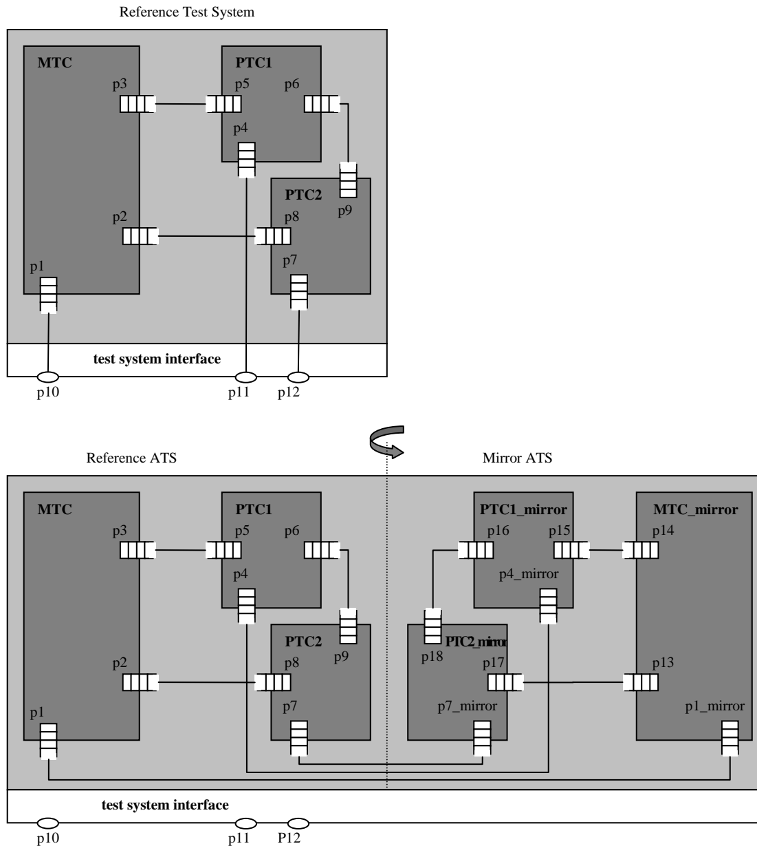
Figure 3: Illustration of multiple component reference test system (a) and derived combined test system (b), including the mirror test multiple component architecture
