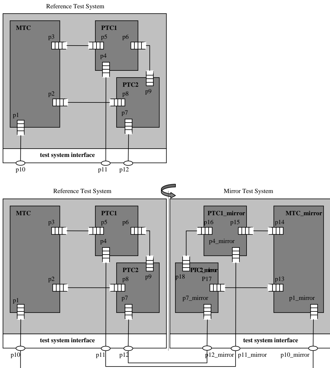
Figure 5: An example reference test system (a) and the resulting architecture according to the Inter TTCN-3 Executable approach (b)
