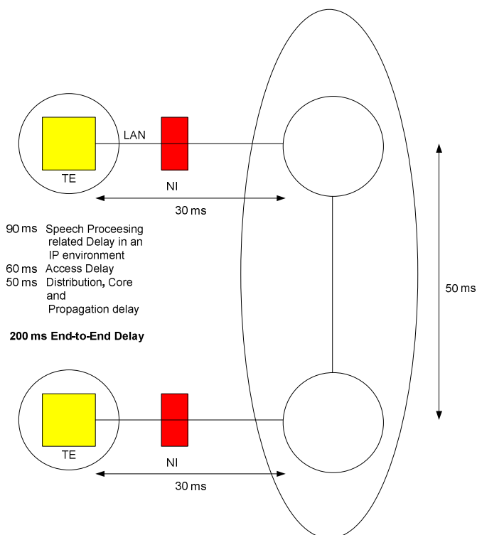
Figure 5: Delay Objectives for HIGH (G.109) voice communication quality (R > 80)
