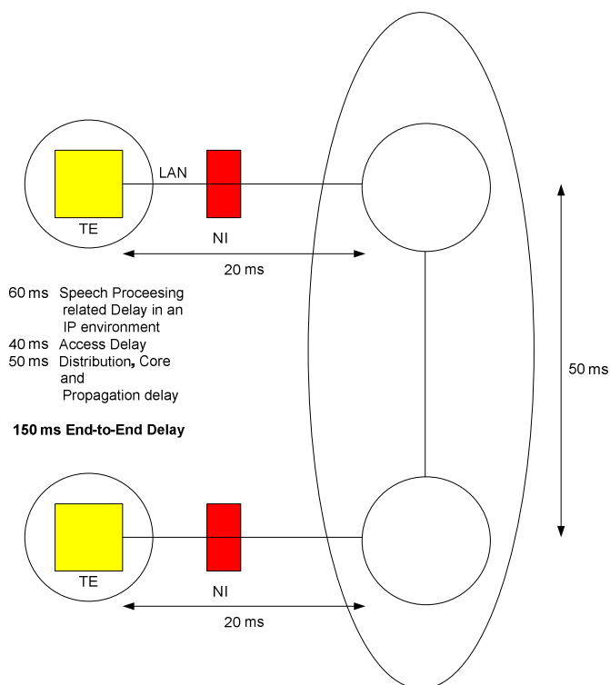
Figure 4: Delay Objectives for BEST (G.109) voice communication quality (R > 90)
