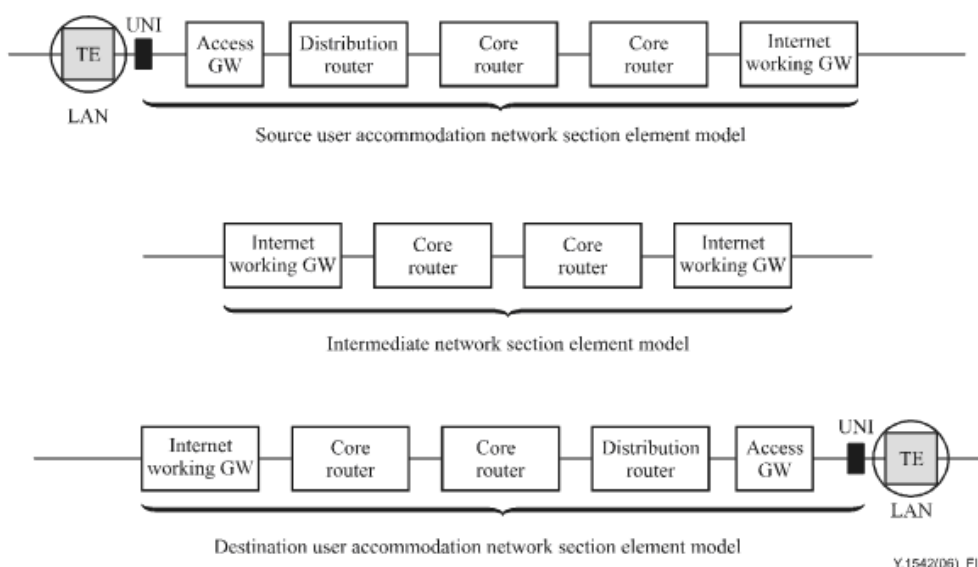
Figure 2: Division of the connection
