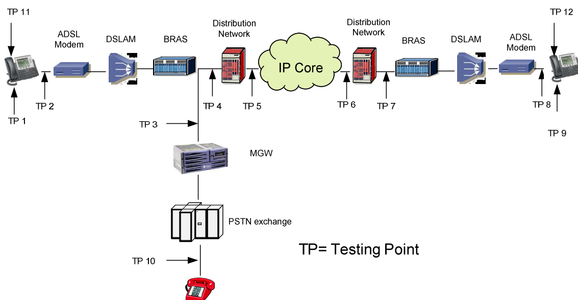
Figure 3: Example reference points for delay definition and verification in the field
