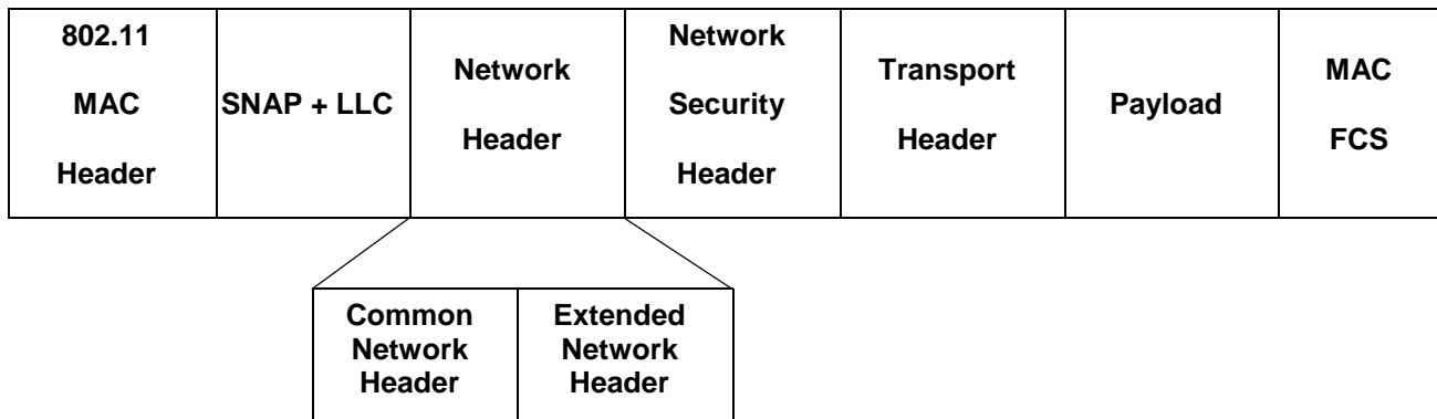
Figure A.1: Structure of the C2C-CC Network Header
