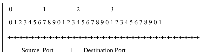
Figure A.3: ASCII Representation of the STP Header
