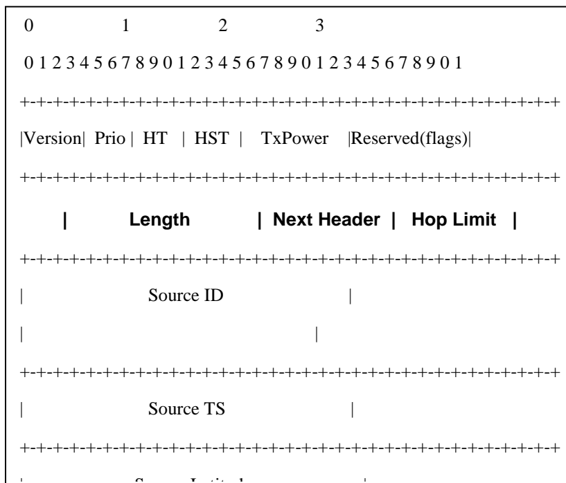
Figure A.2: ASCII Representation of the C2C-CC Demonstrator Common Network Header
