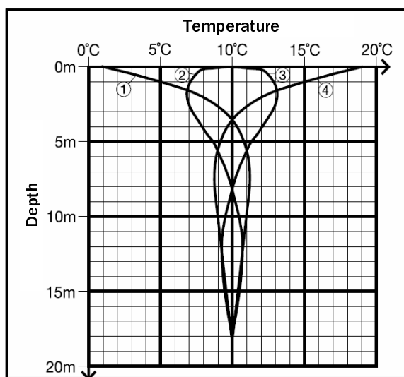
Figure 31: Temperature within the earth vs. limited depth
