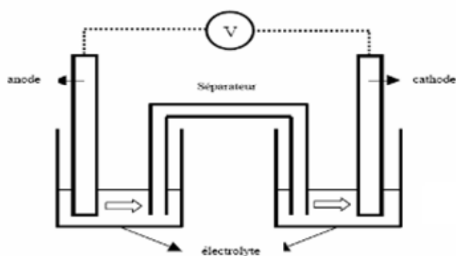
Figure 11: scheme of a Ni-Cd cell with electrochemical reactions
