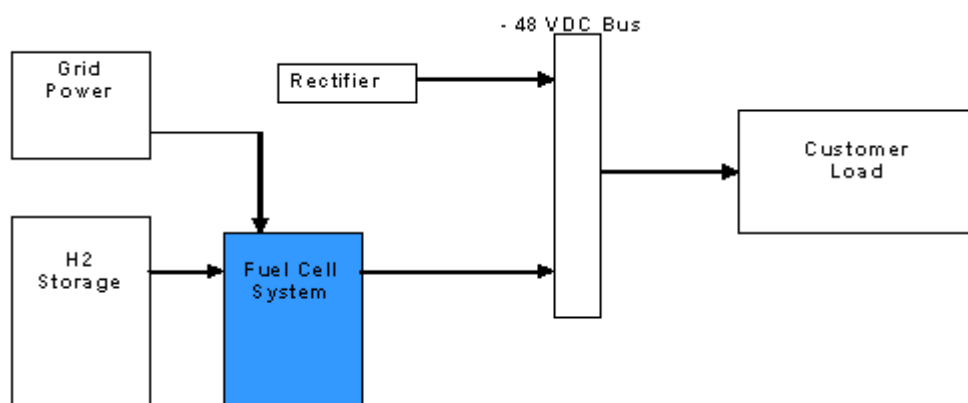
Figure 15: Back-up power application with H 2 tank storage or liquid fuel reformer (grid-connected)
