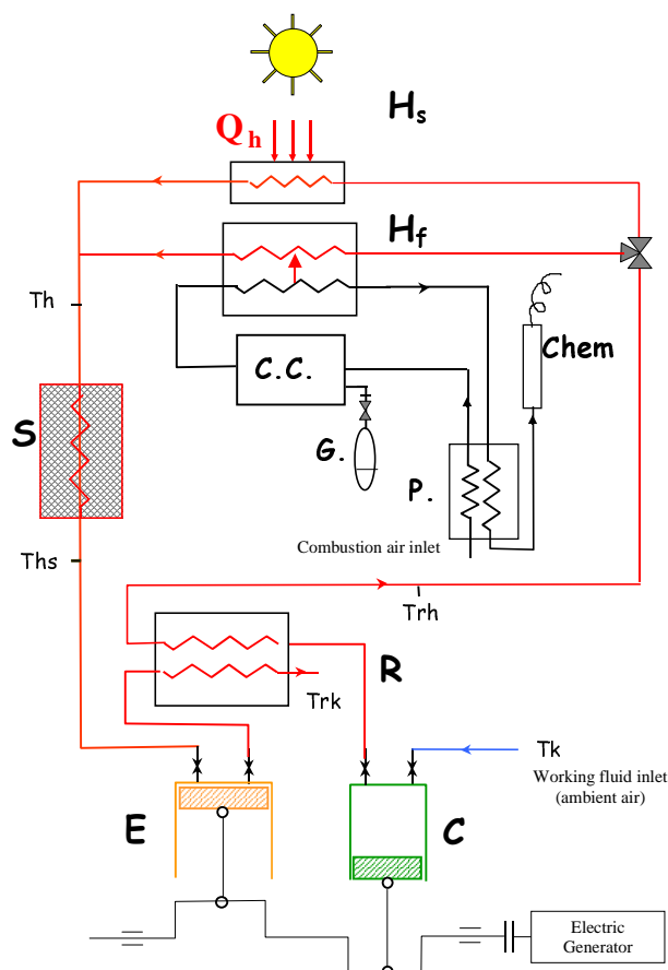
Figure 5: Hybrid system with storage
