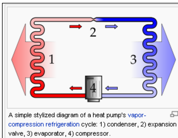
Figure 33: Heat-pump scheme
