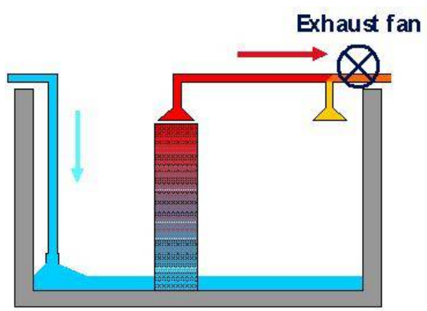
Figure 37: Scheme of total fresh air cooling solution with hot spot exhaust
