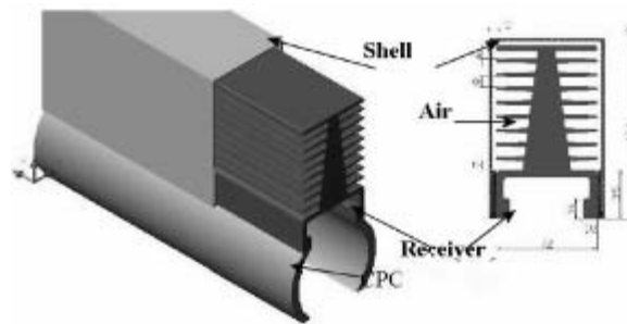
Figure 3: Concentrator second stage (CPC) and « heater »
