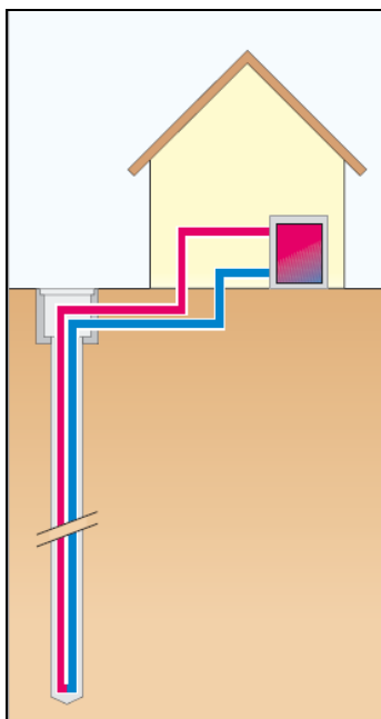
Figure 35: Geothermal plants that use vertical collectors
