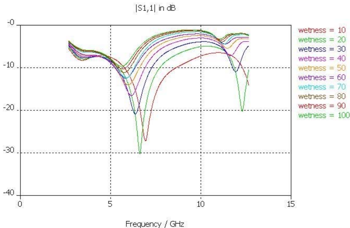
Figure B.4: Match is very sensitive to wetness in cloth. With increasing wetness, more energy is rejected from the antenna and will not be radiated!
