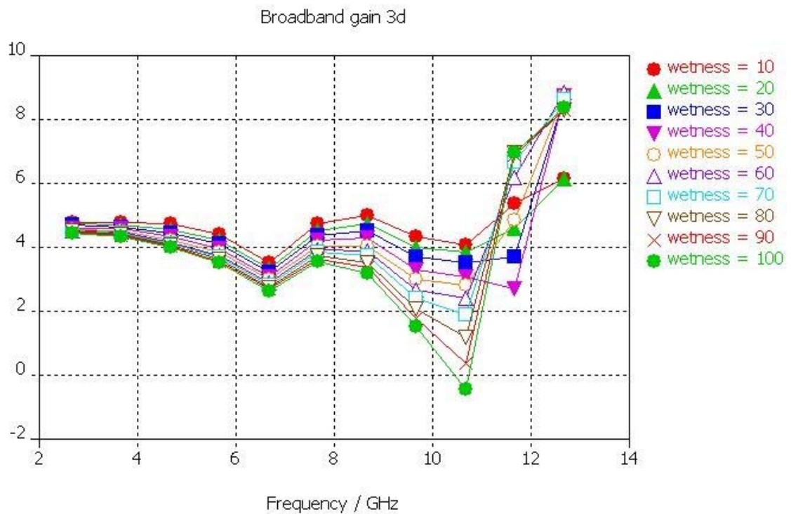
Figure B.6: Results for the gain loss (NOT INCLUDING losses concerning antenna match!)
