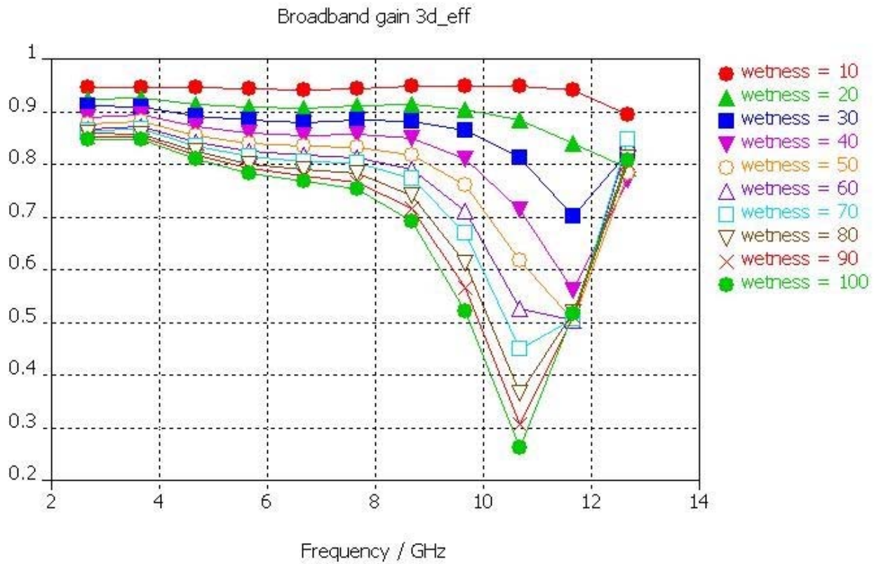
Figure B.5: Efficiency is noticeably reduced by increasing wetness
