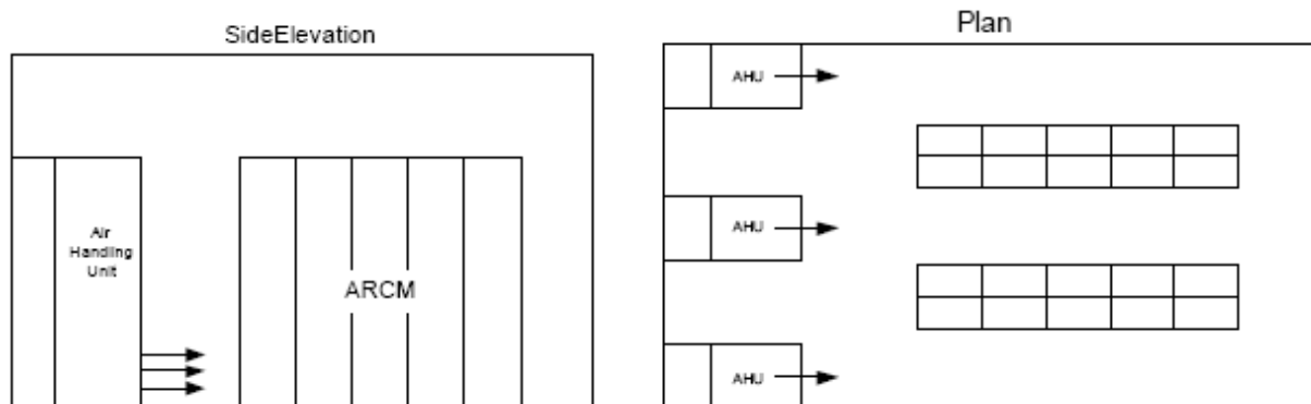
Figure 6.3.2.4b: Option B Free Blow along the aisles
