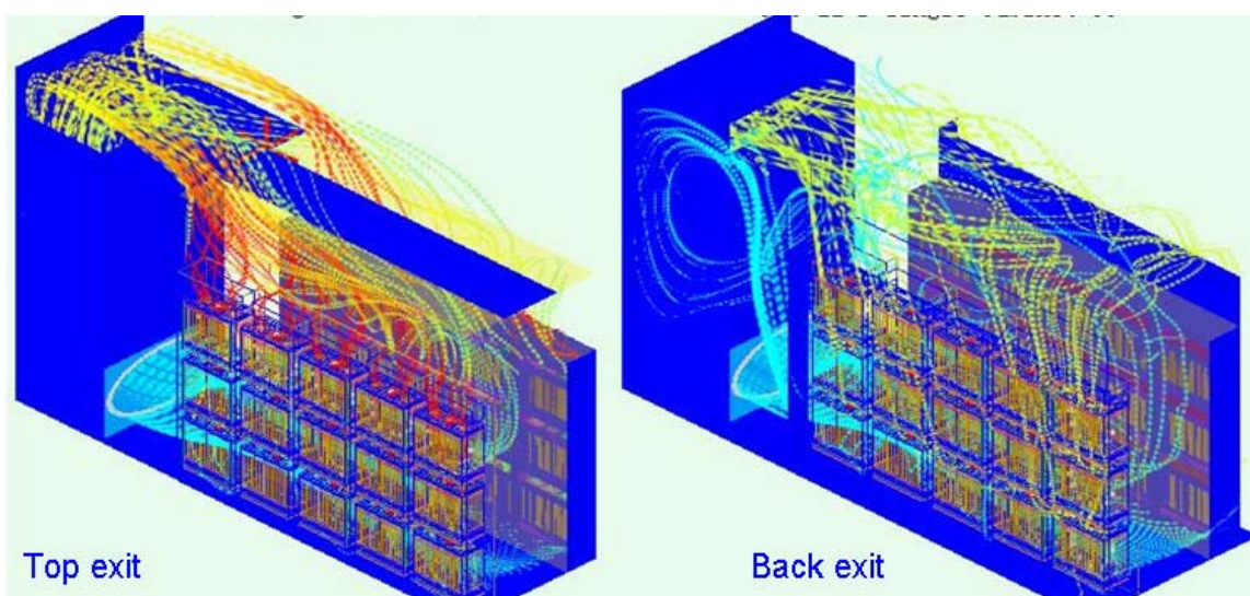
Figure B.3.3.4b: ARCM arrangement in CO
