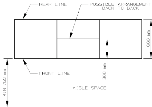
Figure B.3: EN 300 119, 300 mm arrangement
