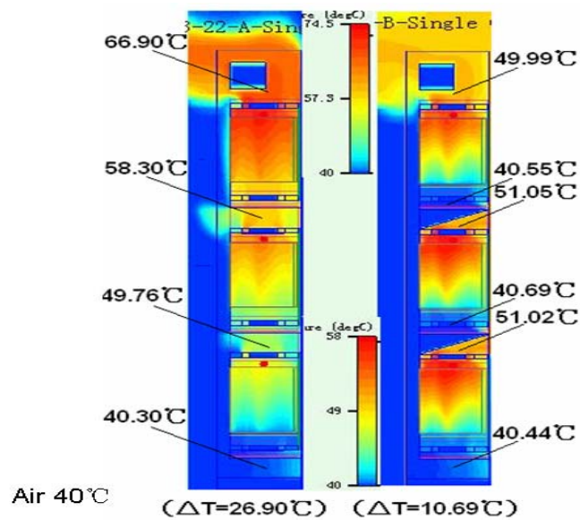
Figure B.3.3.2.a: Temperature profile of two different arrangement
