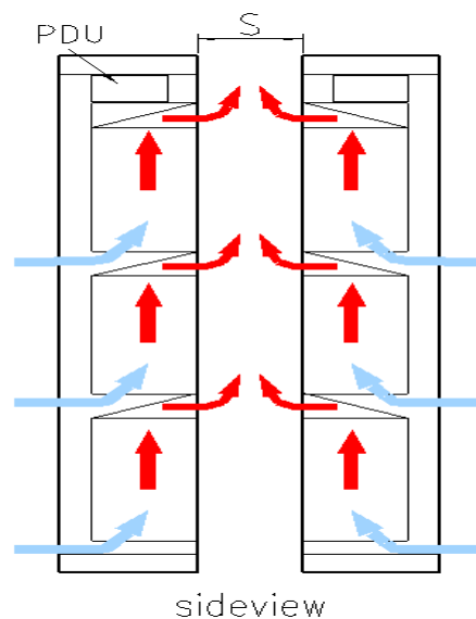
Figure B.3.3: ETSI 300 arranged with distance in CO
