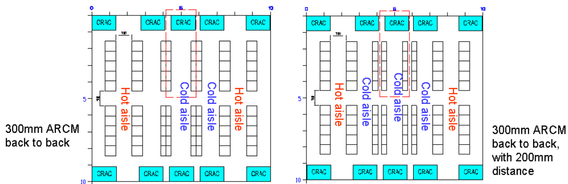
Figure B.3.3.3: Different 300 mm ARCM arrangement in CO
