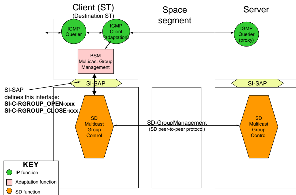
Figure 6.5.1.1: SI-SAP group receiver enable functions
