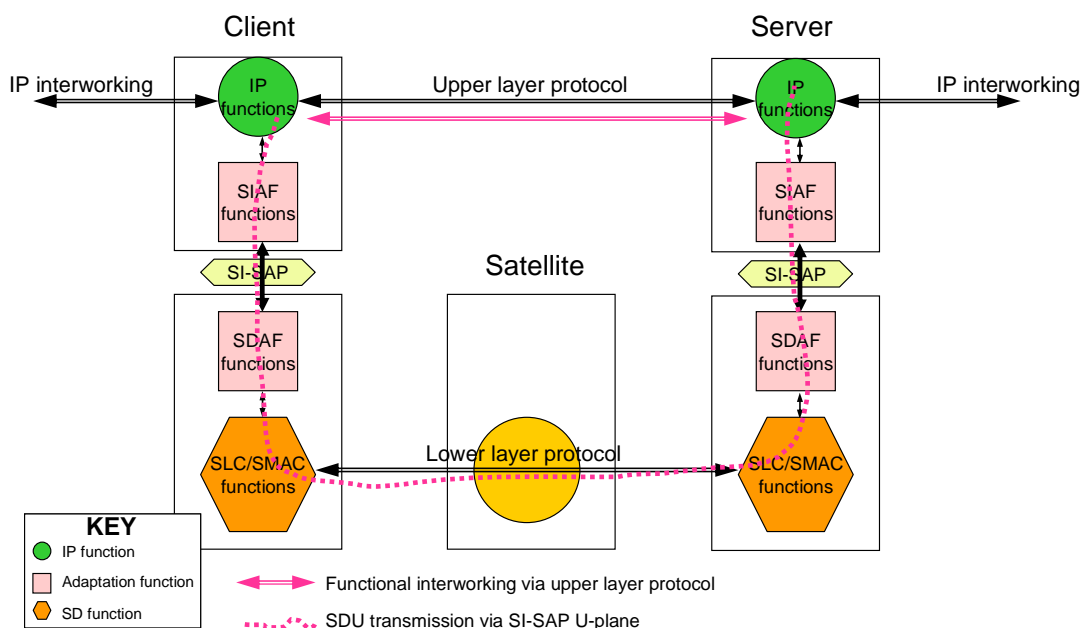
Figure 4.4.2: Interworking using upper layer protocols
