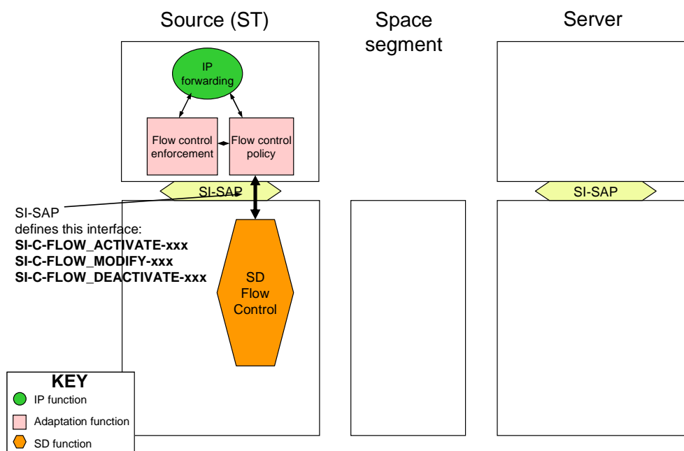
Figure 6.7.1.1: SI-SAP flow control functions
