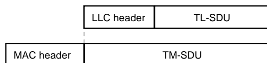
Figure 7.6: Building of data link layer PDU (with no fragmentation)
