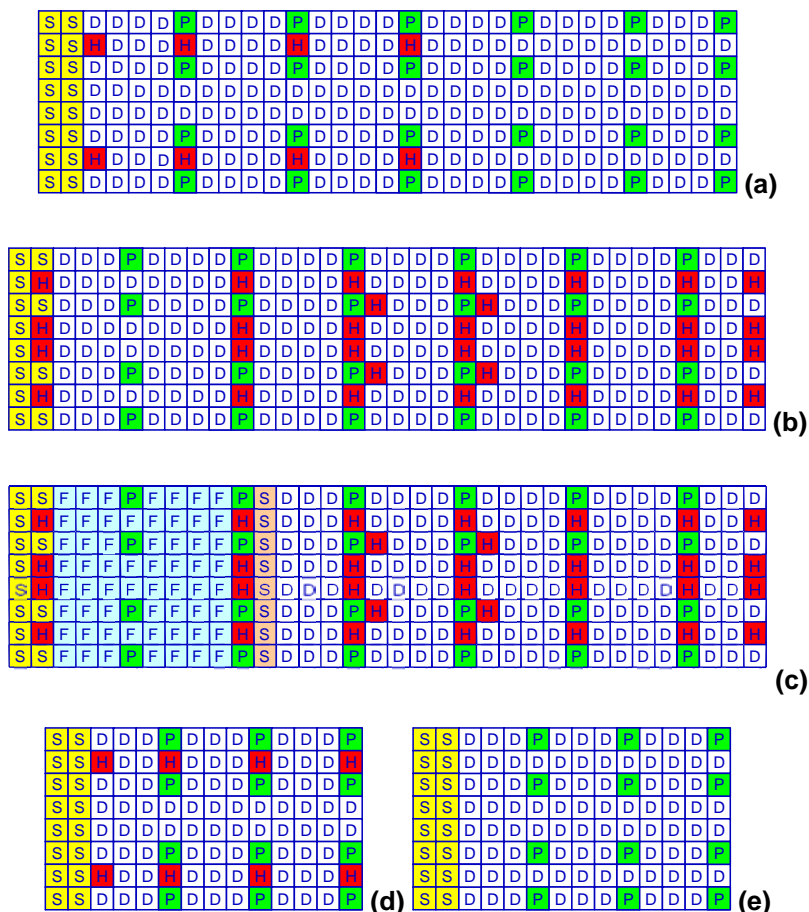
Figure 6.5: Structure of NUB (a), NDB (b), FCB (c), CB (d) and RAB (e), for a 25 kHz (8 sub-carrier) QAM channel
