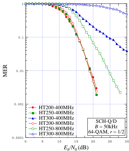
Figure 8.4: MER vs. E_b/N_0 for B = 50 kHz, SCH-Q/D, 64-QAM r = 1/2 , various HT channels
