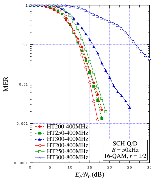
Figure 8.3: MER vs. E_b/N_0 for B = 50 kHz, SCH-Q/D, 16-QAM r = 1/2 , various HT channels
