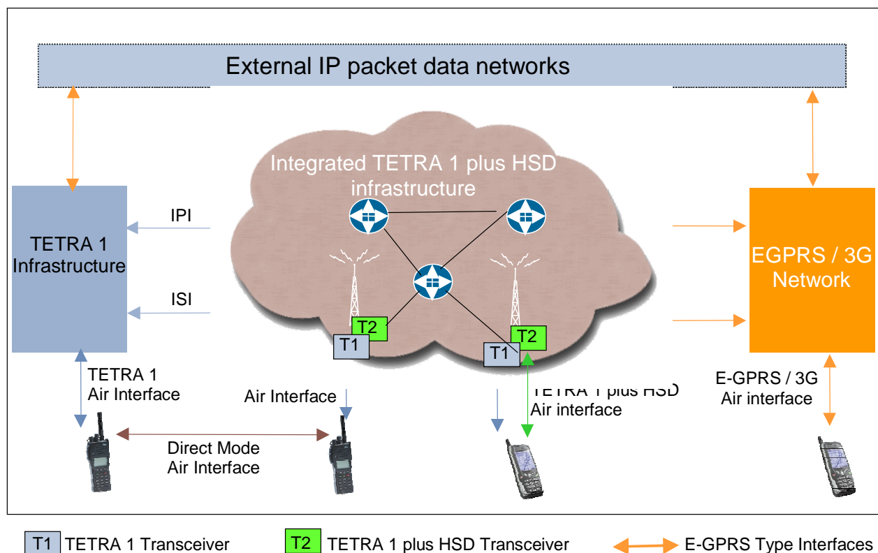
Figure 5.2: Architecture of a TETRA 2 network using Conventional Access
