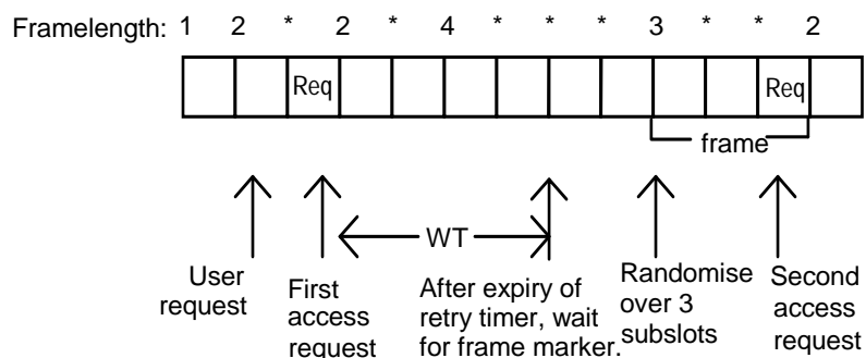
Figure 7.15: Example of random access procedure (BS using discrete access frames)
