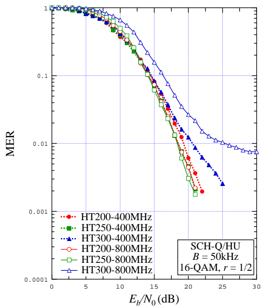
Figure 8.6: MER vs. E_b/N_0 for B = 50 kHz, SCH-Q/HU, 16-QAM r = 1/2 , various HT channels
