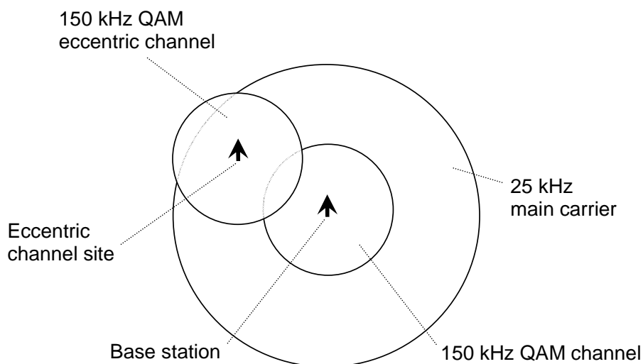
Figure 7.22: Example of a cell using an eccentric channel
