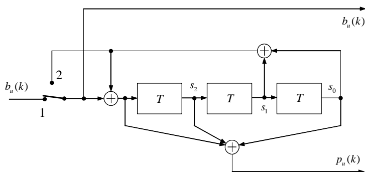
Figure 6.17: RSC encoder
