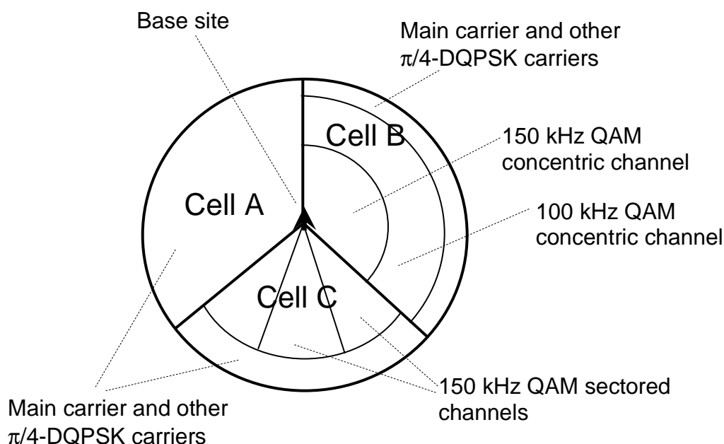
Figure 7.20: Example of CA sectored cells
