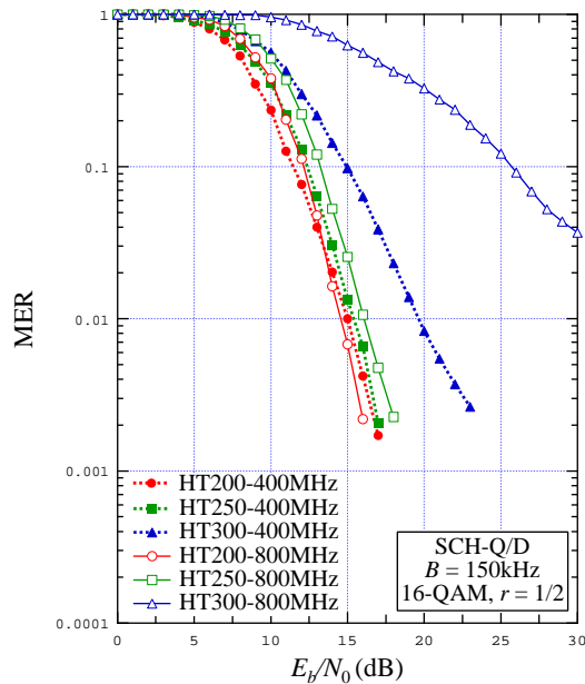
Figure 8.8: MER vs. E_b/N_0 for B = 150 kHz, SCH-Q/D, 16-QAM r = 1/2 , various HT channels
