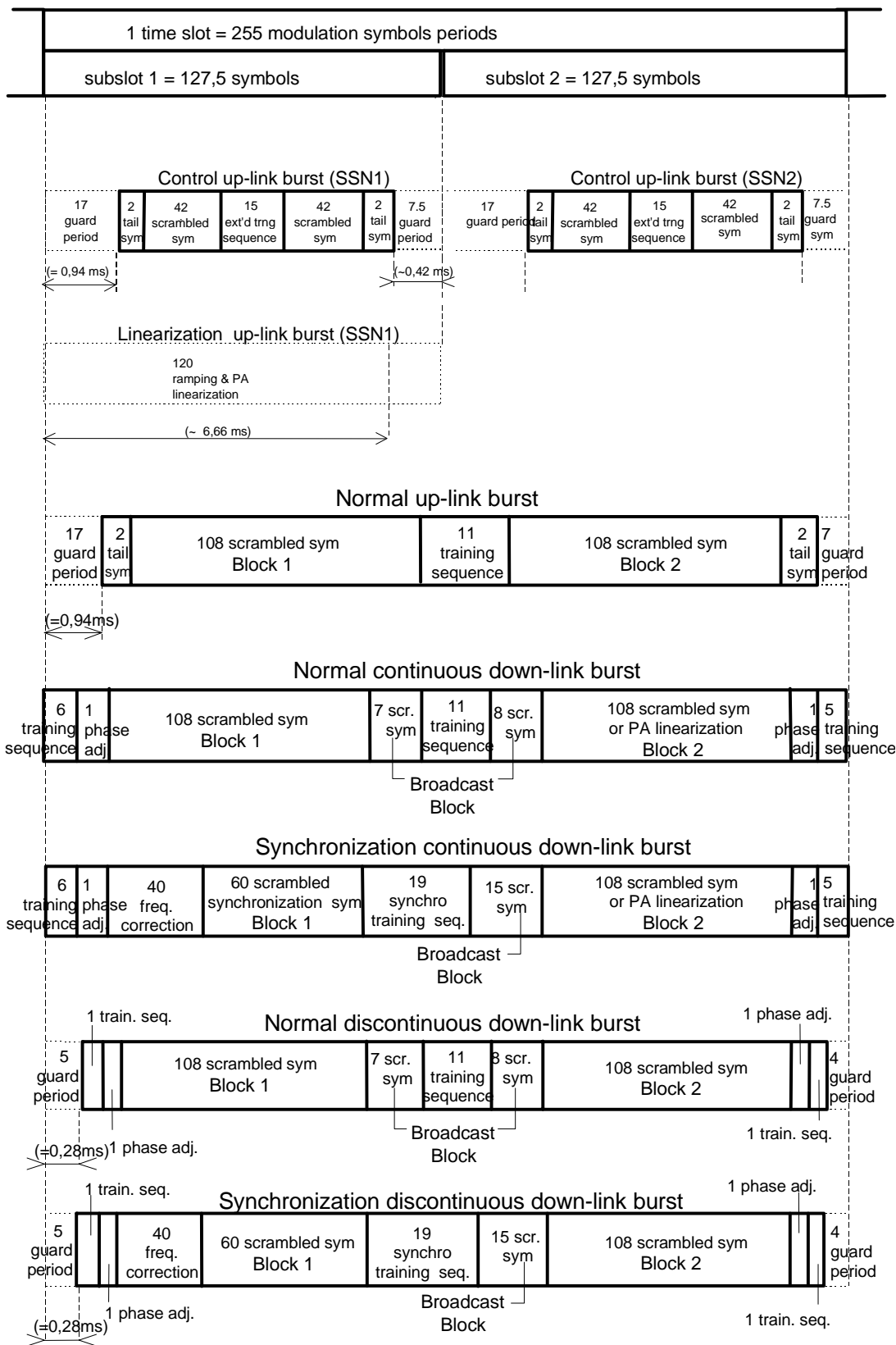
Figure 6.3: Burst types for phase modulation
