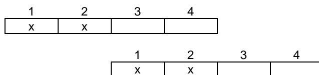
Figure 7.24: Frequency half duplex operation with fast switching capability
