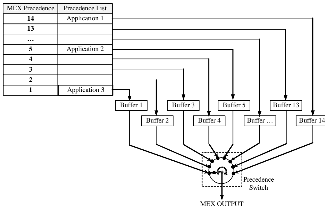
Figure 7.2: MEX precedence
