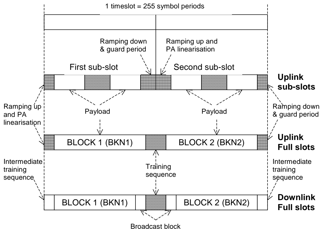
Figure 6.2: Physical layer basic slot structure for phase modulation
