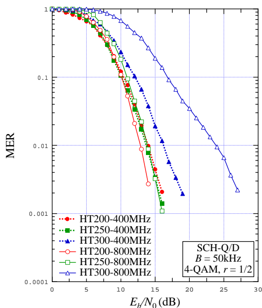
Figure 8.2: MER vs. E_b/N_0 for B = 50 kHz, SCH-Q/D, 4-QAM r = 1/2 , various HT channels
