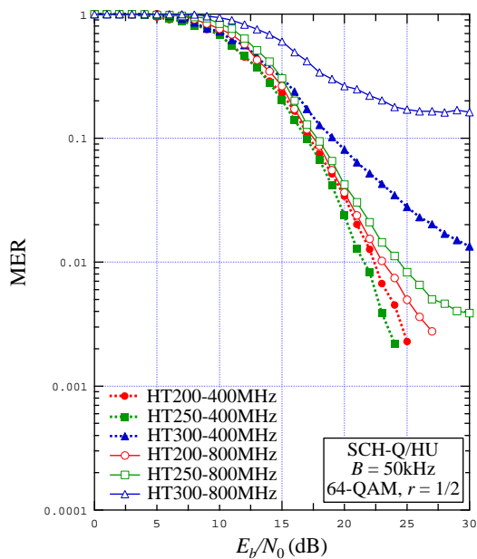
Figure 8.7: MER vs. E_b/N_0 for B = 50 kHz, SCH-Q/HU, 64-QAM r = 1/2 , various HT channels
