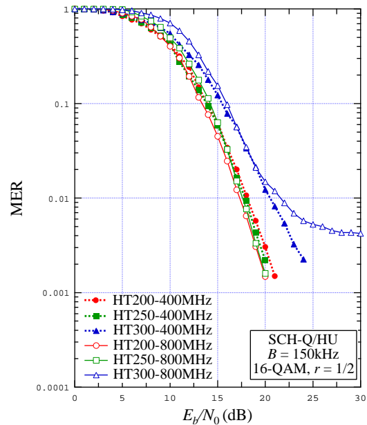
Figure 8.9: MER vs. E_b/N_0 for B = 150 kHz, SCH-Q/HU, 16-QAM r = 1/2 , various HT channels
