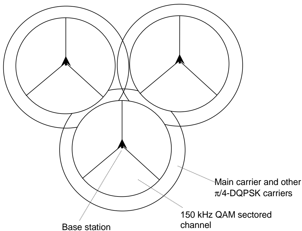
Figure 7.19: Example of CA cells using sectored channels
