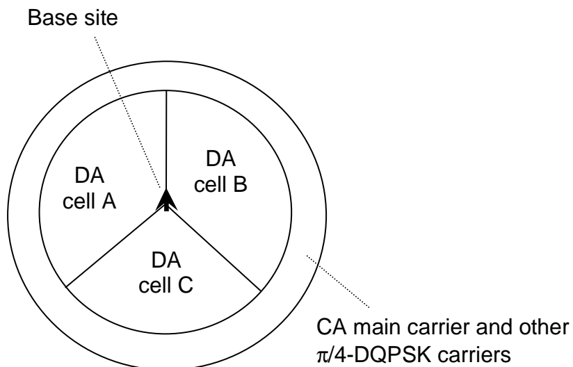
Figure 7.21: Example of a fully super-sectored umbrella channel with DA sectored cells
