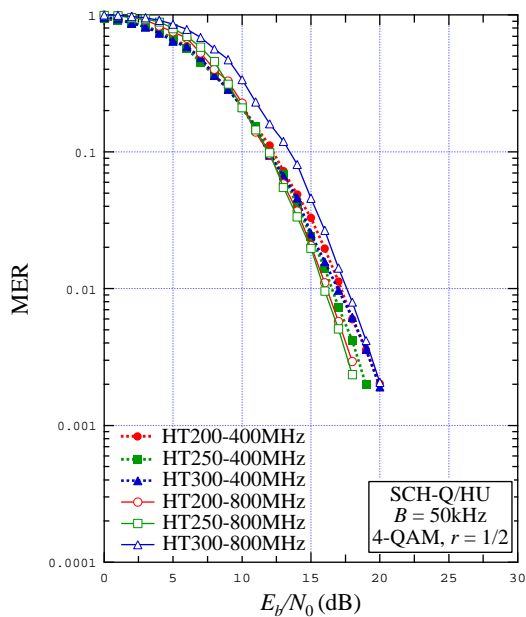
Figure 8.5: MER vs. E_b/N_0 for B = 50 kHz, SCH-Q/HU, 4-QAM r = 1/2 , various HT channels
