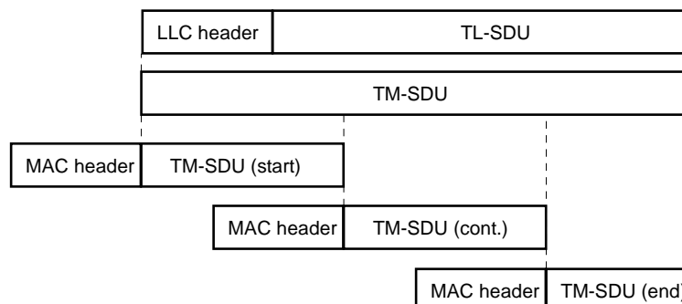
Figure 7.7: MAC fragmentation of a long TM-SDU
