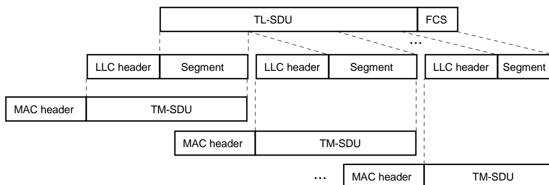
Figure 7.8: Advanced link segmentation by the LLC
