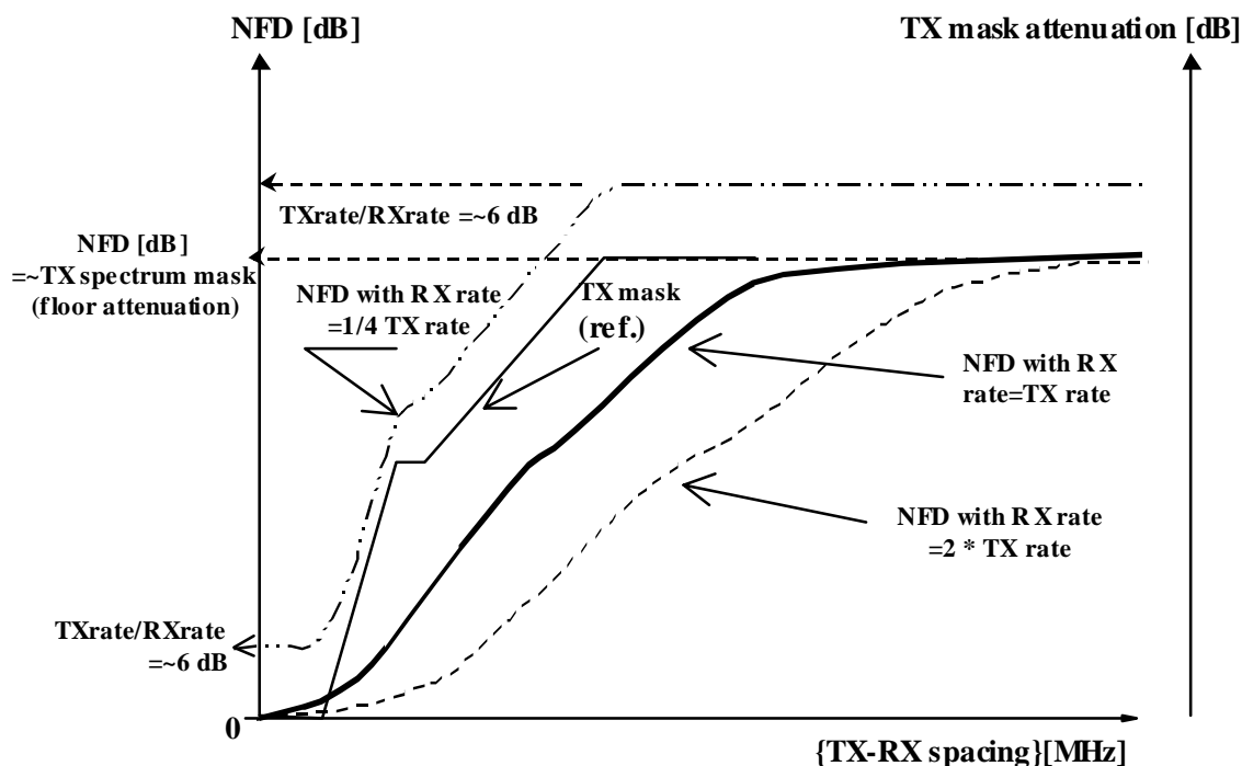
Figure 4: Qualitative examples of mixed NFD among different rate systems of the same class
