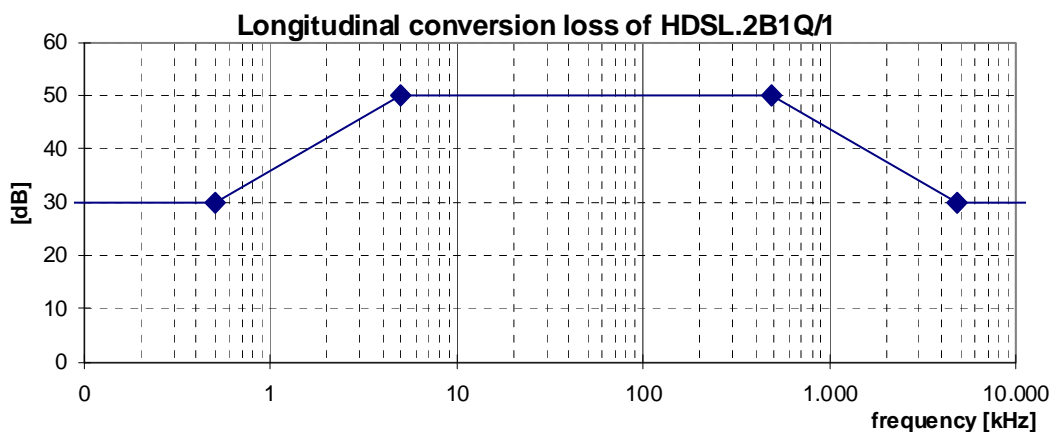
Figure 17: Minimum longitudinal conversion loss for a HDSL.2B1Q/1 signal source
