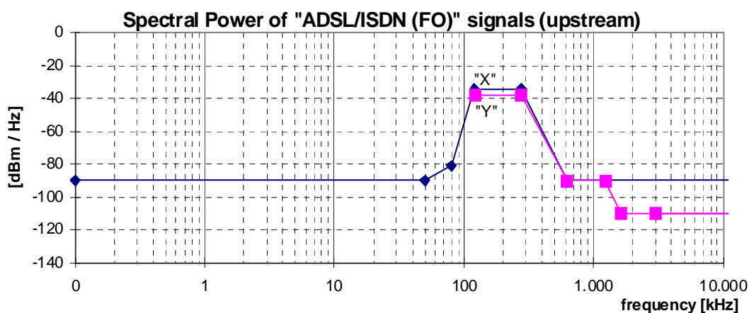
Figure 44: Spectral Power, for "ADSL/ISDN (FO)" signals, as specified in table 75
