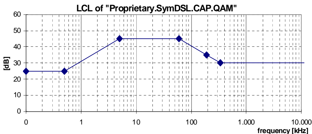
Figure 11: Minimum LCL for a "Proprietary.SymDSL.CAP.QAM" signal source
