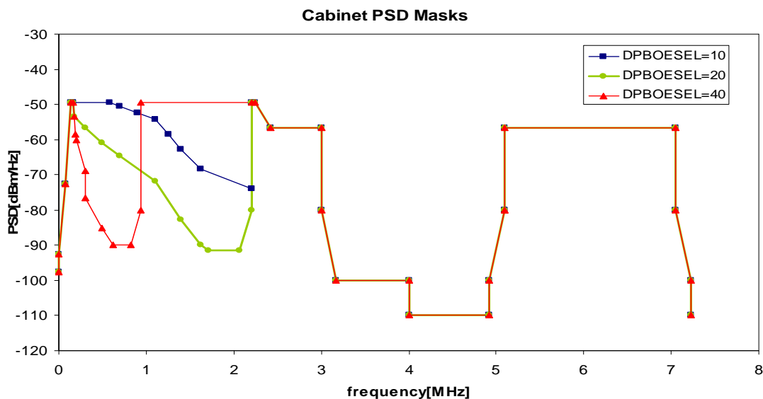
Figure 67: Spectral power for "VDSL2-UK1" downstream signals, as specified in tables 105 and 106, for different values of DPBOESEL
