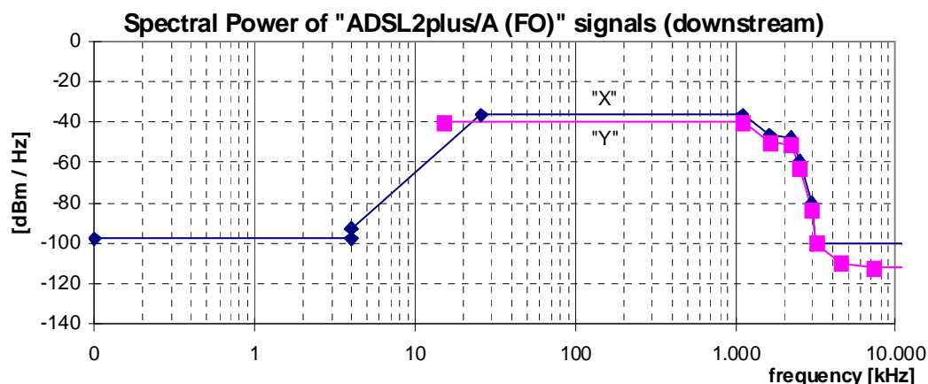
Figure 47: Spectral Power, for downstream "ADSL2plus/A (FO)", as specified in table 80
