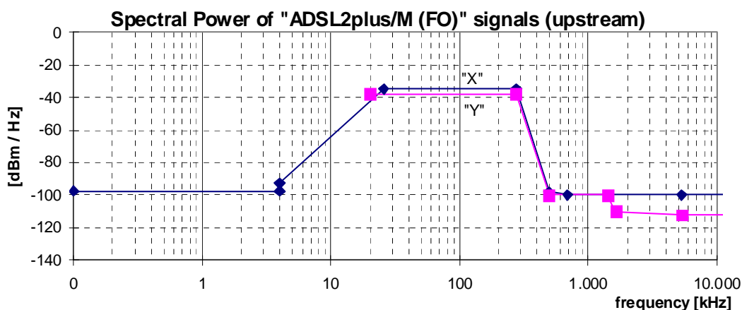
Figure 58: Spectral Power, for upstream ADSL2plus/M (FO) signals, as specified in table 93
