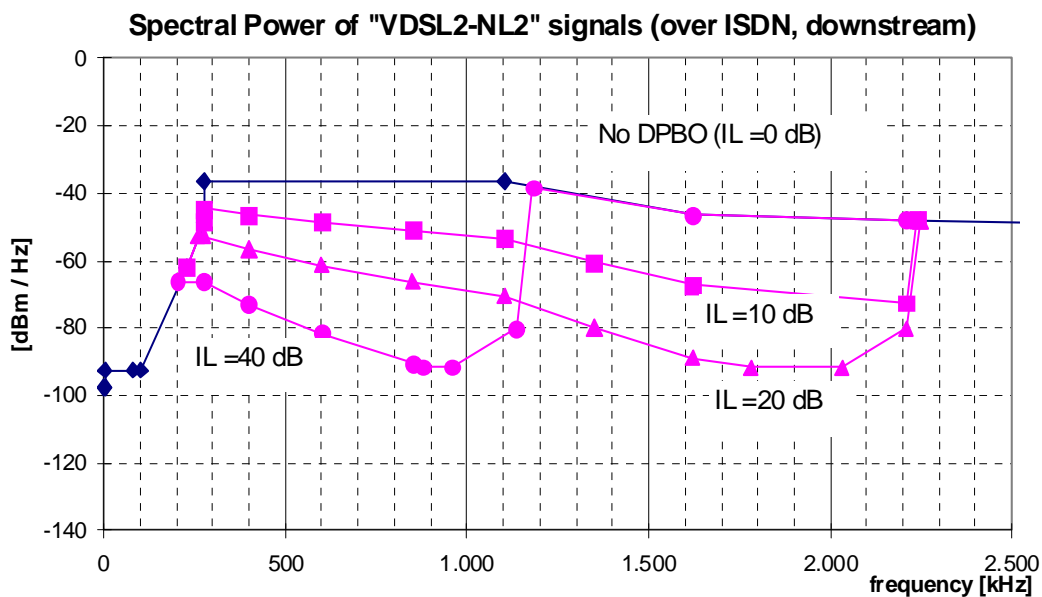
Figure 65: Spectral Power for "VDSL2-NL2" downstream signals (over ISDN), as specified in tables 102 and 103 in the frequency region where downstream PSD Shaping has been applied
