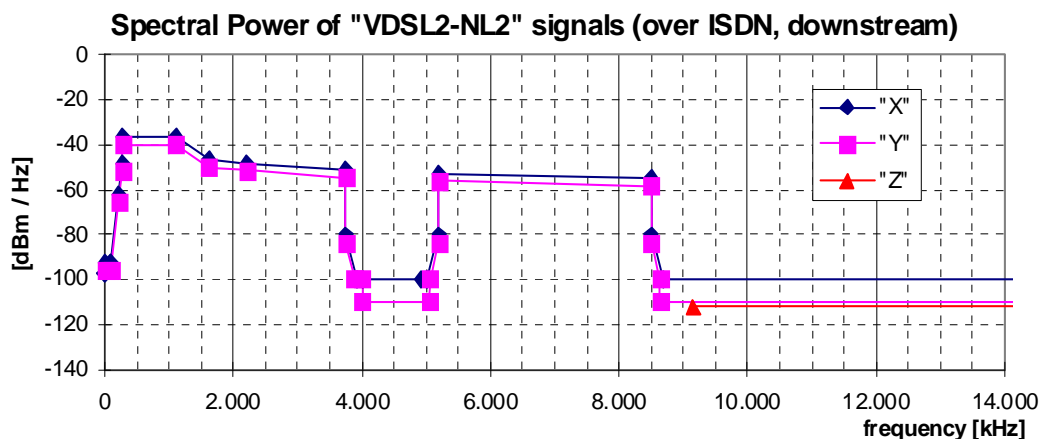
Figure 64: Spectral Power for "VDSL2-NL2" downstream signals (over ISDN), as specified in tables 102 and 103 for IL=0 dB
