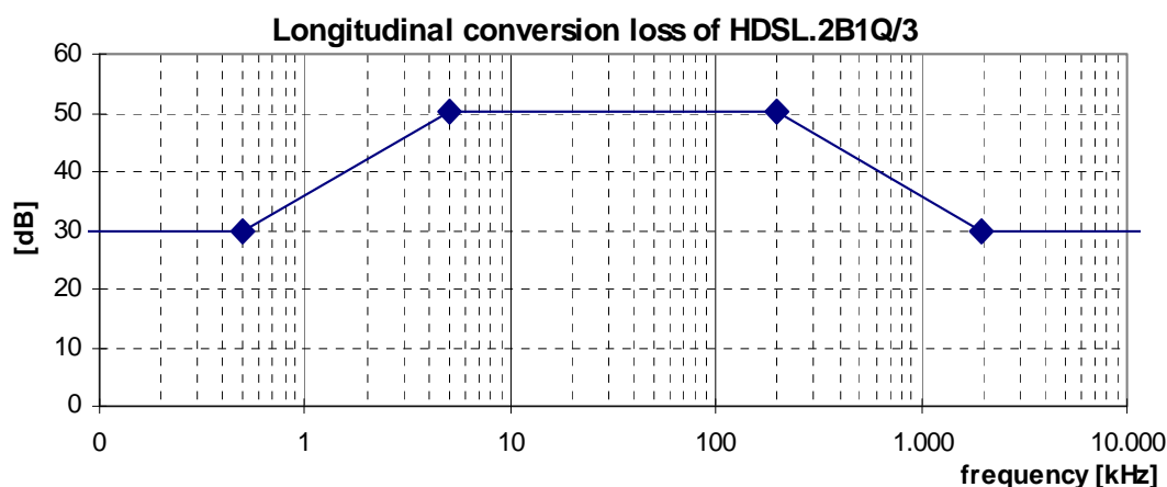
Figure 13: Minimum longitudinal conversion loss for a HDSL.2B1Q/3 signal source (392 kbaud/wirepair)
