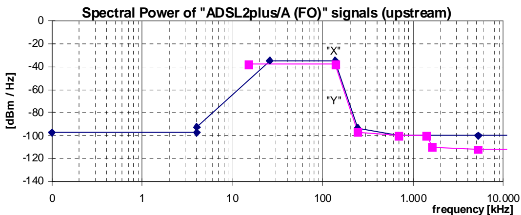
Figure 48: Spectral Power, for upstream "ADSL2plus/A (FO)" signals, as specified in table 81
