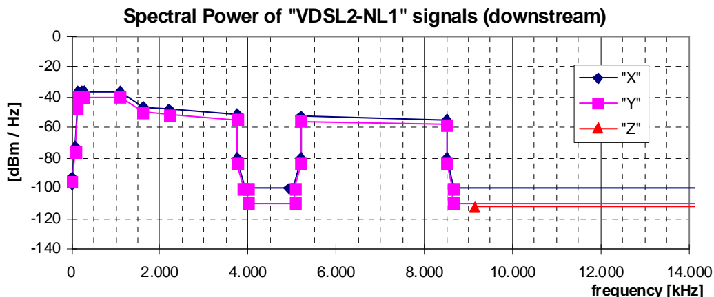
Figure 59: Spectral Power for "VDSL2-NL1" downstream signals, as specified in tables 95 and 96 for IL=0 dB
