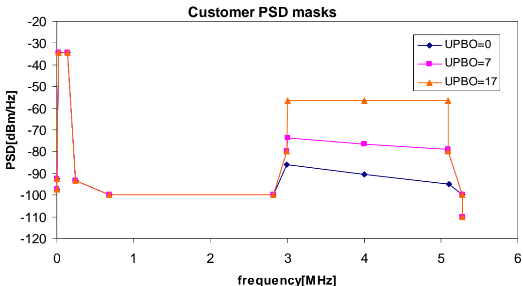
Figure 68: Spectral power for "VDSL2-UK1" upstream signals, as specified in tables 107 and 108, for different values of UPBO
