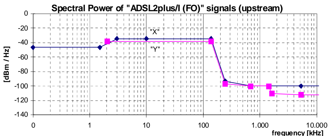
Figure 56: Spectral Power, for upstream "ADSL2plus/I (FO)" signals, as specified in table 91
