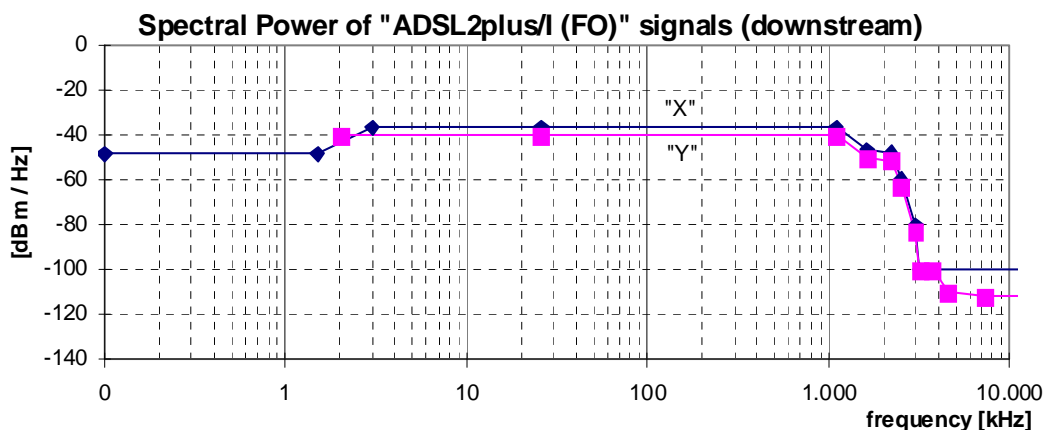
Figure 55: Spectral Power, for downstream "ADSL2plus/I (FO)" signals, as specified in table 90
