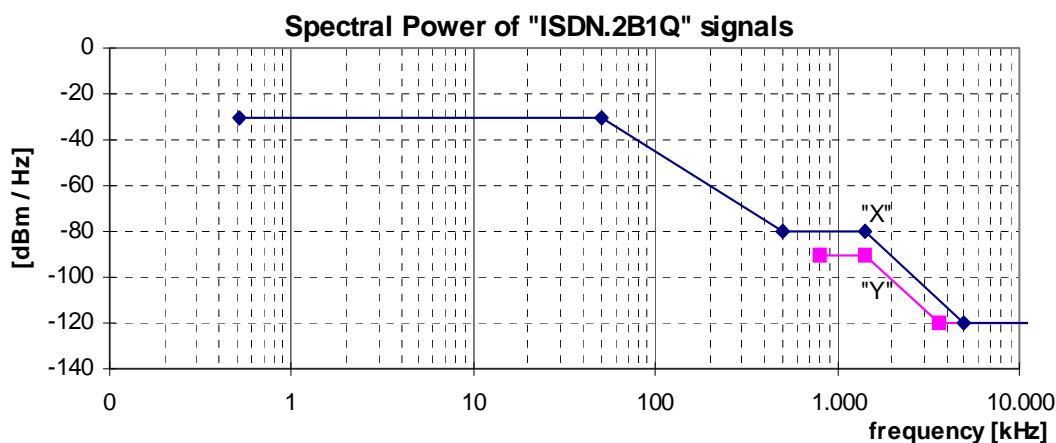
Figure 6: Spectral Power, for ISDN.2B1Q signals, as specified in table 7
