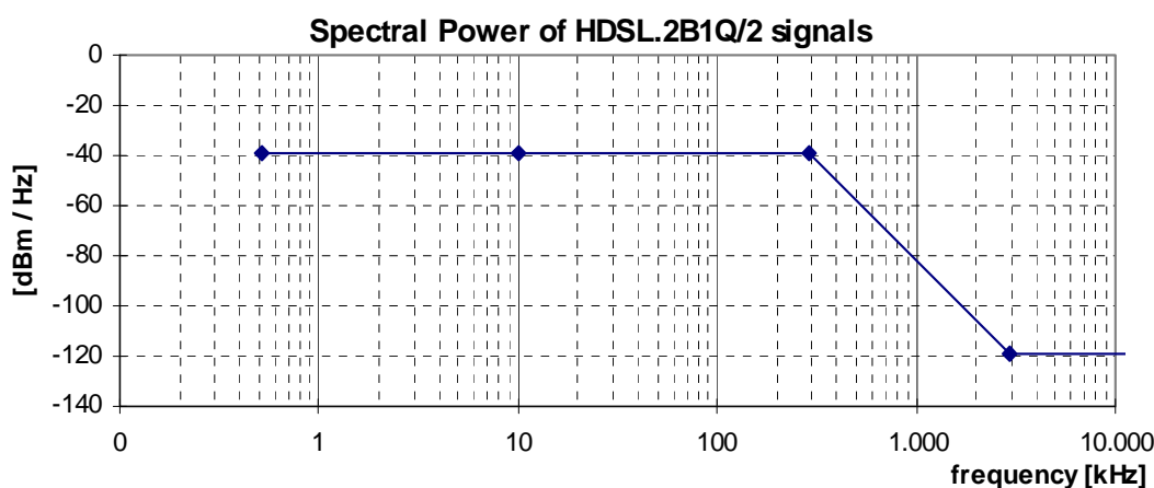
Figure 14: Spectral Power, for HDSL.2B1Q/2 signals, as specified in table 19
