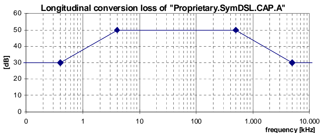
Figure 27: Minimum longitudinal conversion loss for a "Proprietary.SymDSL.CAP.A::261" signal source
