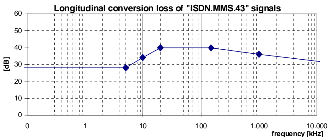
Figure 9: Minimum longitudinal conversion loss for a "ISDN.MMS43" signal source
