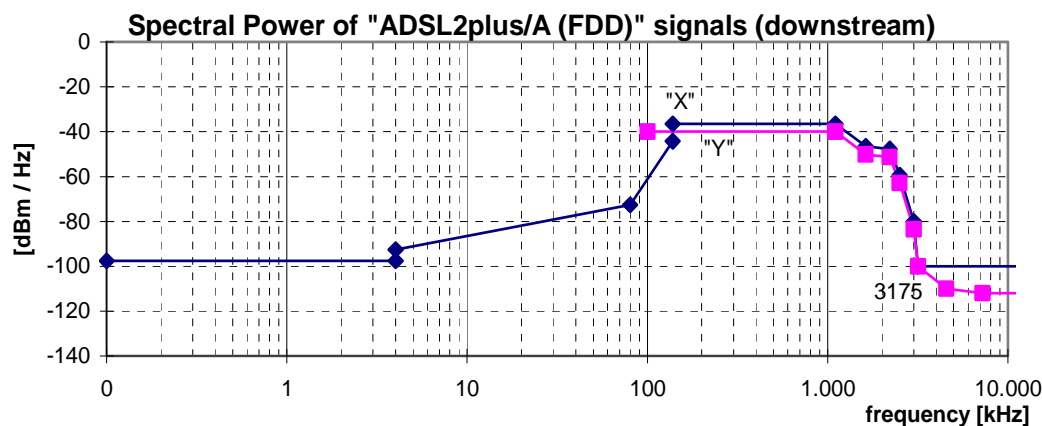
Figure 50: Spectral Power, for downstream "ADSL2plus/A (FDD)" signals, as specified in table 84
