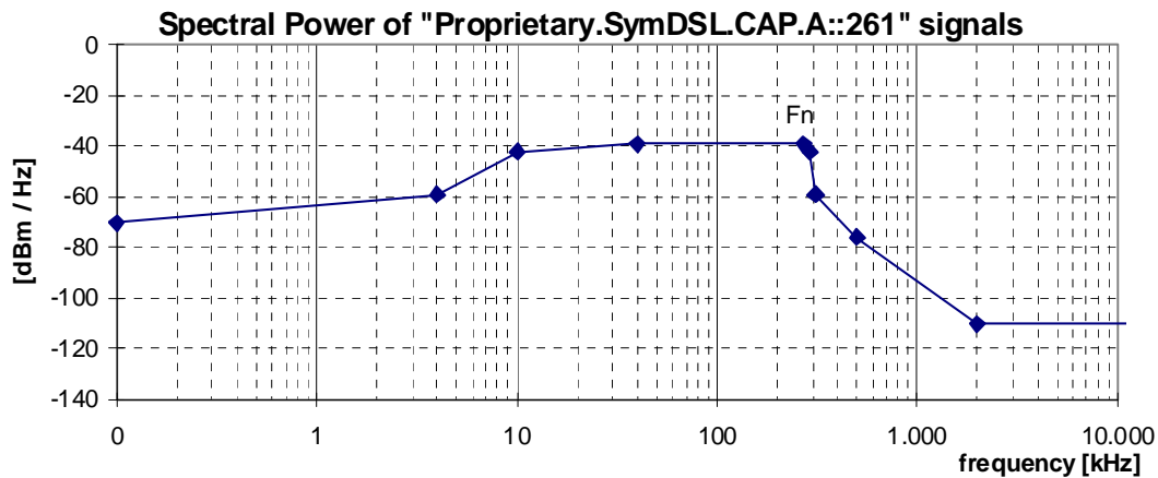
Figure 26: Spectral Power, for "Proprietary.SymDSL.CAP.A::261" signals (at F_N = 261 kHz), as specified in table 41
