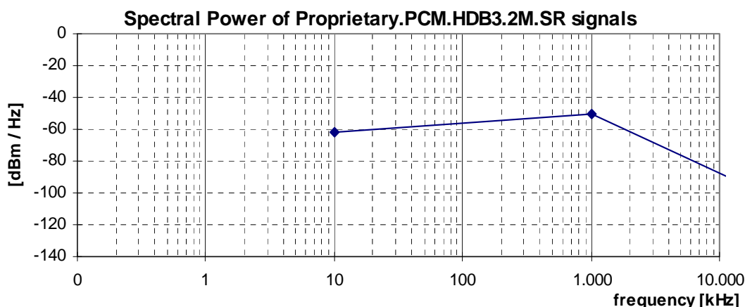
Figure 36: Spectral Power, for Proprietary.PCM.HDB3.2M.SR signals, as specified in table 62
