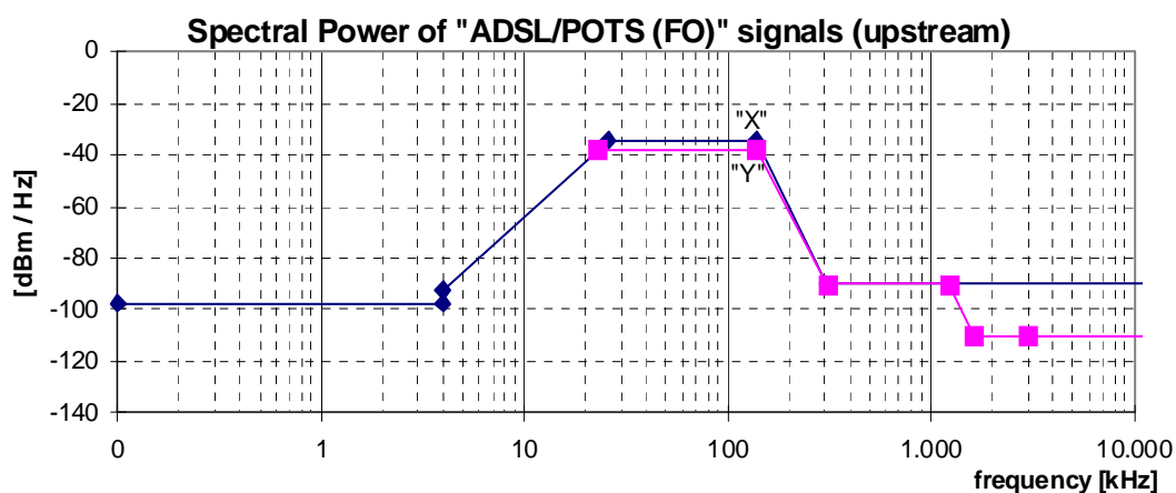
Figure 40: Spectral Power, for "ADSL/POTS (FO)" signals, as specified in table 68
