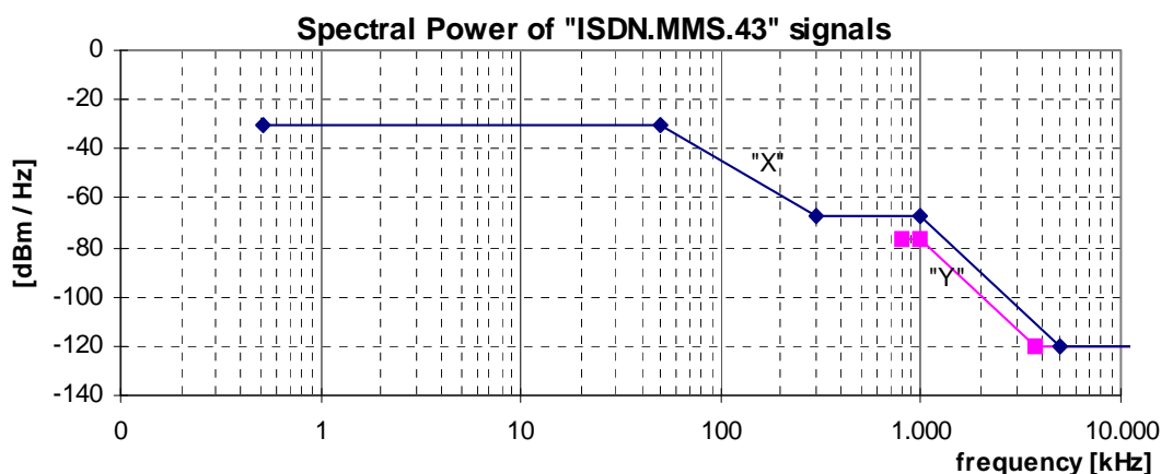
Figure 8: Spectral Power, for "ISDN.MMS.43" signals, as specified in table 10
