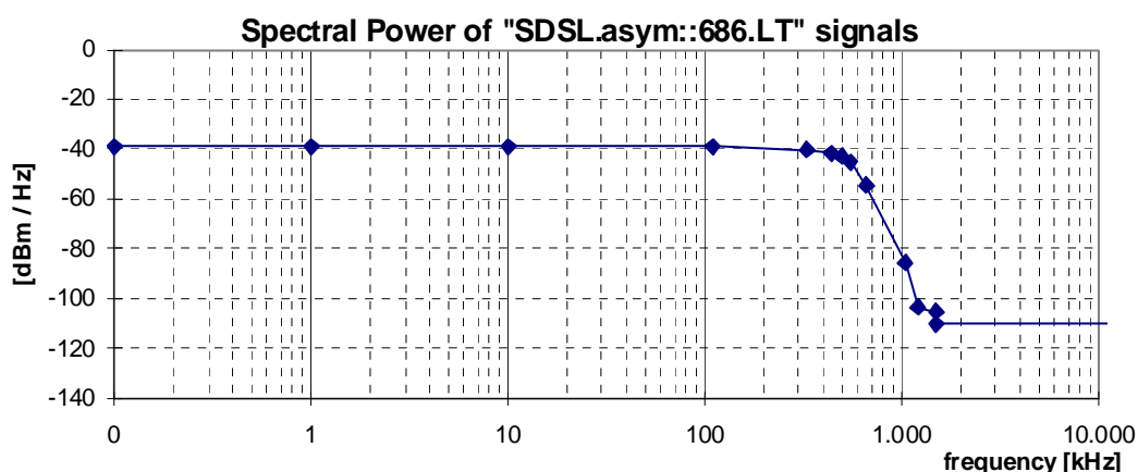
Figure 24: Spectral Power, for "SDSL.asym::686.LT" signal, as specified in table 36
