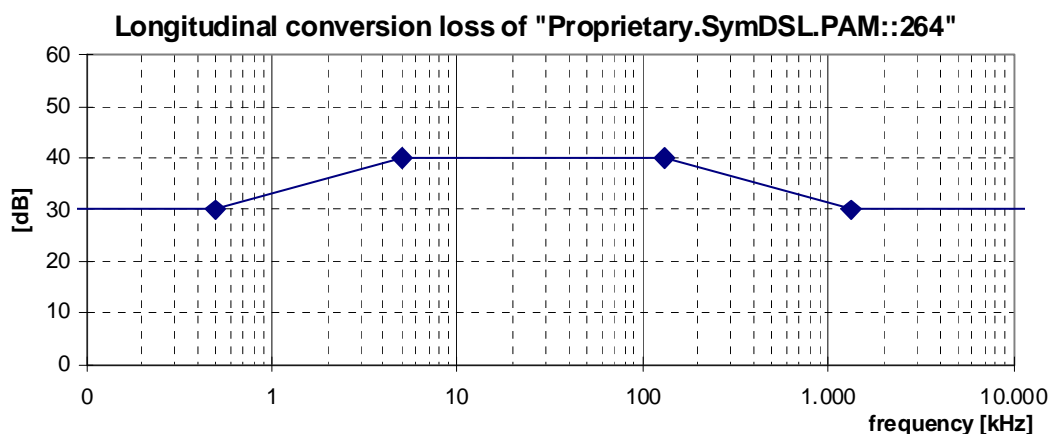
Figure 33: Minimum longitudinal conversion loss for a "Proprietary.SymDSL.PAM::264" signal source
