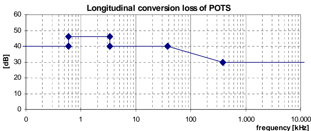
Figure 4: Minimum longitudinal conversion loss for a POTS-signal source
