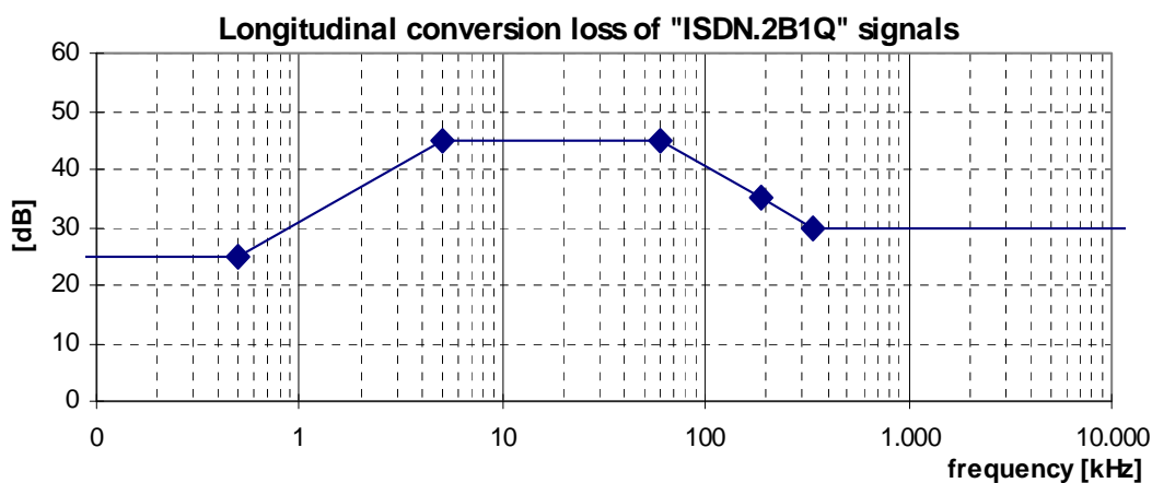
Figure 7: Minimum longitudinal conversion loss for a "ISDN.2B1Q" signal source
