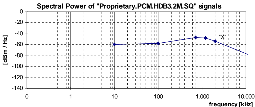
Figure 38: Spectral Power, for Proprietary.PCM.HDB3.2M.SQ signals, as specified in table 65
