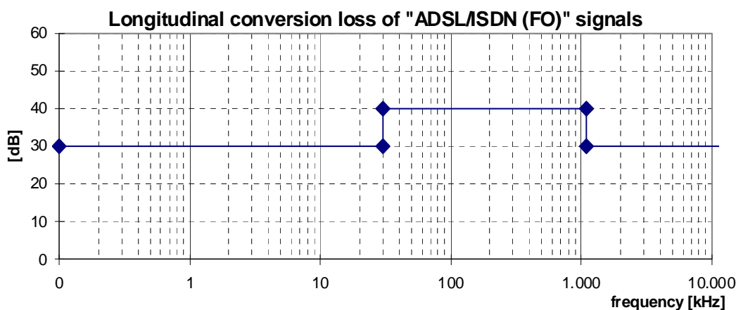
Figure 45: Minimum longitudinal conversion loss
