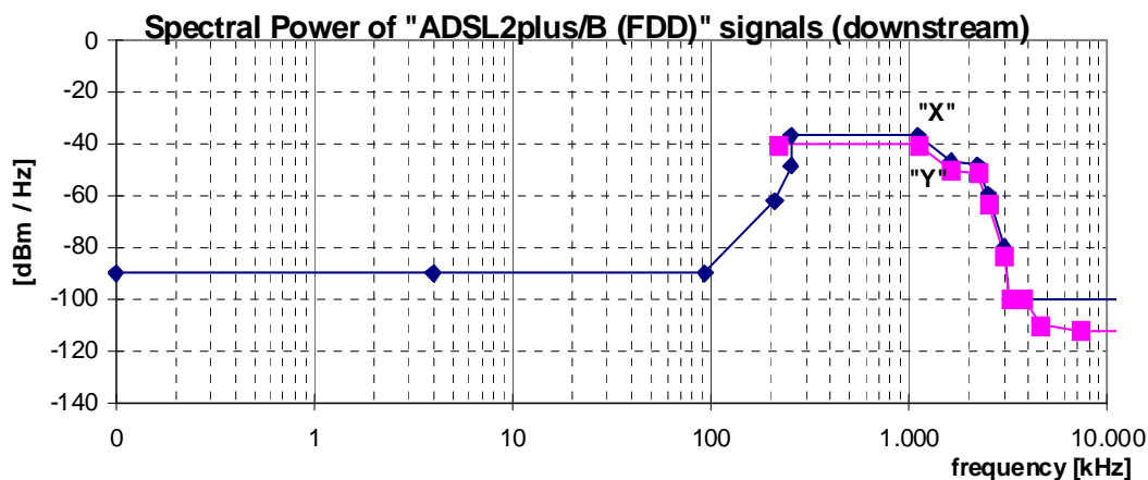
Figure 54: Spectral Power, for downstream "ADSL2plus/B (FDD)" signals, specified in table 89
