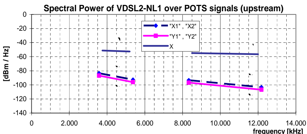
Figure 62: Spectral Power for "VDSL2-NL1" upstream receive signals, as specified in table 98
