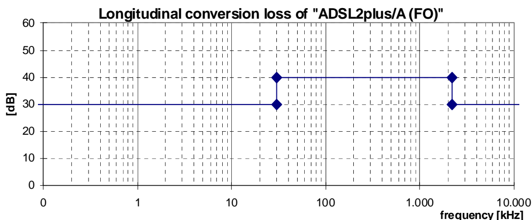
Figure 49: Minimum longitudinal conversion loss
