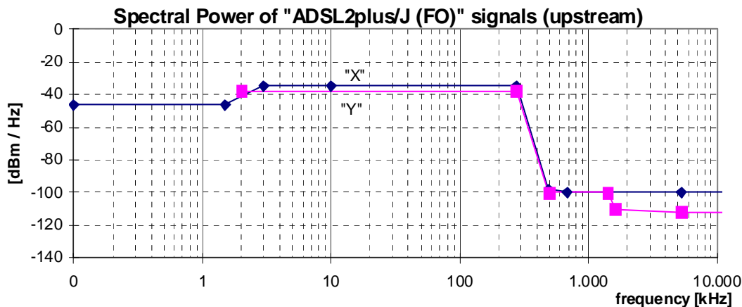
Figure 57: Spectral Power, for upstream "ADSL2plus/J (FO)" signals, as specified in table 92
