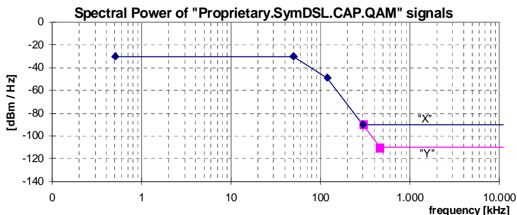
Figure 10: Spectral Power, for "Proprietary.SymDSL.CAP.QAM" signals, as specified in table 13
