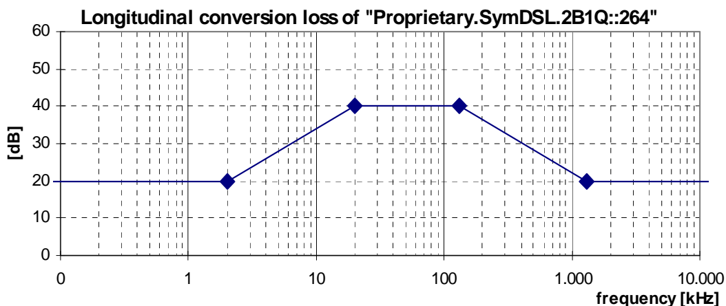
Figure 35: Minimum longitudinal conversion loss for a "Proprietary.SymDSL.2B1Q::264" signal source
