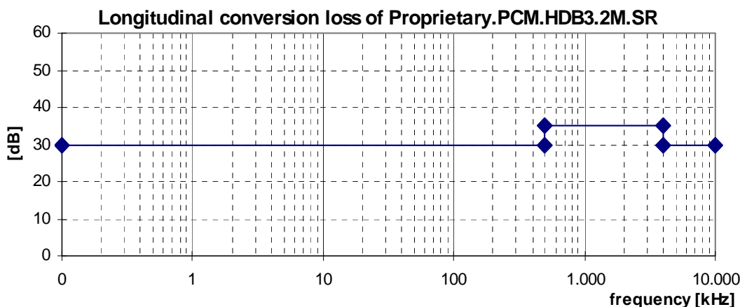
Figure 37: Minimum longitudinal conversion loss for a "Proprietary.PCM.HDB3.2M.SR" signal source
