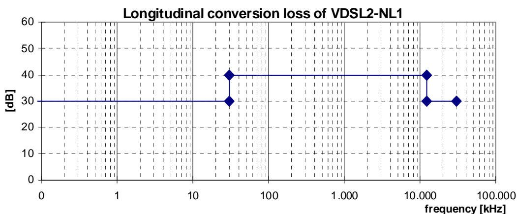
Figure 63: Minimum longitudinal conversion loss
