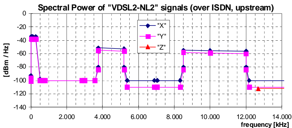
Figure 66: Spectral Power, for "VDSL2-NL2" upstream signals (over ISDN), as specified in table 104
