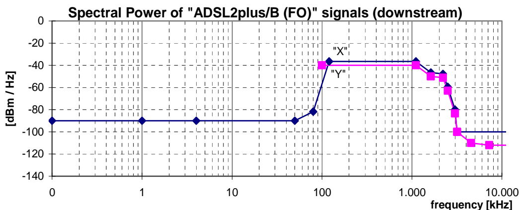
Figure 51: Spectral Power, for downstream "ADSL2plus/B (FO)" signals, as specified in table 85
