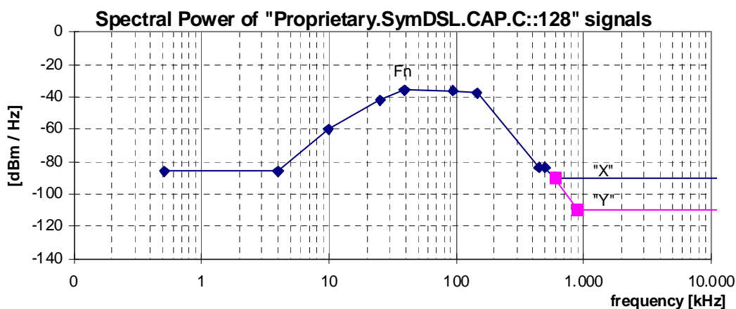
Figure 30: Spectral Power, for "Proprietary.SymDSL.CAP.C::128" signals (at F_N = 128 kHz), as specified in table 49
