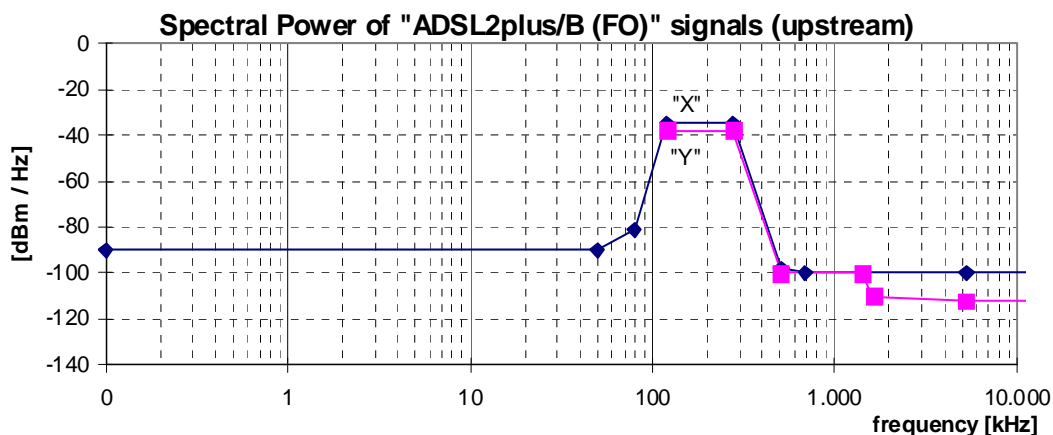
Figure 52: Spectral Power, for upstream "ADSL2plus/B (FO)" signals, as specified in table 86
