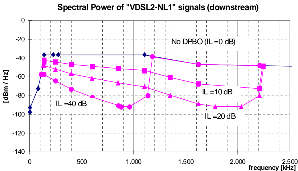
Figure 60: Spectral Power for "VDSL2-NL1" downstream signals, as specified in tables 95 and 96, for a frequency band where downstream PSD Shaping has been applied
