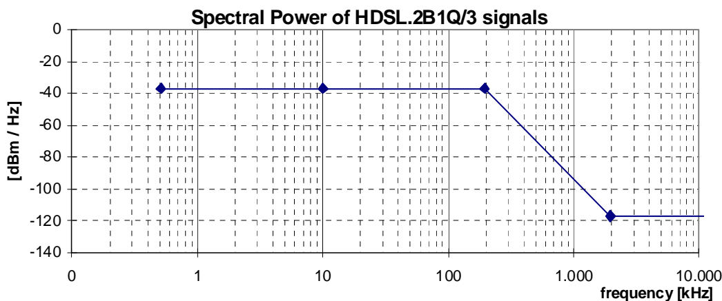
Figure 12: Spectral Power, for HDSL.2B1Q/3 signals, as specified in table 16
