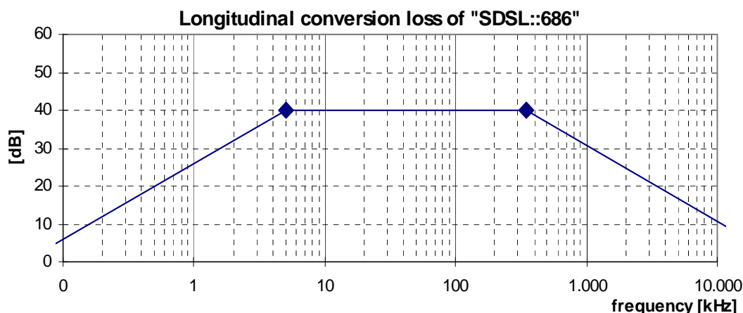
Figure 21: Minimum longitudinal conversion loss for a "SDSL::686" signal source
