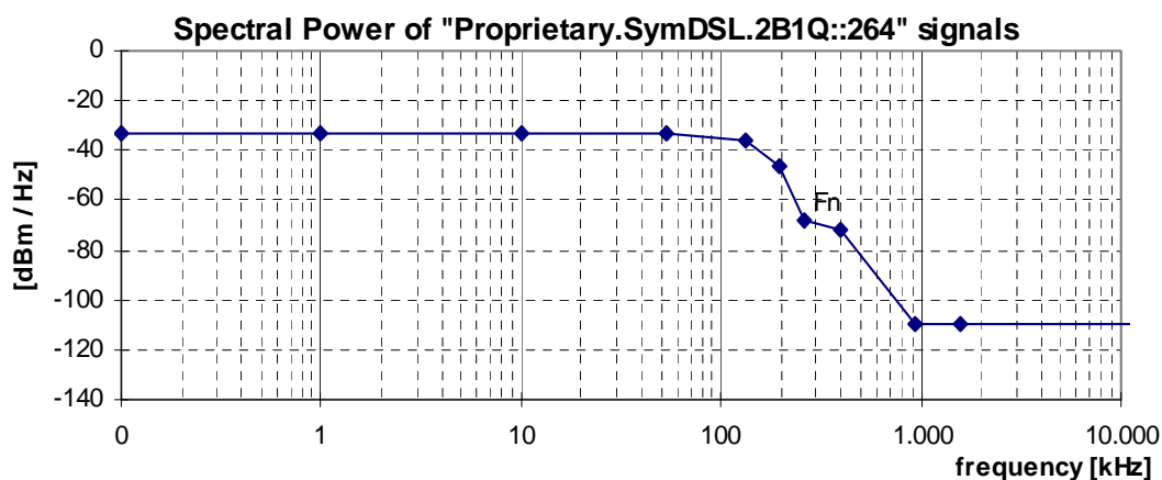
Figure 34: Spectral Power, for "Proprietary.SymDSL.2B1Q::264" signals (at F_N = 264 kHz), as specified in table 53
