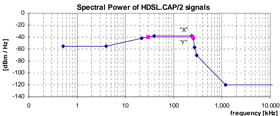
Figure 18: Spectral Power, for HDSL.CAP/2 signals, as specified in table 25
