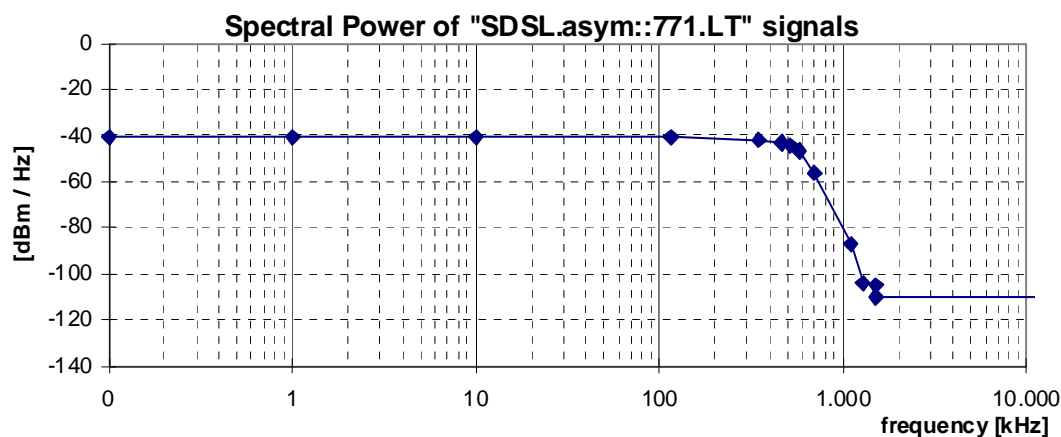
Figure 25: Spectral Power, for "SDSL.asym::771.LT" signal, as specified in table 36
