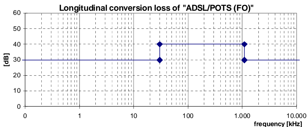
Figure 41: Minimum longitudinal conversion loss
