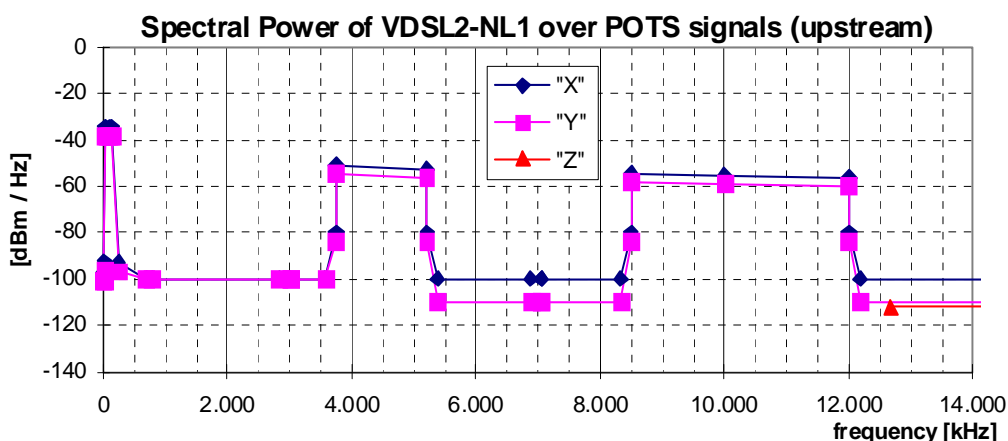
Figure 61: Spectral Power for "VDSL2-NL1" upstream transmit signals, as specified in table 97
