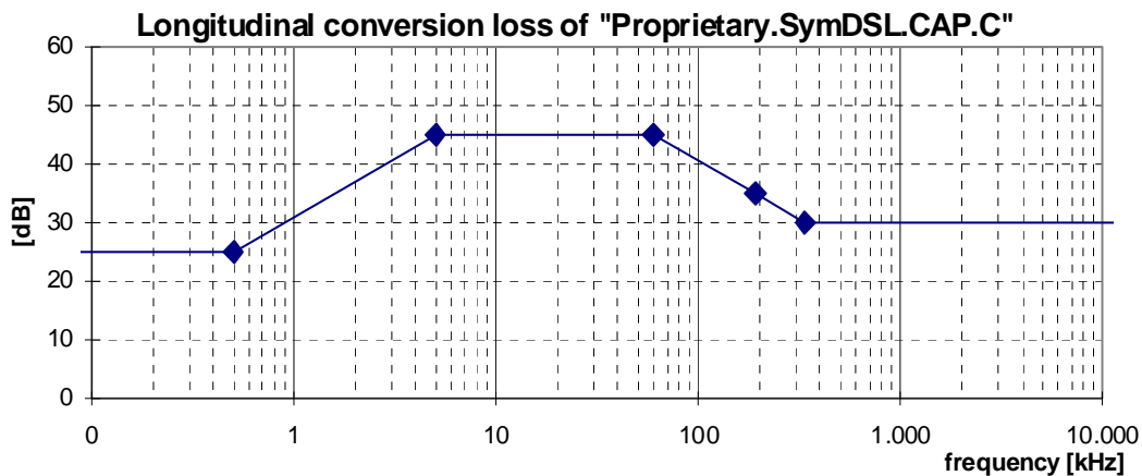
Figure 31: Minimum longitudinal conversion loss for a "Proprietary.SymDSL.CAP.C::Fn" signal source
