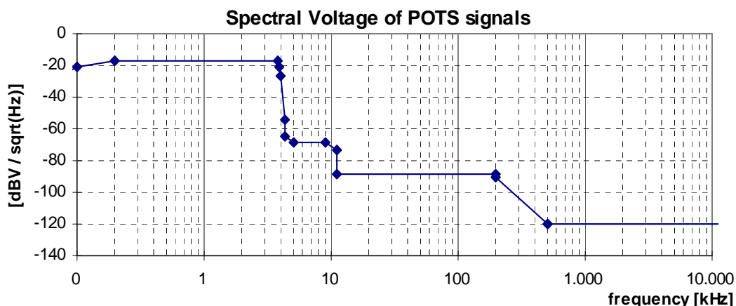
Figure 3: Spectral Voltage, for POTS signals, as specified in table 1
