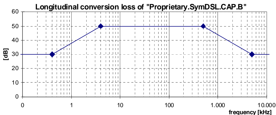
Figure 29: Minimum longitudinal conversion loss for a "Proprietary.SymDSL.CAP.B::261" signal source
