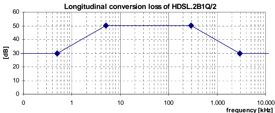
Figure 15: Minimum longitudinal conversion loss for a HDSL.2B1Q/2 signal source (584 kbaud/wirepair)
