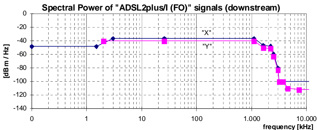
Figure 55: Spectral Power, for downstream "ADSL2plus/l (FO)" signals, as specified in table 90
