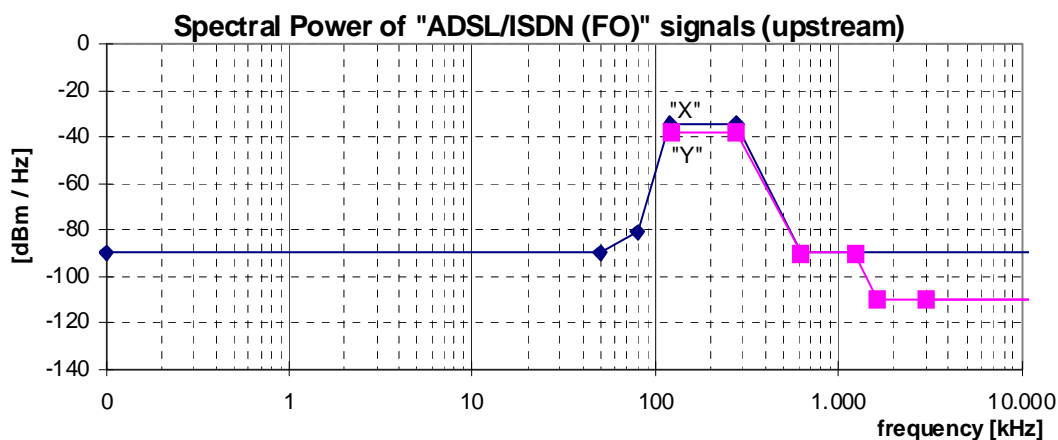
Figure 44: Spectral Power, for "ADSL/ISDN (FO)" signals, as specified in table 75
