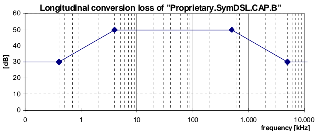
Figure 29: Minimum longitudinal conversion loss for a "Proprietary.SymDSL.CAP.B::261" signal source
