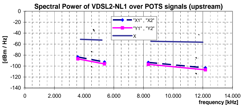
Figure 62: Spectral Power for "VDSL2-NL1" upstream receive signals, as specified in table 98
