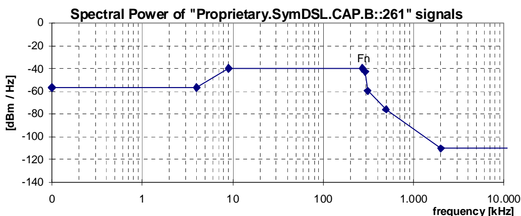
Figure 28: Spectral Power, for "Proprietary.SymDSL.CAP.B::261" signals (at F_N = 261 kHz), as specified in table 45
