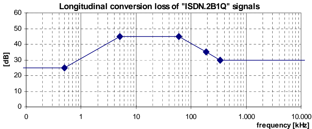
Figure 7: Minimum longitudinal conversion loss for a "ISDN.2B1Q" signal source
