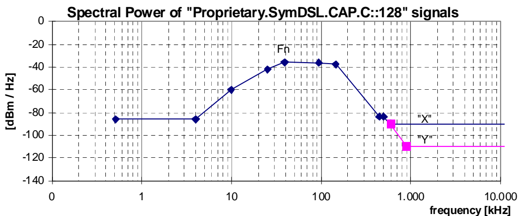
Figure 30: Spectral Power, for "Proprietary.SymDSL.CAP.C::128" signals (at F_N = 128 \text{ kHz} ), as specified in table 49
