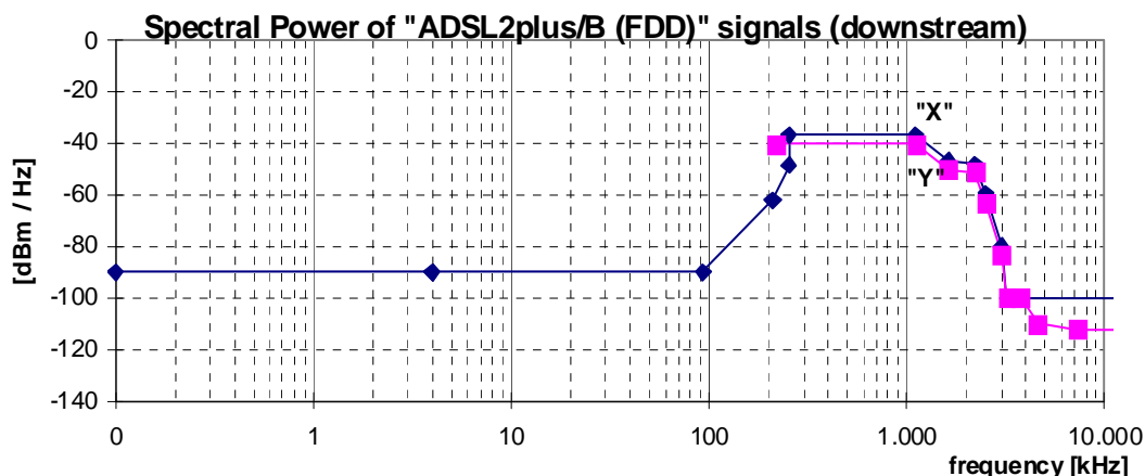
Figure 54: Spectral Power, for downstream "ADSL2plus/B (FDD)" signals, specified in table 89
