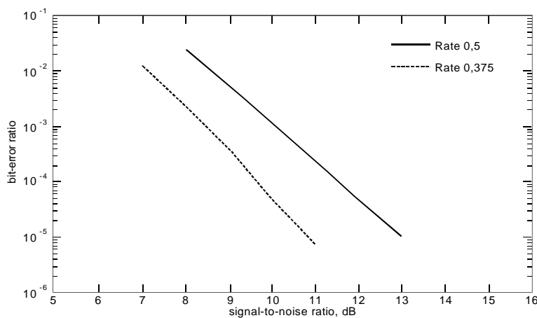
Figure 3: Performance of DAB in a simulated Raleigh Channel, Mode 2, Urban environment, 15 km/h speed, L-Band
