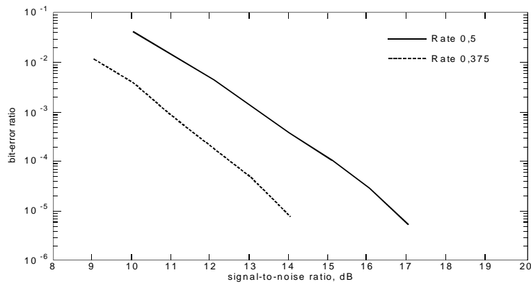
Figure 7: Performance of DAB in a simulated Raleigh Channel, Mode 3, Rural environment, 130 km/h speed, L-Band
