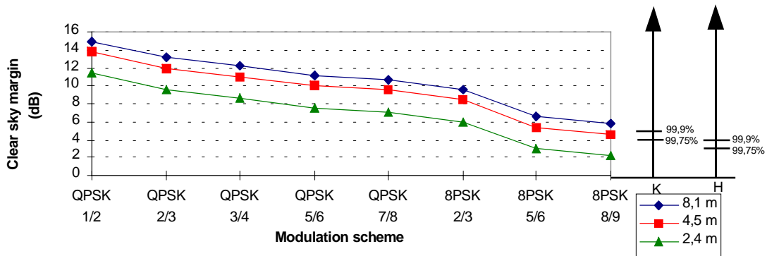
Figure 7: Clear sky margins for DSNG links (beam centre-to-beam centre), using transportable terminals of 1,5 m (useful EIRP 65 dBW) for different receiving earth stations (8,1 m, 4,5 m, 2,4 m)
