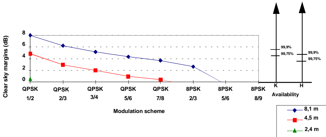
Figure 6: Clear sky margins for DSNG links (beam edge-to-beam edge), using transportable terminals of 1,5 m (useful EIRP 65 dBW) for different receiving earth stations (8,1 m, 4,5 m, 2,4 m)
