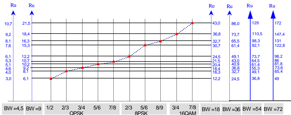
Figure 3b: Bit rate capacity versus available bandwidth (Ru in Mbit/s, and BW in MHz)
