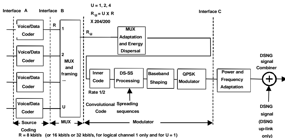
Figure 16: Functional block diagram of the System
