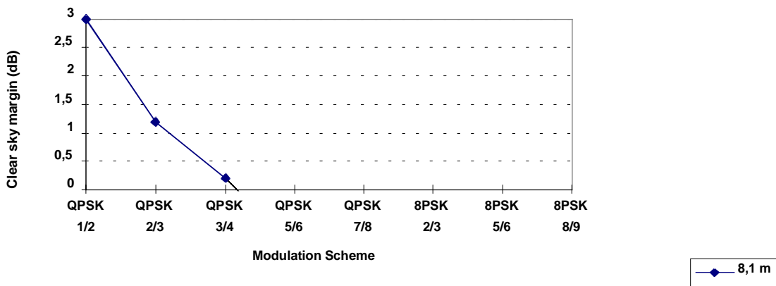
Figure 9: Clear sky margins for DSNG links (beam edge-to-beam edge), using transportable terminals of 0,9 m (useful EIRP 60 dBW) for different receiving earth stations (8,1 m, 4,5 m, 2,4 m)
