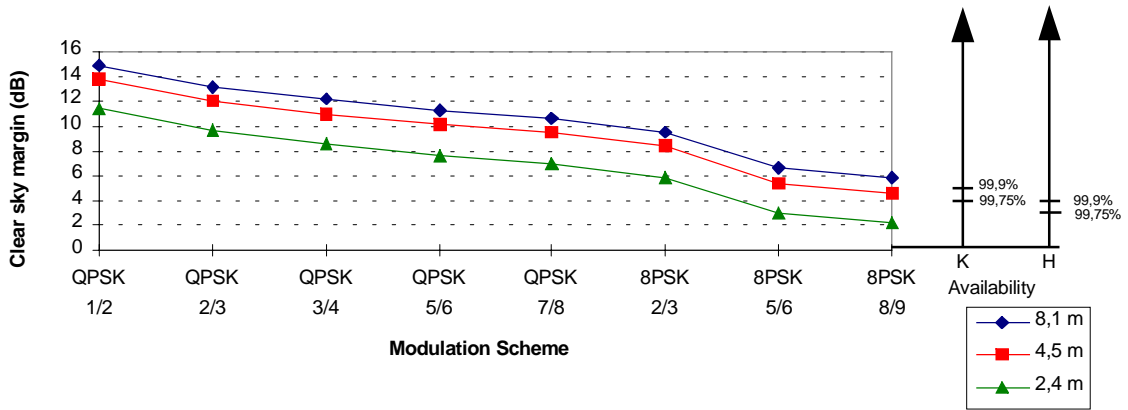
Figure 5: Clear sky margins for DSNG links (beam centre-to-beam centre), using transportable terminals of 1,8 m (useful EIRP 67 dBW) for different receiving earth stations (8,1 m, 4,5 m, 2,4 m)
