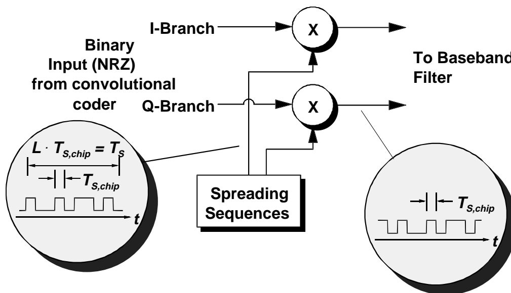
Figure 15: Basic principle of Direct-Sequence Spread-Spectrum coding
