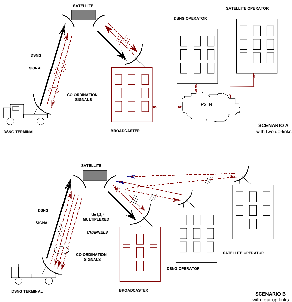
Figure 14: Example environments for DSNG and co-ordination channels transmissions by satellite
