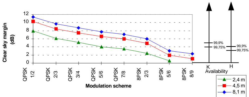
Figure 10: Clear sky margins for DSNG links (beam centre-to-beam centre), using transportable terminals of 0,9 m (useful EIRP 60 dBW) for different receiving earth stations (8,1 m, 4,5 m, 2,4 m)
