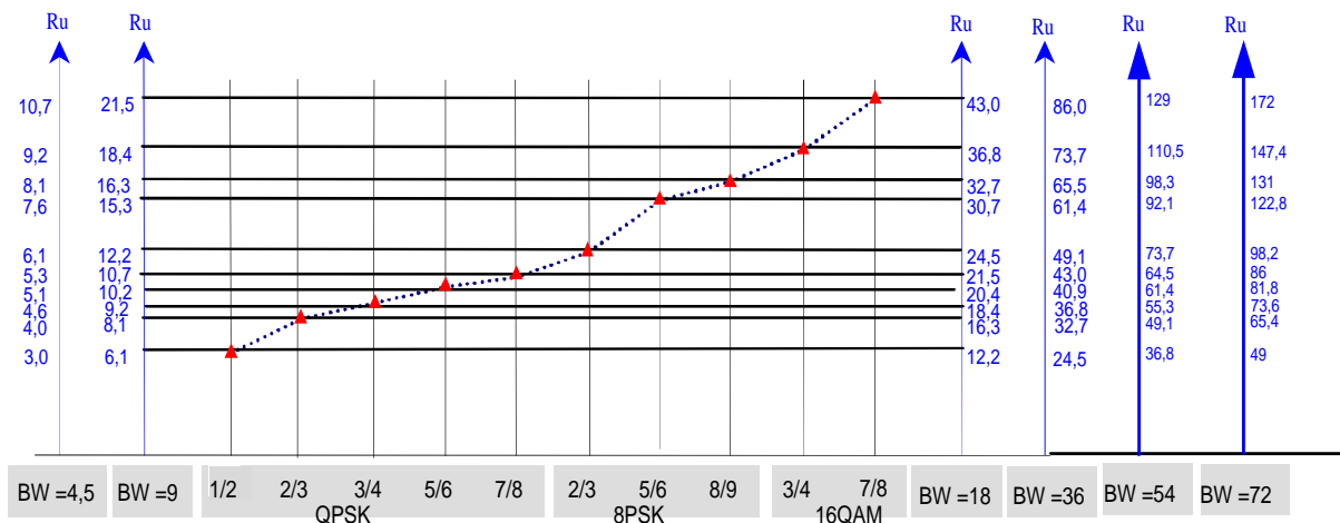
Figure 3a: Bit rate capacity versus available bandwidth (Ru in Mbit/s, and BW in MHz)
