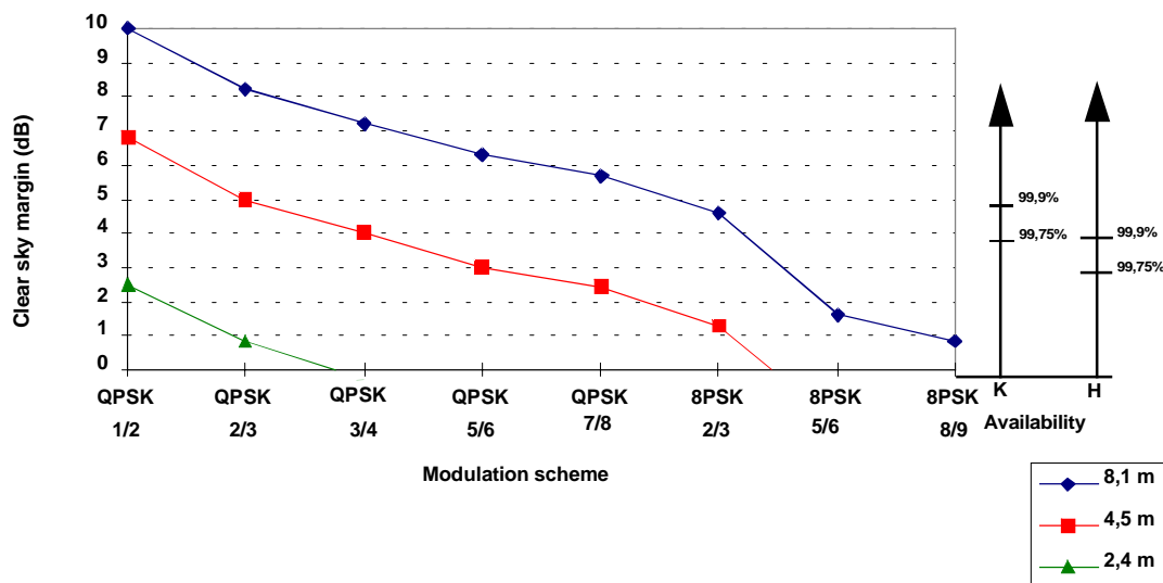
Figure 4: Clear sky margins for DSNG links (beam edge-to-beam edge), using transportable terminals of 1,8 m (useful EIRP 67 dBW) for different receiving earth stations (8,1 m, 4,5 m, 2,4 m)
