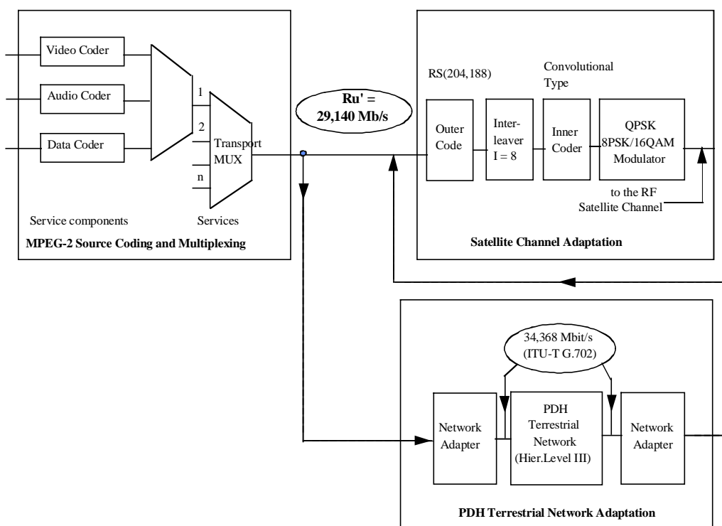
Figure 13: Example of Connection of the System with Terrestrial PDH Network following ETS 300 813 [12]
