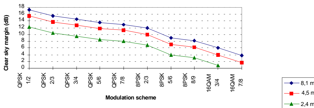
Figure 12: Clear sky margins for fixed contribution links considering different receiving earth stations (8,1 m, 4,5 m and 2,4 m) located at beam centre (Transponder operated in "Nominal Gain-3 dB")
