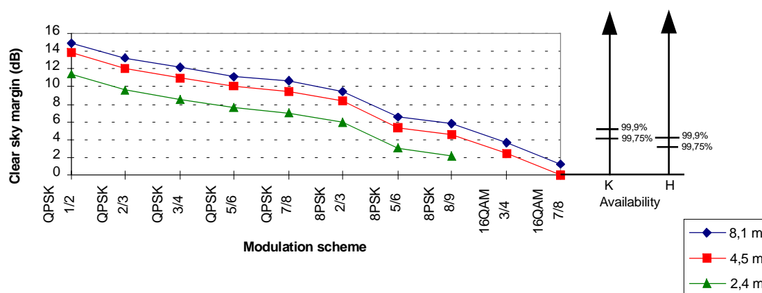
Figure 11: Clear sky margins for fixed contribution links considering different receiving earth stations (8,1 m, 4,5 m and 2,4 m) located at beam centre (Transponder operated in "Nominal Gain")
