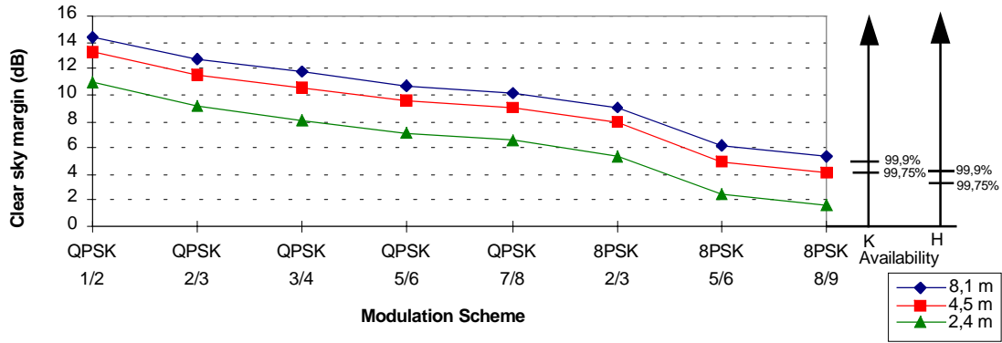
Figure 8: Clear sky margins for DSNG links (beam centre-to-beam centre), using transportable terminals of 1,2 m (useful EIRP 63 dBW) for different receiving earth stations (8,1 m, 4,5 m, 2,4 m)
