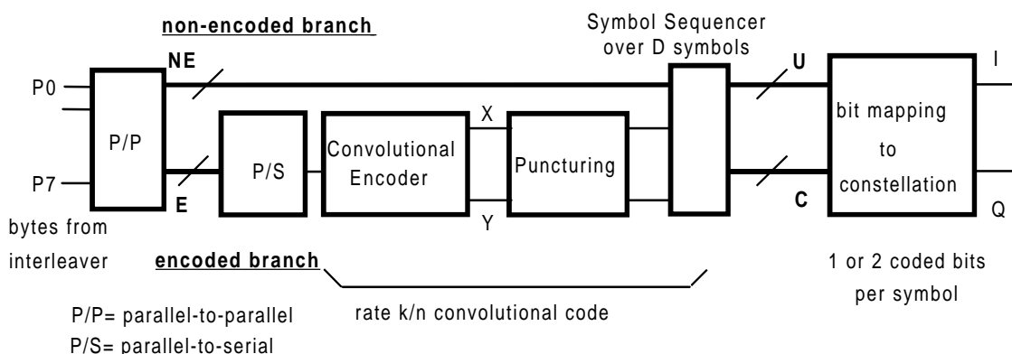
Figure 2: Inner trellis coder principle
