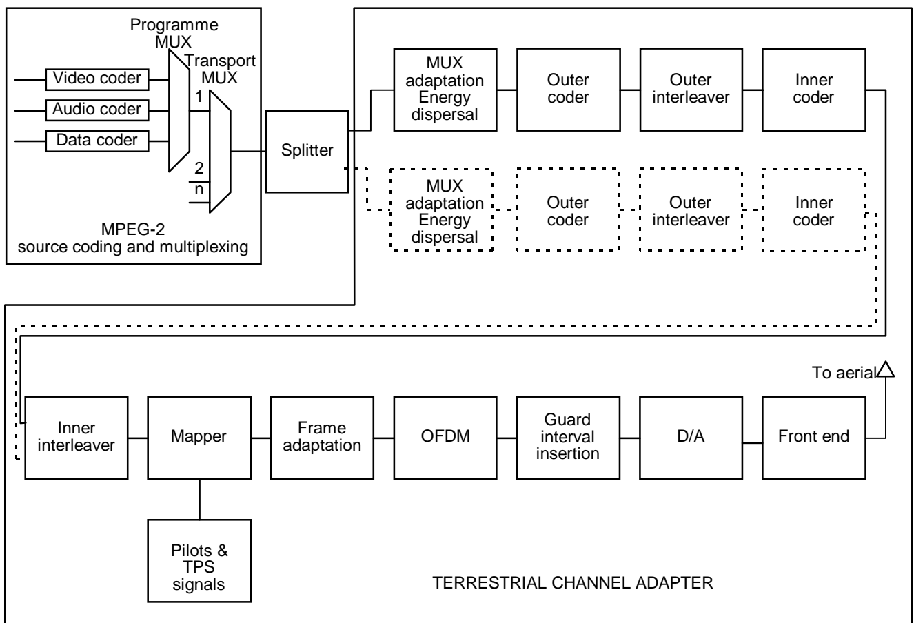
Figure 5: Functional block diagram of the system
