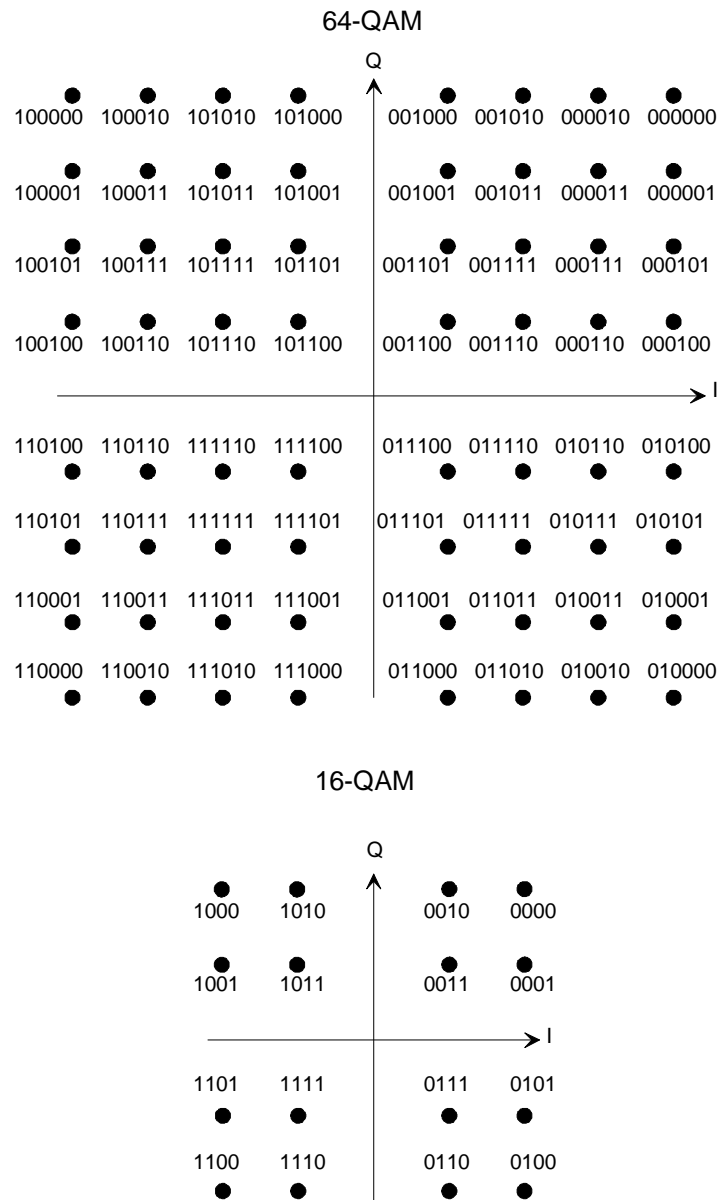
Figure 2: Constellation diagram for the hierarchical modulation ( \alpha=2 )
