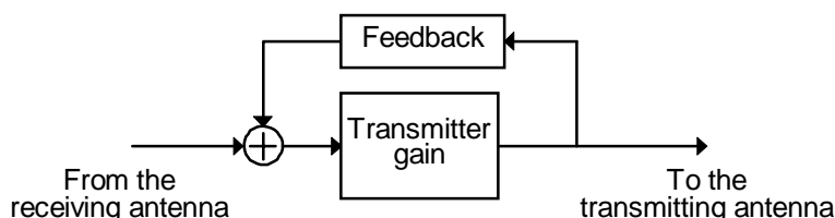
Figure 8: Principle of a re-transmitter
