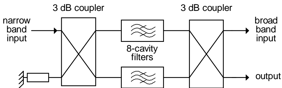
Figure 9: RF DVB-T combiner
