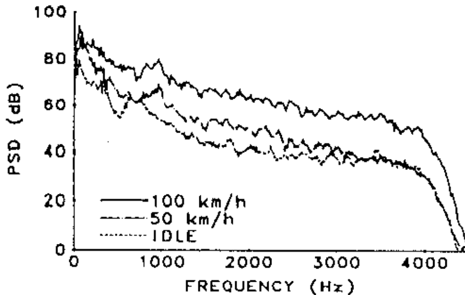
Figure 2: Noise power
