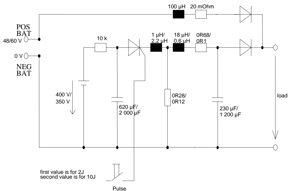
Figure 9: Alternative voltage transient generator for Interface "A"
