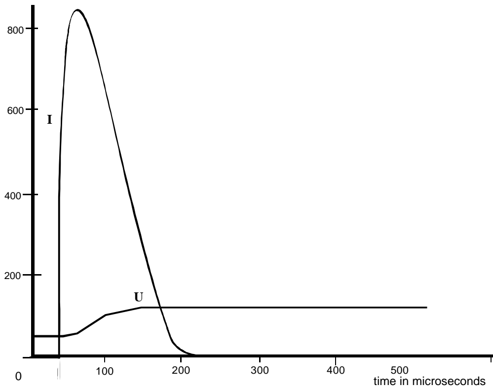
Figure 10: Output voltage and current with 100 Ω / 1 000 μF load (10 J)
