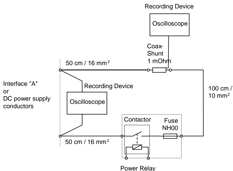
Figure 7: Test set-up for a method for testing high power systems (e.g. more than 1 kW)
