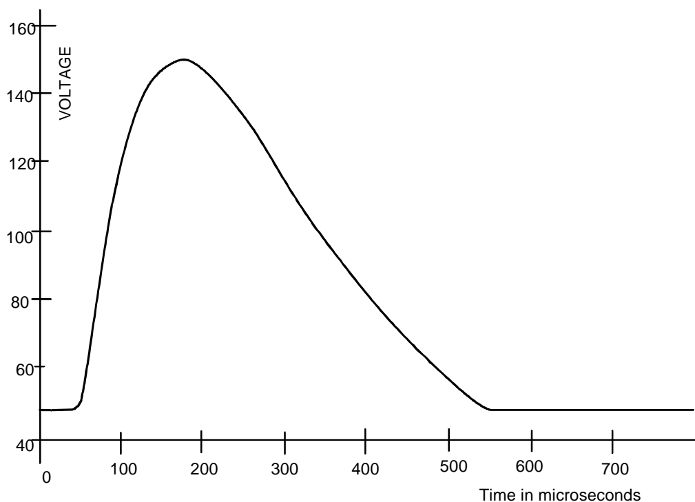
Figure 12: Output voltage with 100 kΩ load (both versions)
