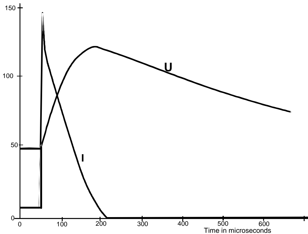
Figure 11: Output voltage and current with 10 Ω / 100 μF load (2 J)
