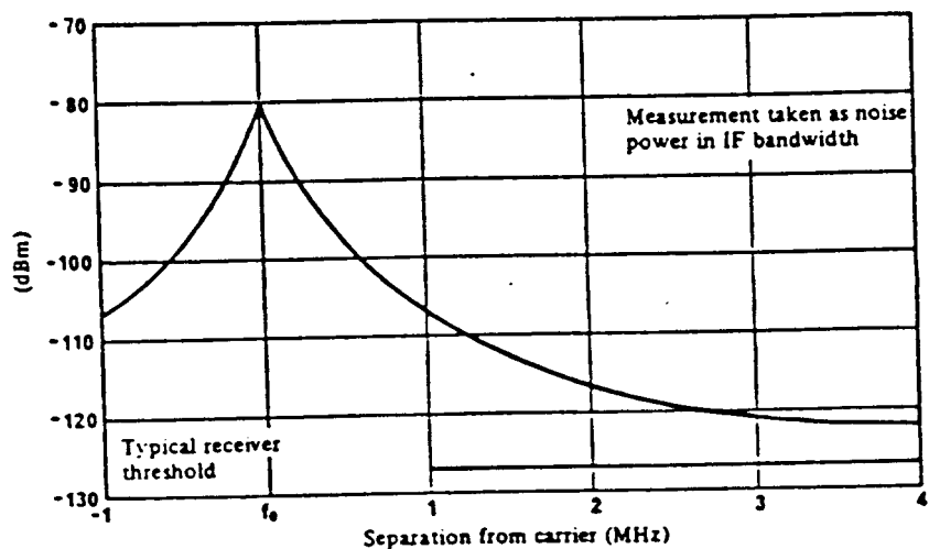
Figure K.2: Typical transmitter noise VHF high band (150 MHz to 170 MHz): solid-state output stage
