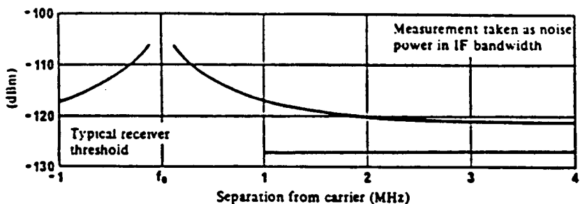
Figure K.3: Typical transmitter noise VHF low band (71,5 - 87,9 MHz): solid-state output stage
