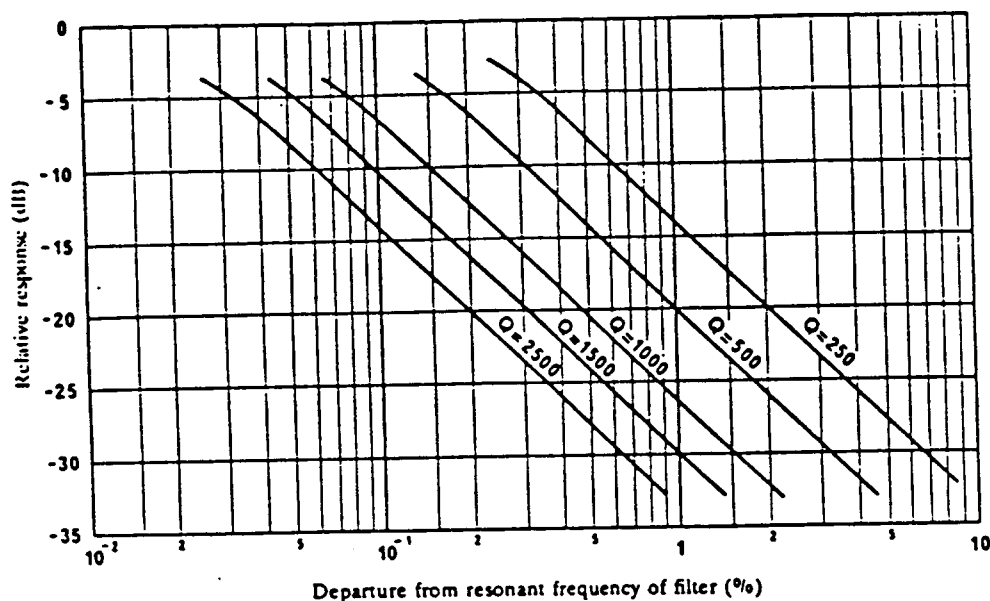
Figure J.3: Theoretical response of cavity band-pass filters
