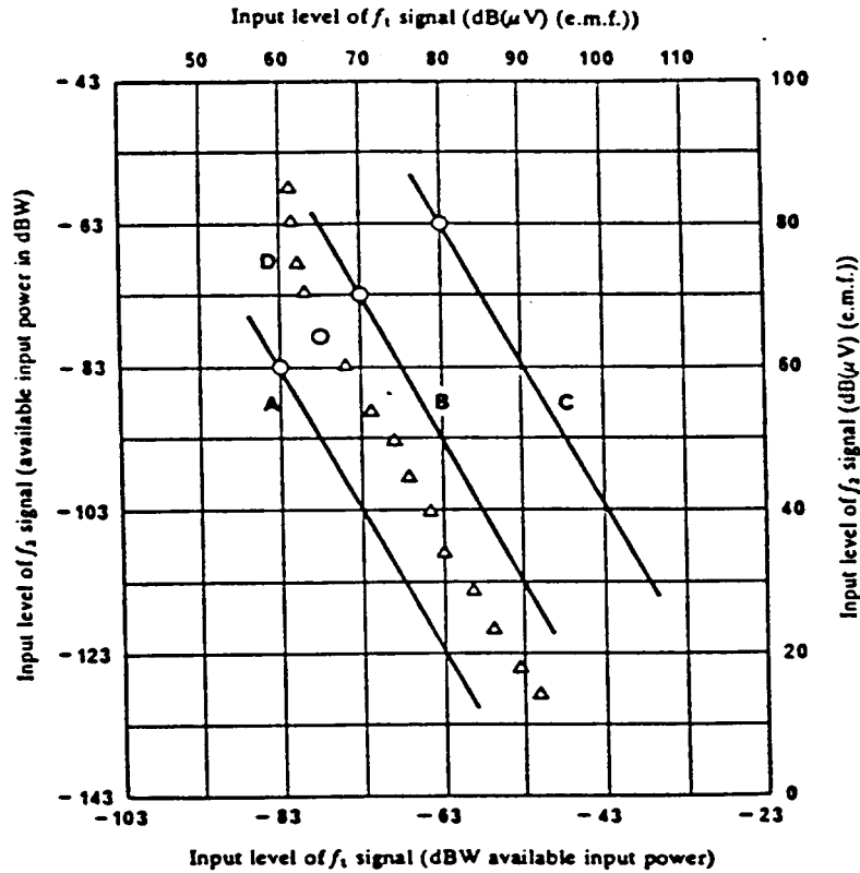
Figure J.2: Receiver intermodulation characteristic
