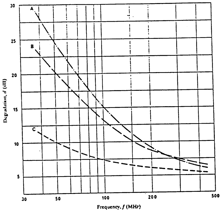
Figure A.4: Variation of degradation of mobile reception and minimum values of field strength to be protected for signal quality grade 3 and receiver sensitivity of 0,7 \mu\text{V} e.m.f.
