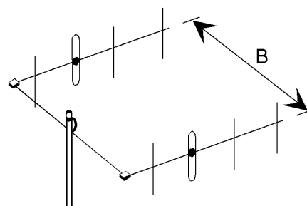
Figure C.10: Vertically polarized (bayed)
