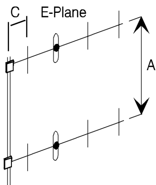
Figure C.7: Vertically polarized (stacked)
