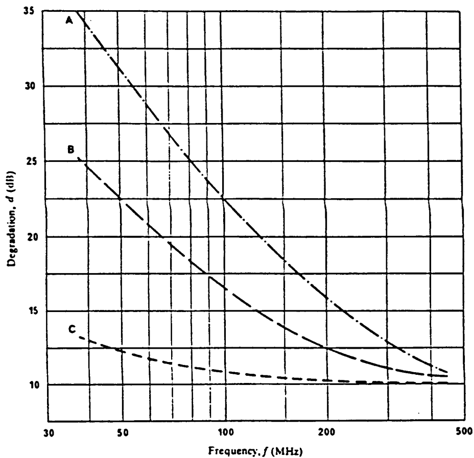
Figure A.3: Variation of degradation of mobile reception and minimum values of field strength to be protected for signal quality grade 4 and receiver sensitivity of 0,7 \mu\text{V} e.m.f.
