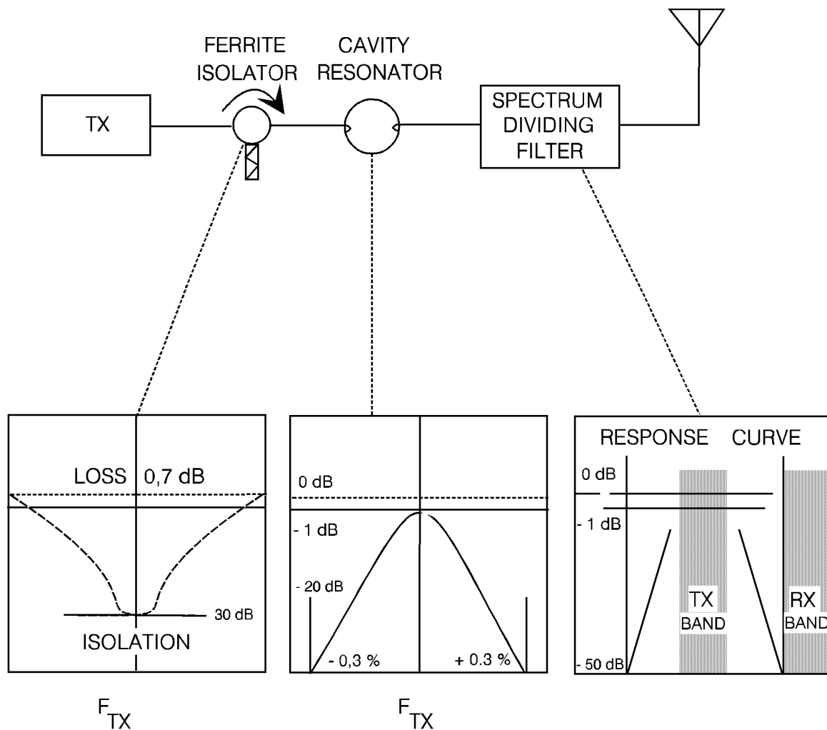
Figure H.19: Typical TX filter system for talkthrough operation (VHF 150 MHz to 160 MHz)
