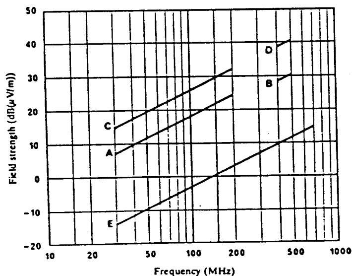
Figure A.2: Minimum useable and medium field strengths for typical hand-portable stations based on minimum useable input of 0,7 \mu\text{V} e.m.f., in the absence of man-made noise
