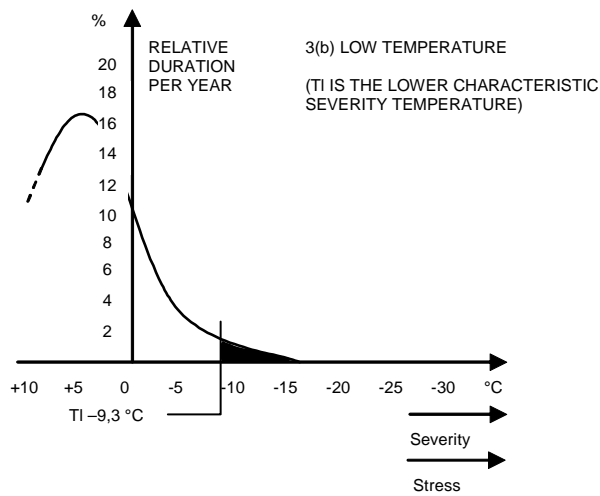
Figure 3: Separated distributions of outdoor air temperature showing the boundary value of the upper (Tu) and the lower (TI) characteristic temperature
