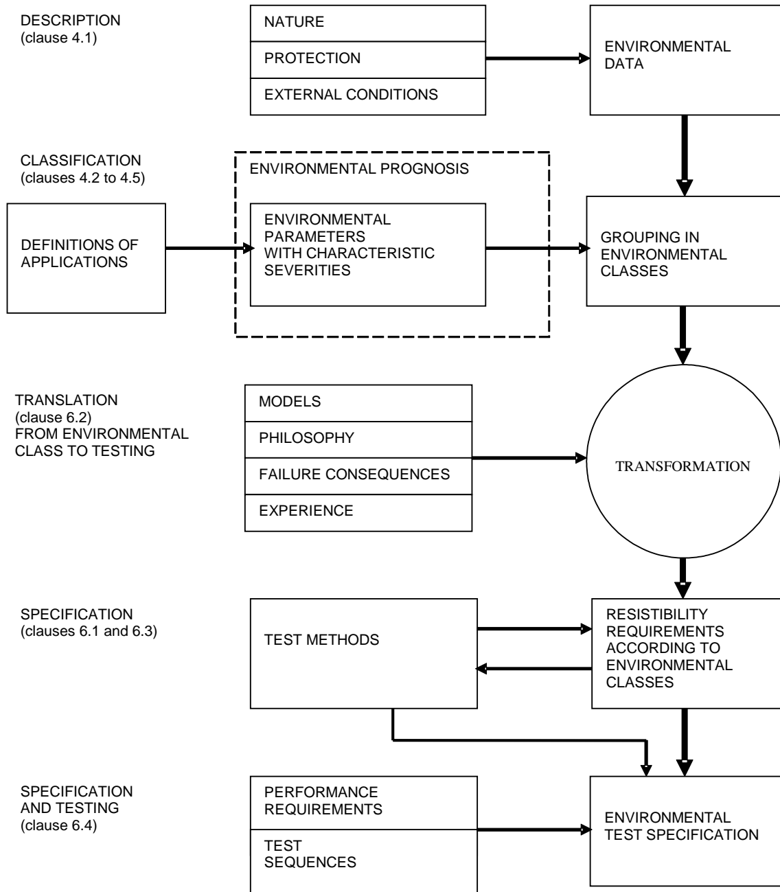
Figure 1: Outline for the preparation of the test specification
