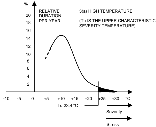
Figure 2: Distribution of outdoor temperature
