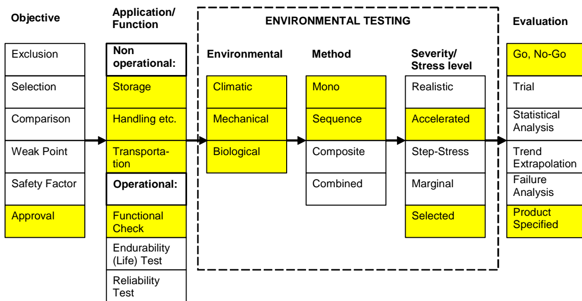
Figure 5: Outline of environmental testing applications
