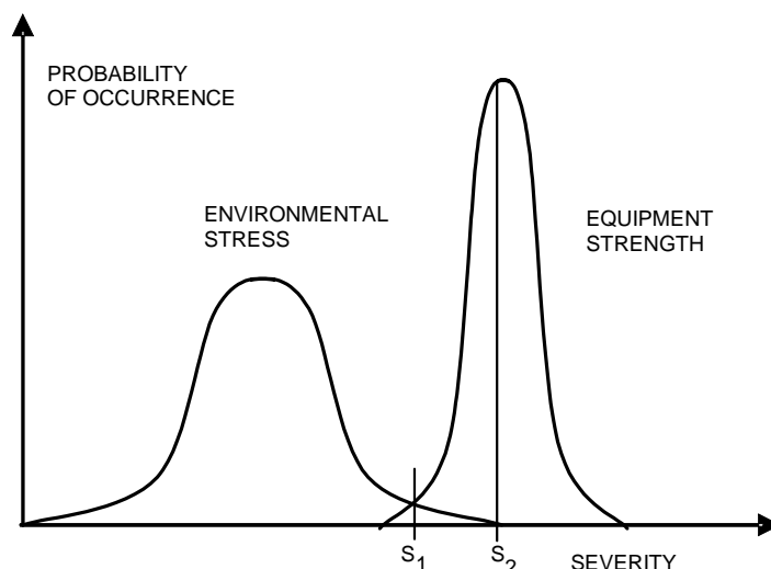
Figure 7: Stress-strength curves for an equipment with a lower strength limit which is too low
