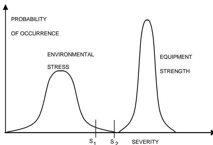
Figure 6: Stress-strength curves for an equipment with a reasonable safety margin
