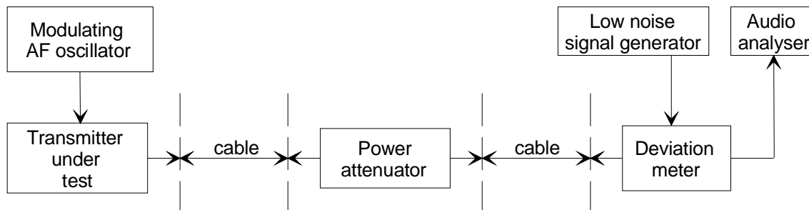
Figure 54: Measurement configuration for modulation frequencies above 3 kHz
