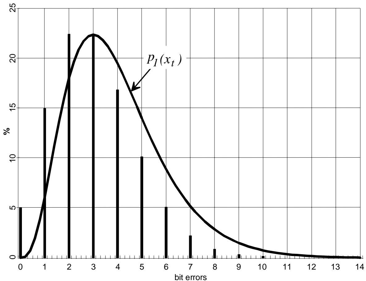
Figure 17: BER uncertainty
