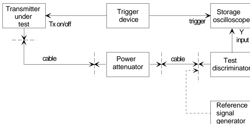
Figure 52a: Transmitter frequency/time measurement configuration (attack and release)
