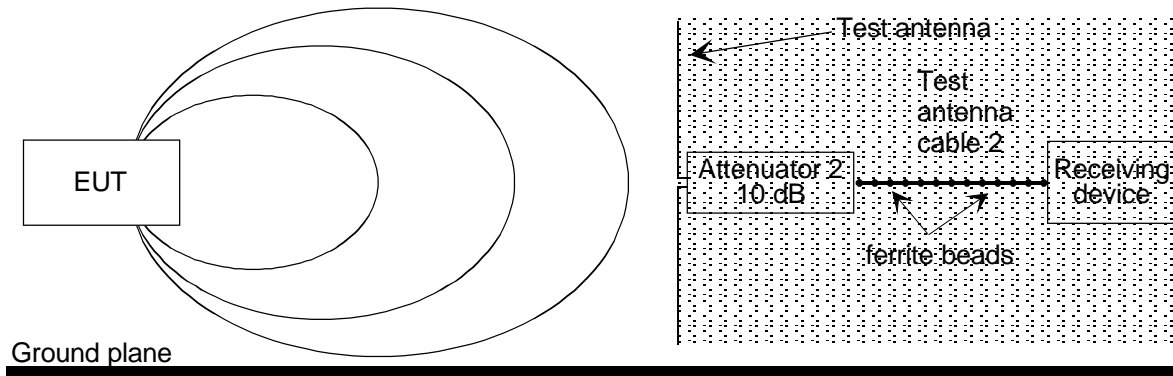
Figure 57: Stage one: EUT measurement
