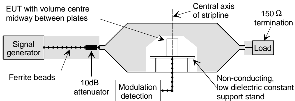
Figure 37: Stage 1: EUT measurement
