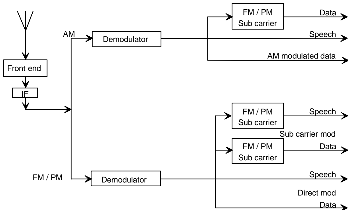
Figure 13: Possible receiver configurations
