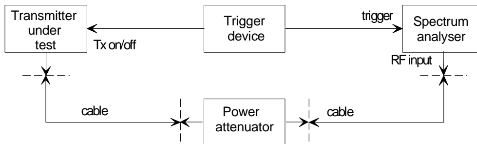
Figure 52b: Transmitter power level/time measurement configuration (attack and release)
