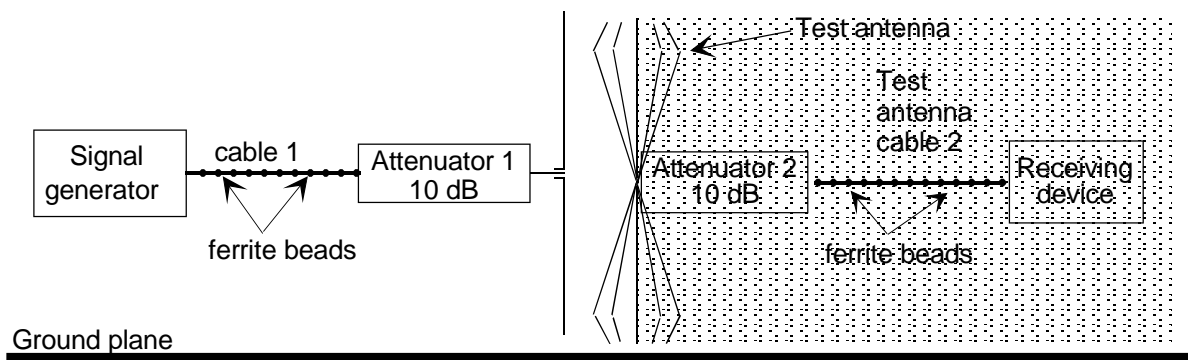
Figure 64: Stage two: Substitution measurement
