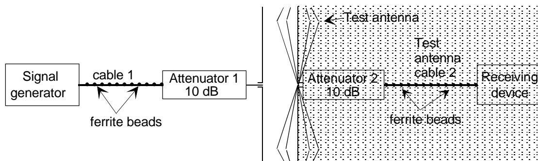
Figure 62: Stage two: Substitution measurement
