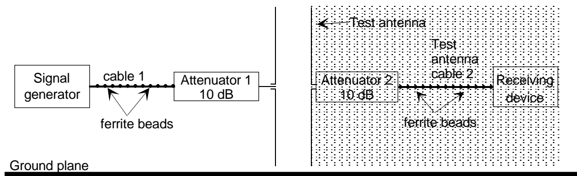
Figure 60: Stage two: Substitution
