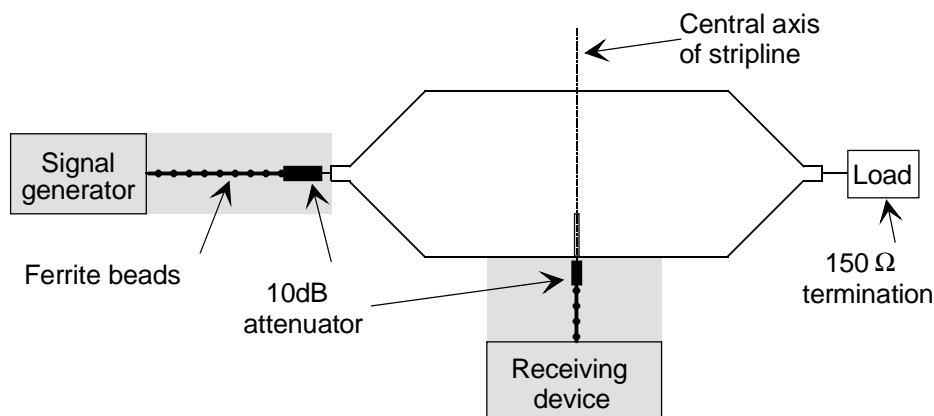
Figure 35: Stage 2: Radiated attenuation measurement
