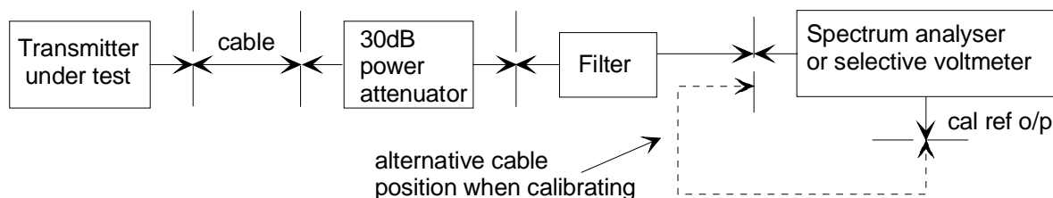
Figure 48a: Conducted spurious emission measurement configuration (direct method)
