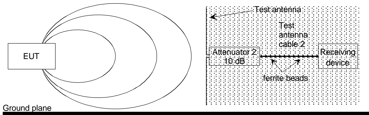
Figure 59: Stage one: EUT measurement
