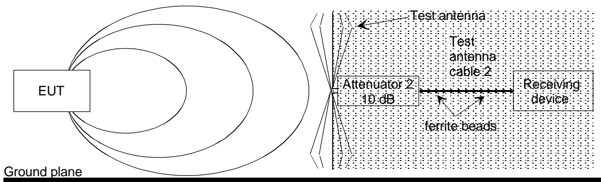
Figure 65: Stage one: EUT measurement
