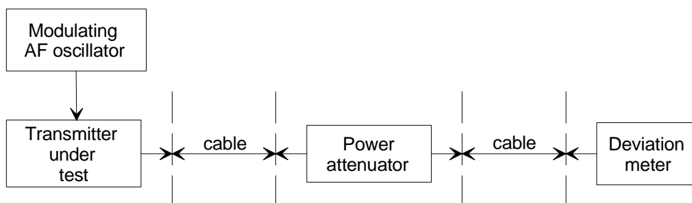
Figure 53: Maximum permissible frequency deviation measurement configuration
