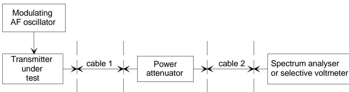
Figure 46: Measurement configuration for adjacent channel power (method 2)
