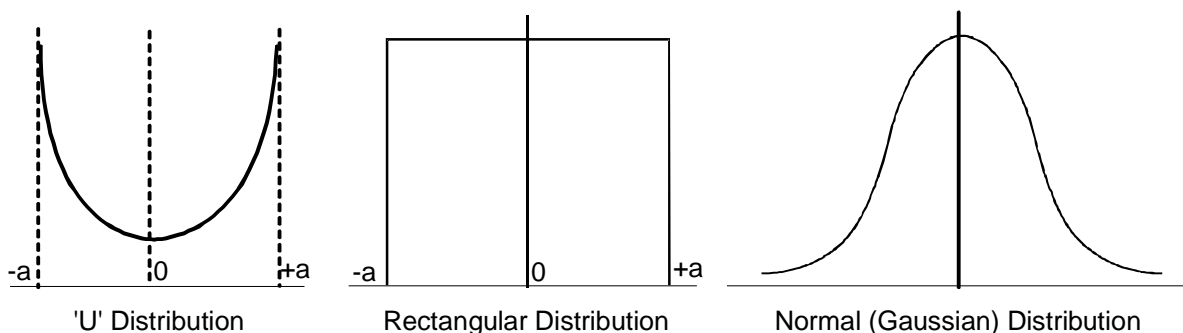
Figure 5: Types of uncertainty distribution
