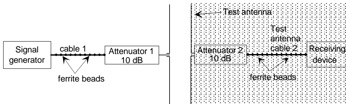
Figure 56: Stage two: Substitution measurement
