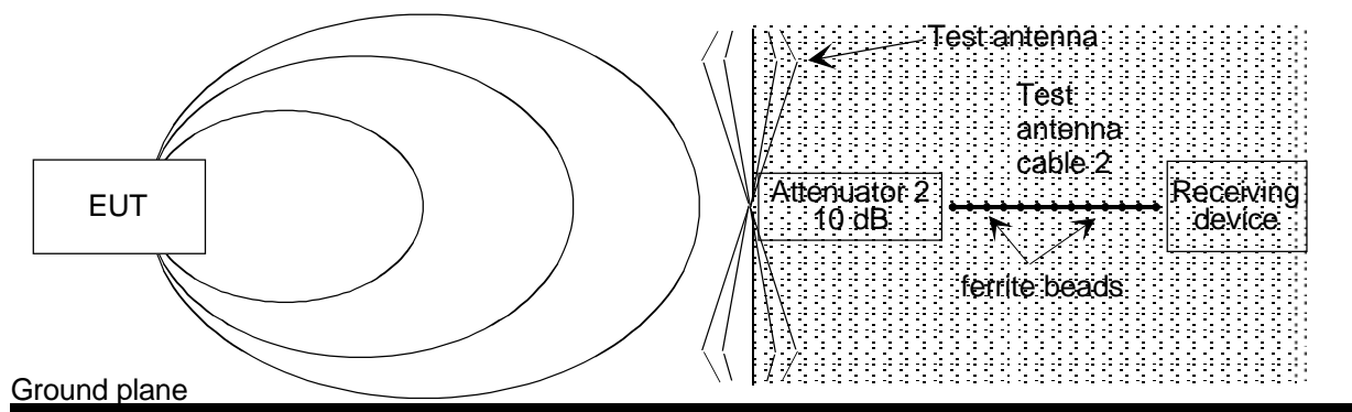
Figure 63: Stage one: EUT measurement
