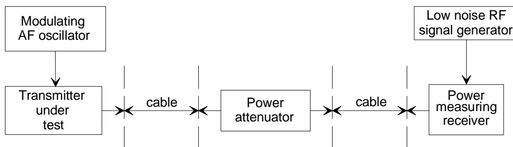
Figure 45: Measurement configuration for adjacent channel power measurement (method 1)
