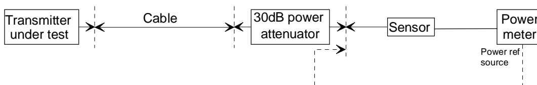
Figure 44a: Carrier Power measurement configuration
