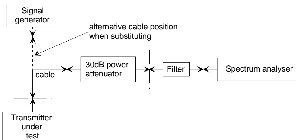
Figure 48b: Conducted spurious emissions measurement configuration (substitution method)
