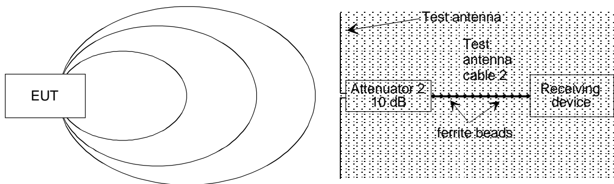
Figure 55: Stage one: EUT measurement
