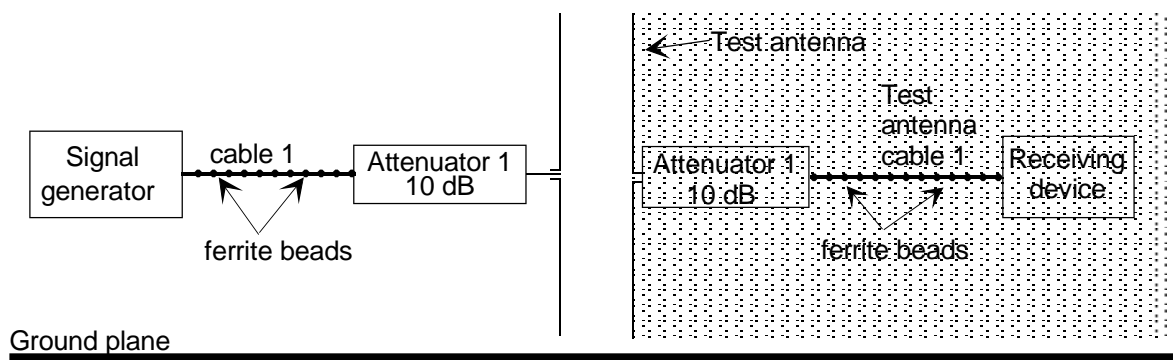
Figure 58: Stage two: Substitution measurement
