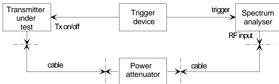
Figure 51: Transmitter power level/time measurement configuration (attack and release)
