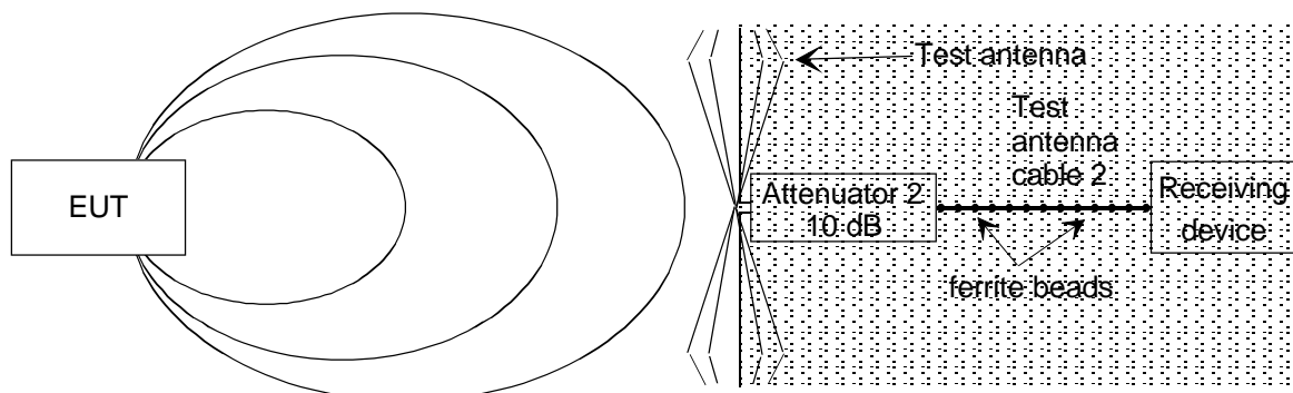
Figure 61: Stage one: EUT measurement
