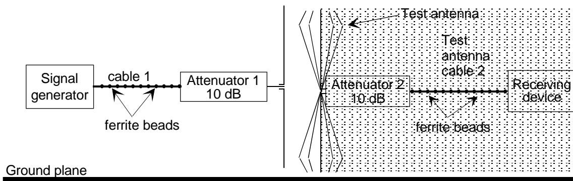
Figure 66: Stage two: Typical emission substitution test
