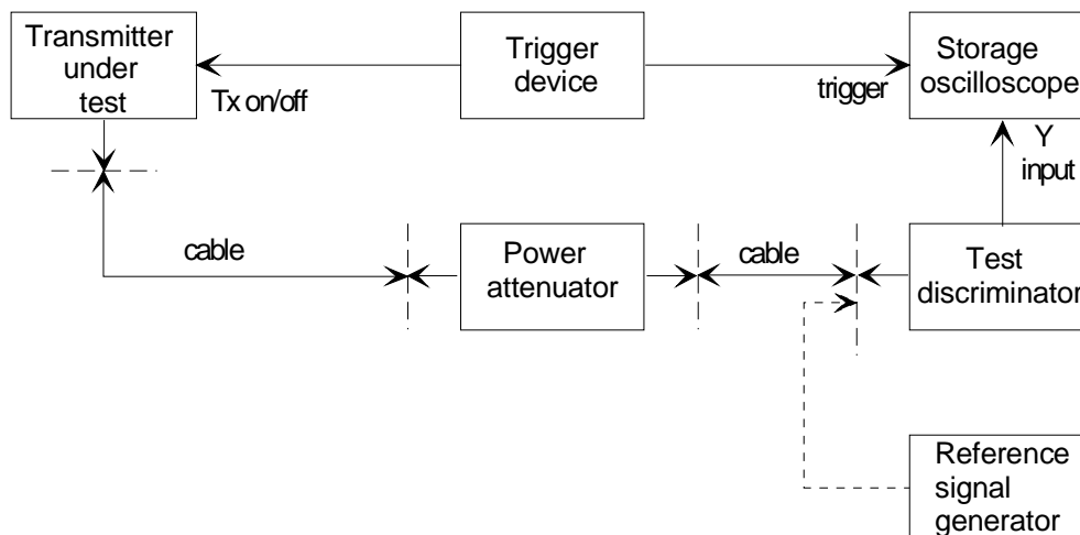
Figure 50: Transmitter frequency/time measurement configuration (attack and release)
