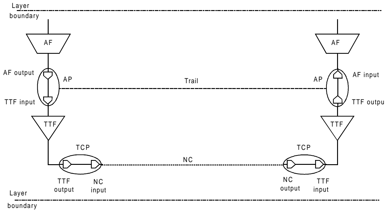
Figure 2: End transport entities/functions
