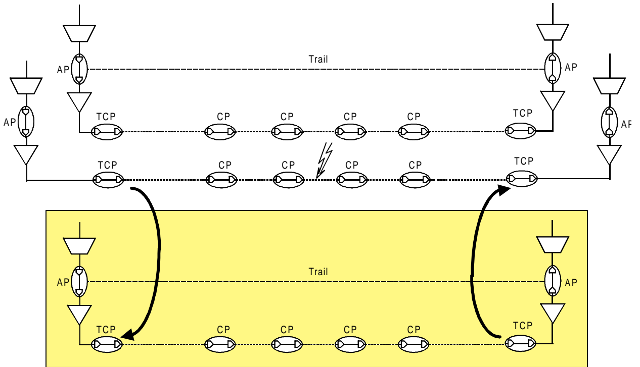
Figure 9: 1:2 protection
