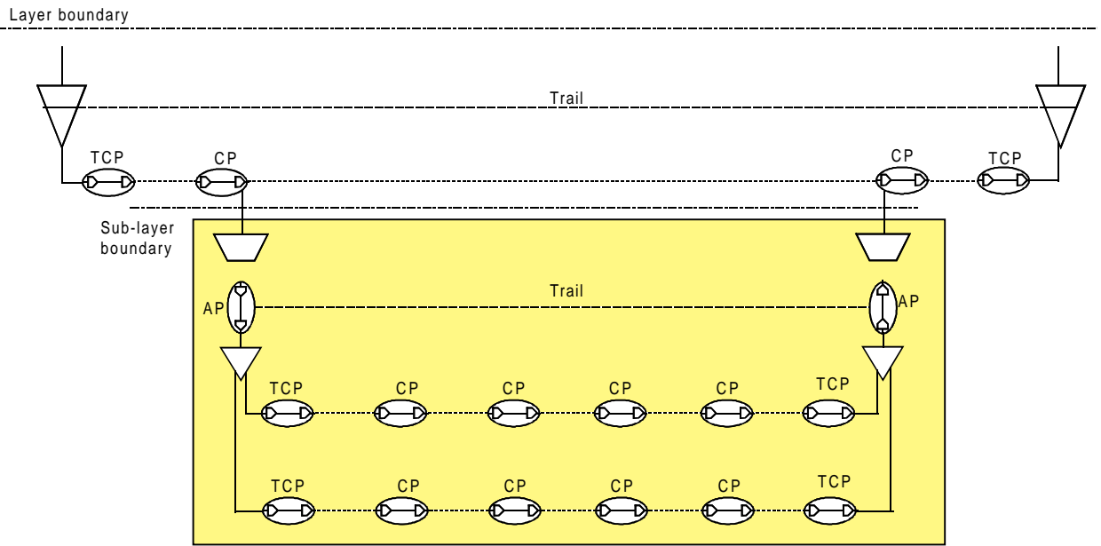
Figure 8: VP/VC sub-network connection 1+1 protection
