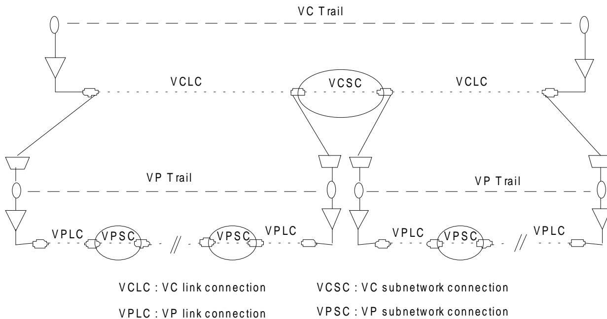
Figure 3a: A given VC trail configuration
