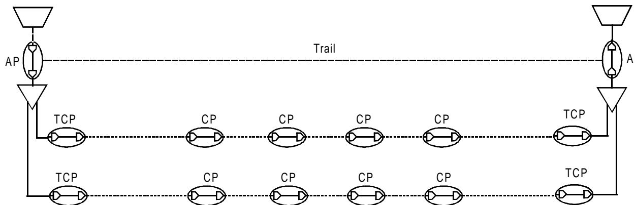
Figure 7: VPNC/VCNC 1+1 protection
