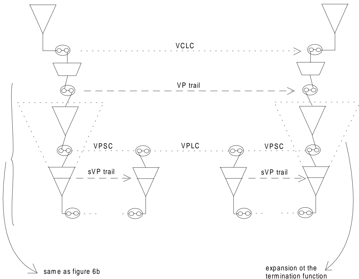
Figure 6c: Sublayering for VP tandem connection monitoring
