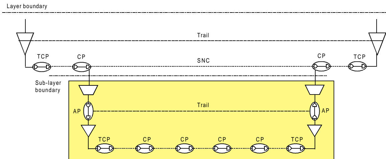
Figure 5: Sub-network monitoring
