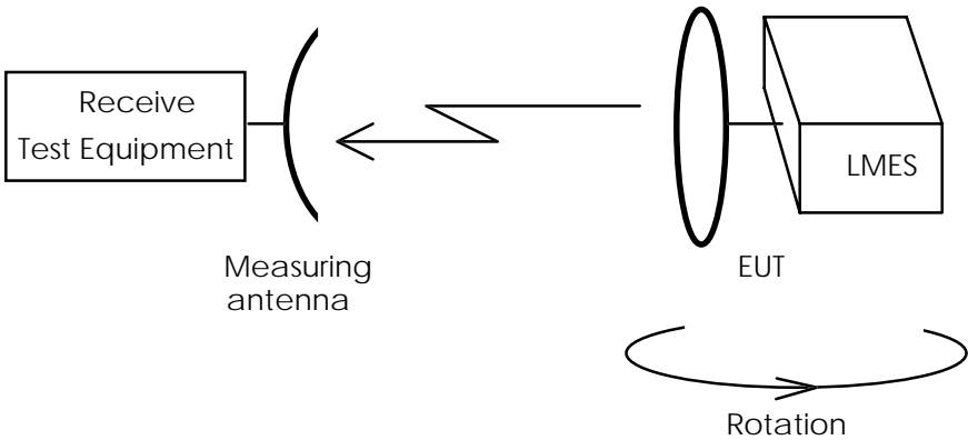
Figure 1: Test arrangement - emissions measurement, first axis
