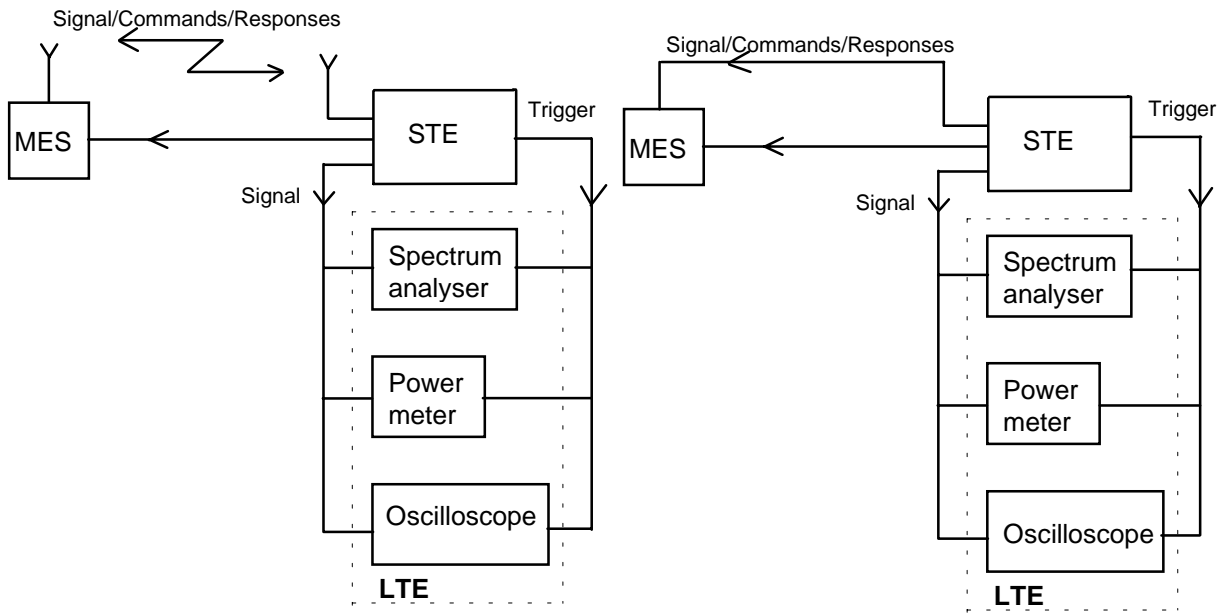
Radiated test
