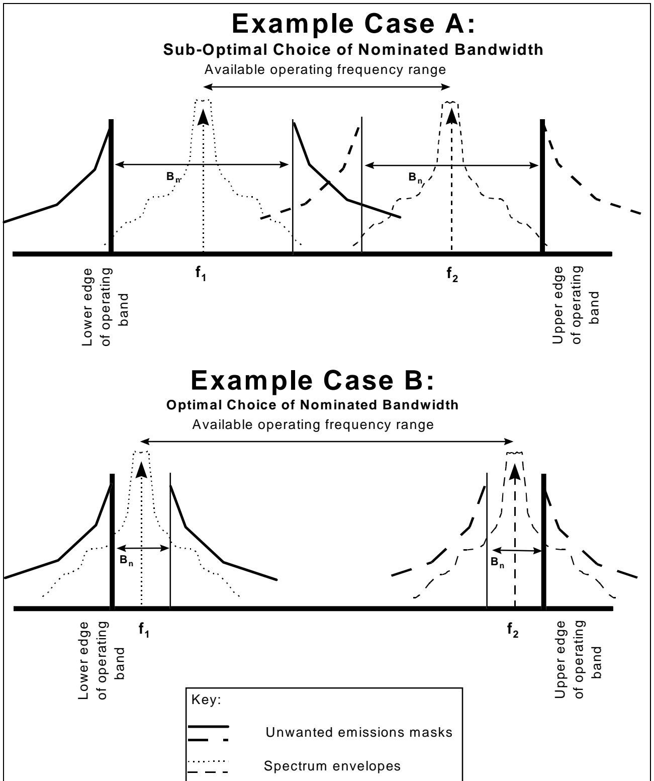
Figure E.2: Choice of nominated bandwidth
