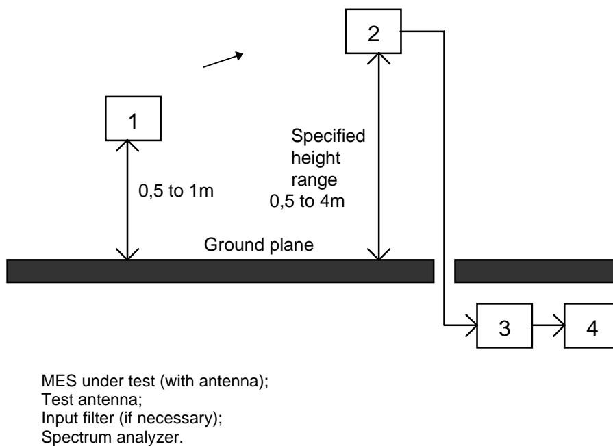
Figure C.1: Measurement arrangement No. 1
