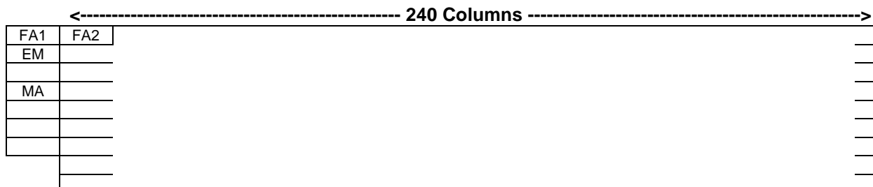
Figure C.1: Frame structure at 139 264 kbit/s
