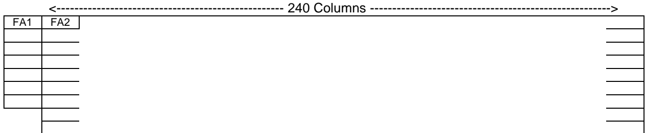
Figure C.1: Frame structure at 139 264 kbit/s
