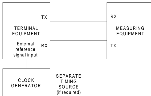
Figure A.3: Output timing
