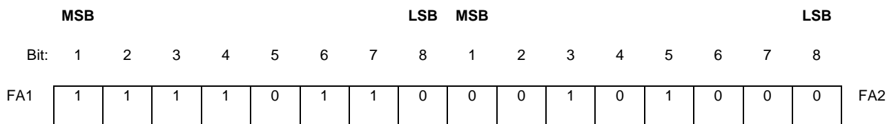
Figure C.1: Frame structure at 34 368 kbit/s
