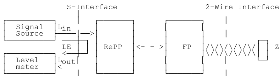
Figure 11: FP with analogue 2-wire interface
