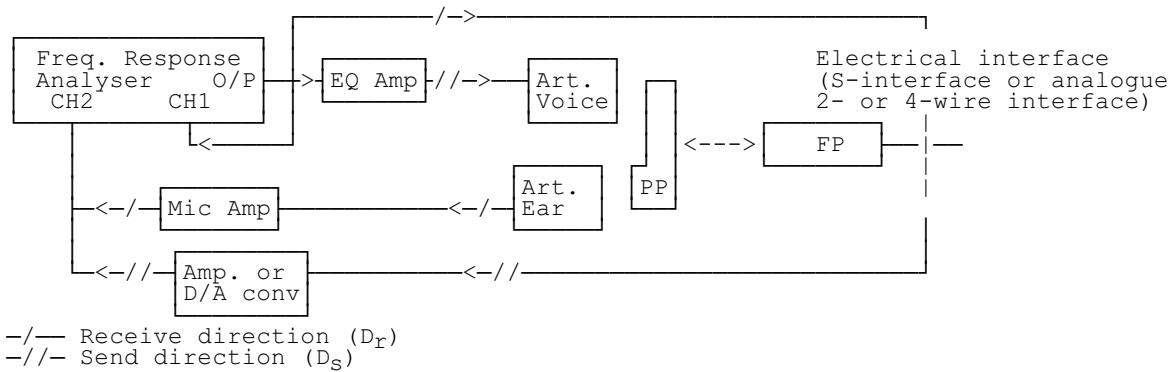
Figure 7: DECT network delay test configuration
