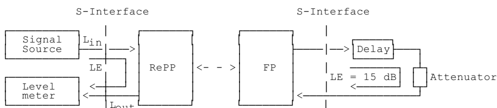
Figure 10: FP with 4-wire interface
