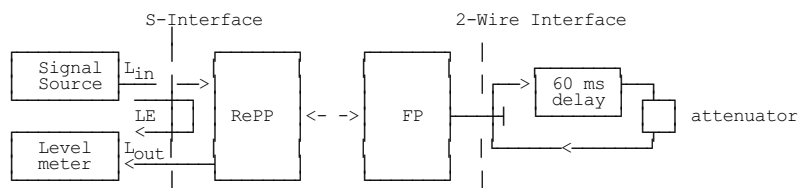
Figure 12: FP with analogue 2-wire interface
