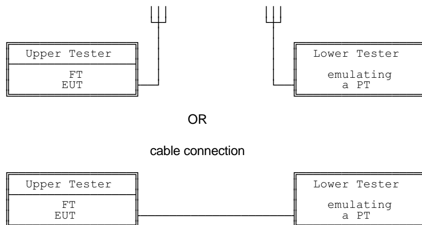
Figure 2: The EUT is a FT
