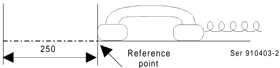
Figure A.2: Handset position for stability loss test
