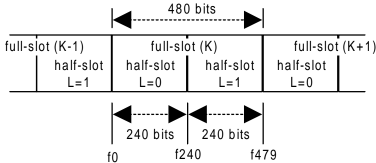
Figure 25: Half-slot format
