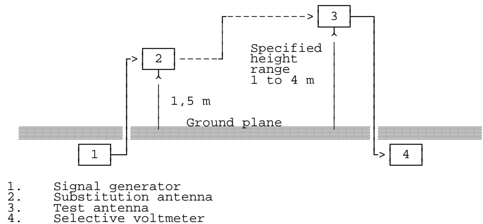
Figure 3: Measuring arrangement for calibration
