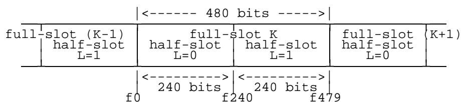
Figure 25: Half-slot format
