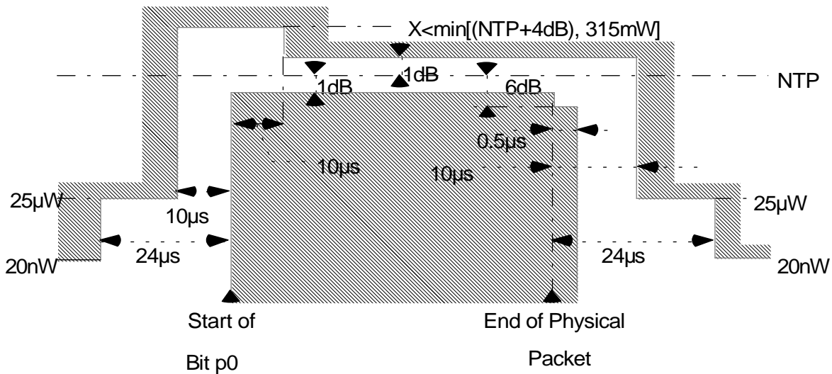
Figure 29: Power-time template
