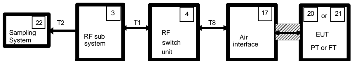
Figure 10: Test set-up 1
