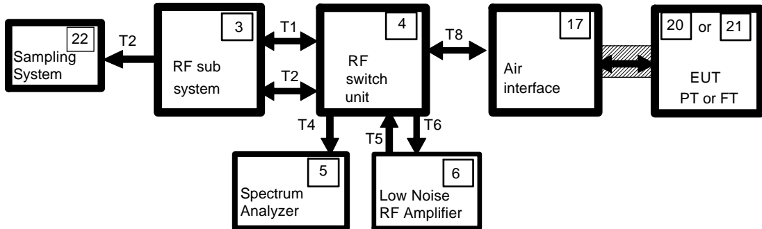
Figure 13: Test set-up 4
