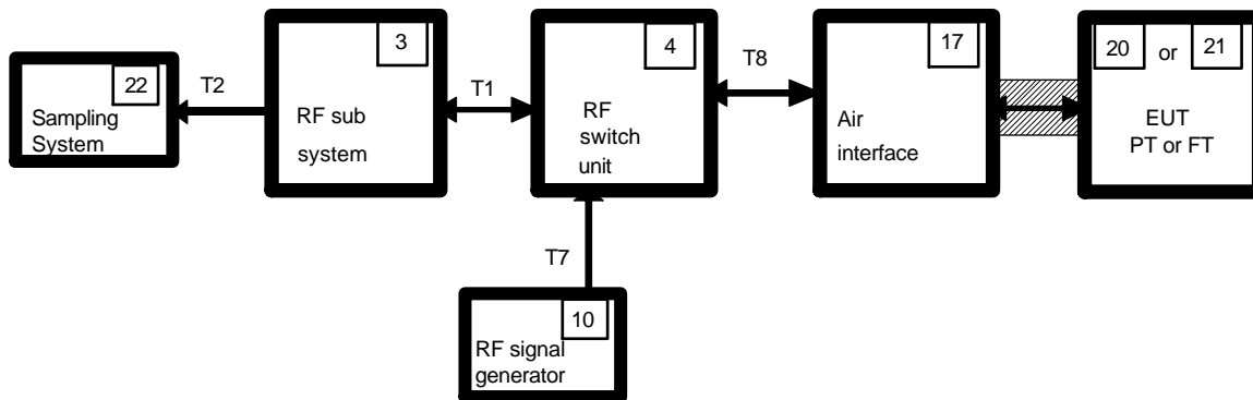
Figure 11: Test set-up 2
