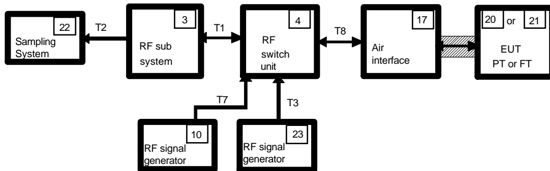
Figure 12: Test set-up 3
