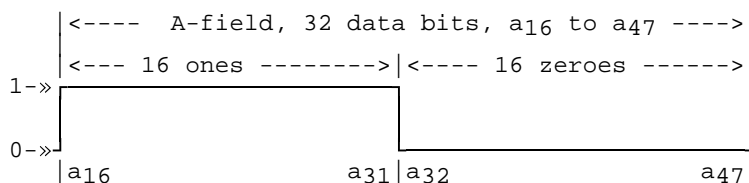
Figure 30: Test packet structure for Case 2, A-field
