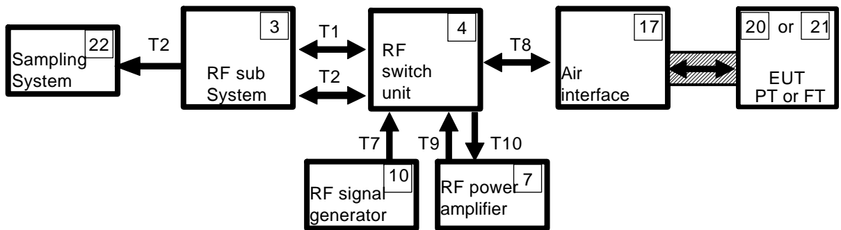
Figure 14: Test set-up 5
