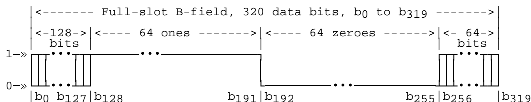
Figure 31: Test packet structure for case 2, half-slot
