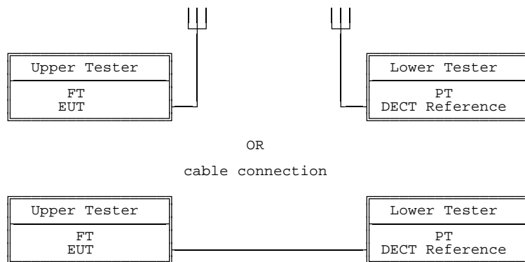
Figure 2: The EUT as an FT
