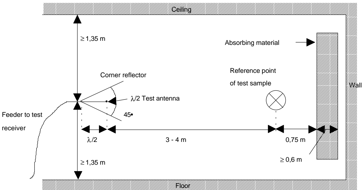
Figure 8: Indoor test site arrangement (shown for horizontal position)
