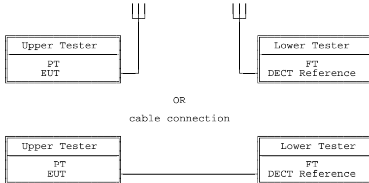
Figure 1: The EUT as a PT
