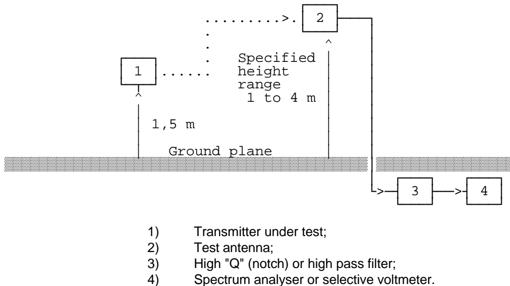
Figure B.3: Measurement arrangement N°1
