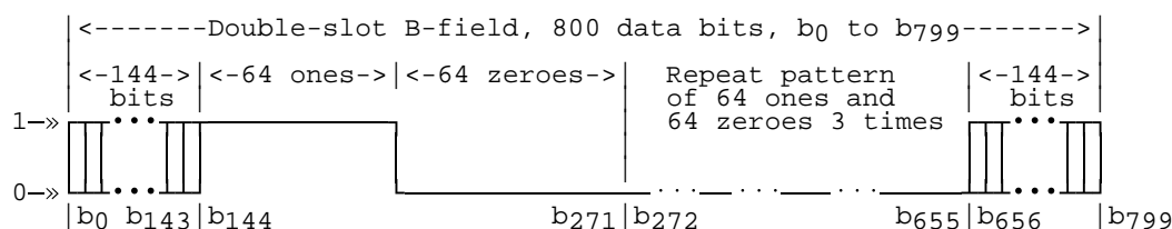
Figure 32: Test packet transmission for case 2, full-slot
