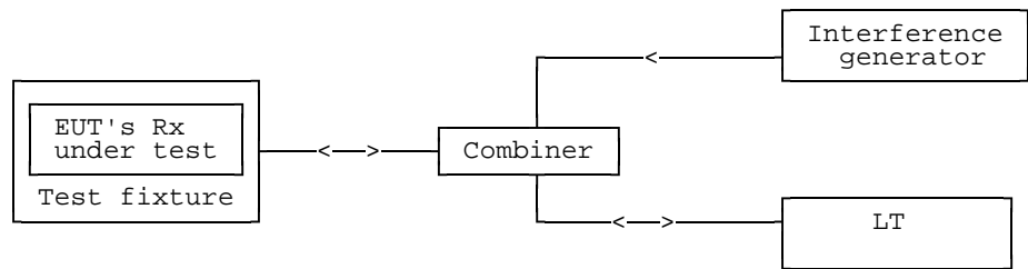
Figure 7: Measuring arrangement for calibration
