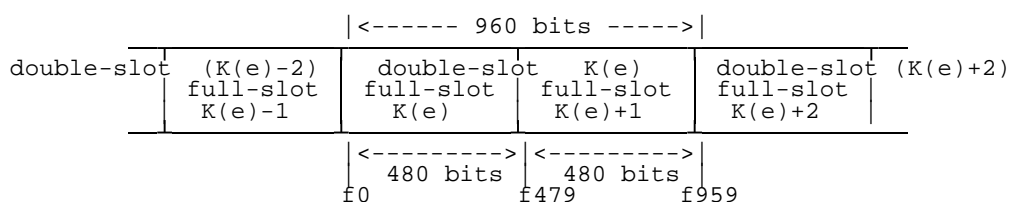
Figure 26: high_slotDouble-slot format
