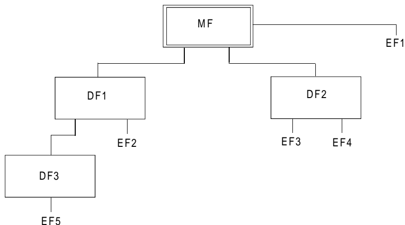
Figure 7: Logical structure
