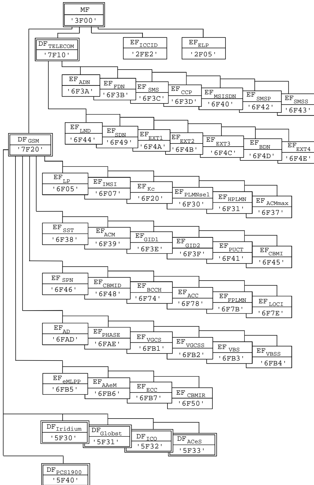
Figure 8: File identifiers and directory structures of GSM
