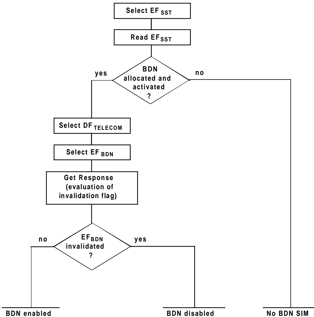
BDN capability request (see subclause 11.5.1)
