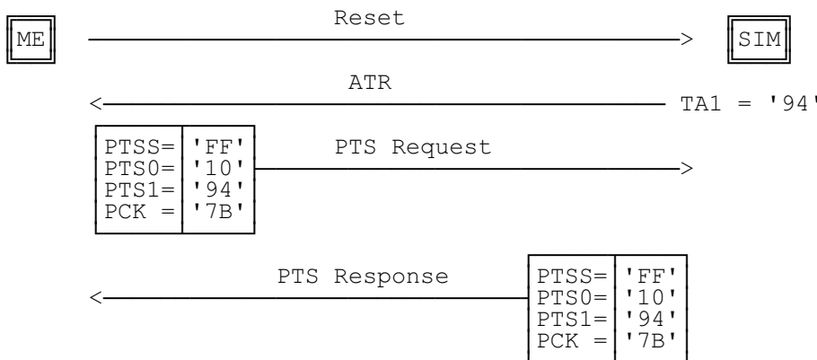
Figure 2: PTS procedure requesting enhanced speed values (F=512, D=8, see subclause 5.8.3)
