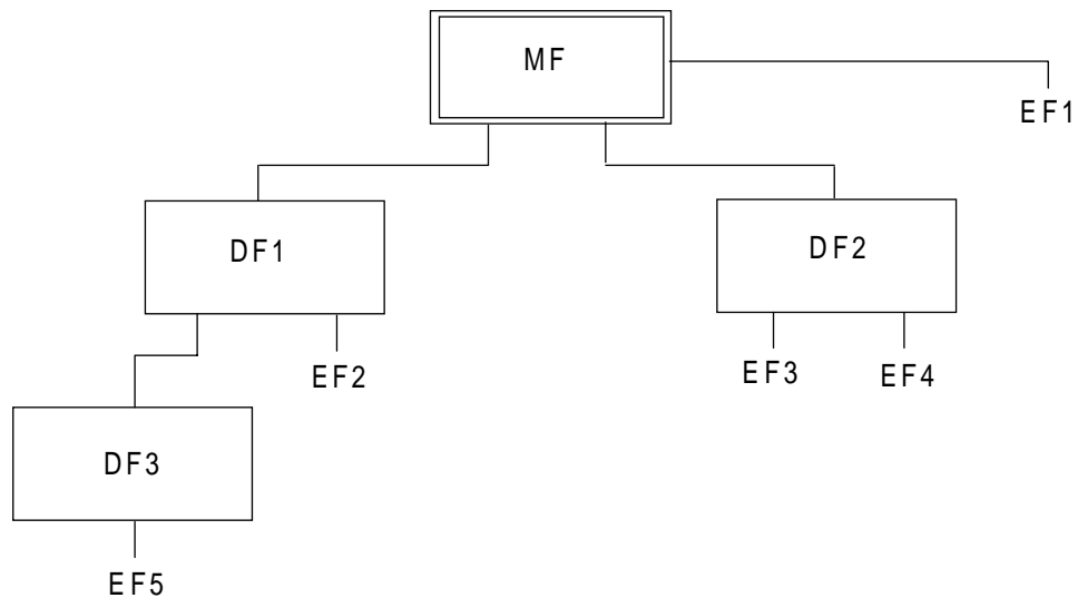
Figure 7: Logical structure
