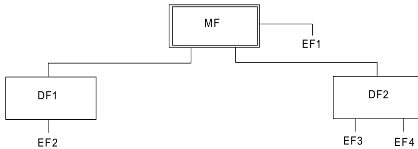
Figure 7: Logical structure
