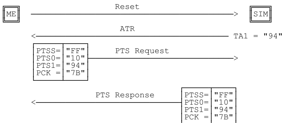
Figure 2: PTS procedure requesting enhanced speed values (F=512, D=8, see clause 5.8.3)
